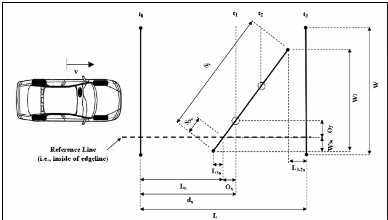
Figure 24. Z-Configuration Layout.
