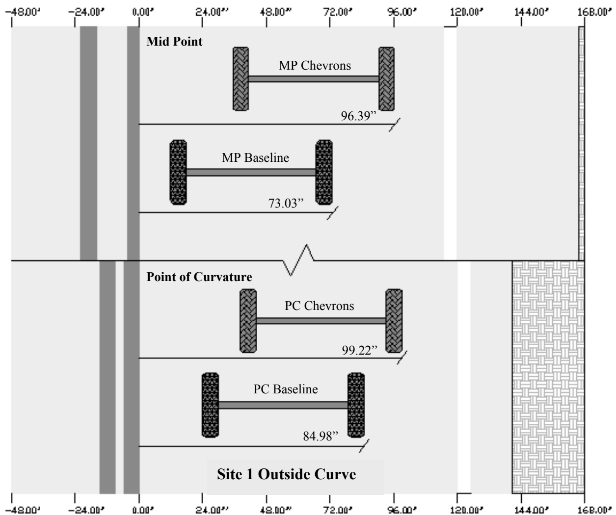
Figure 28. Baseline and Chevron Lateral Position Diagram
