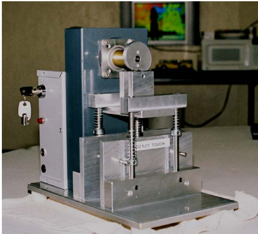
Figure 3.11 Final Prototype Loading Device
