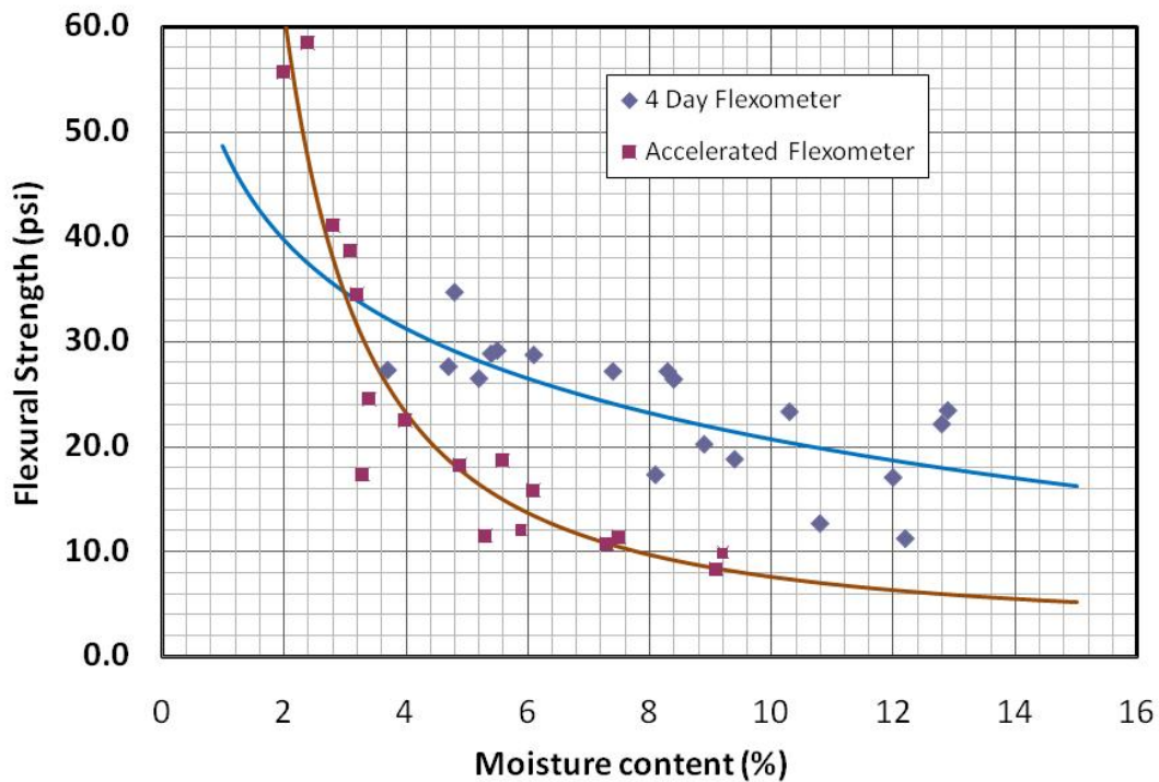
Figure 5.11 Comparison of Data Obtained from Standard, 4-Day Flexometer and Accelerated Flexometer Tests; Waco-Frost Source
