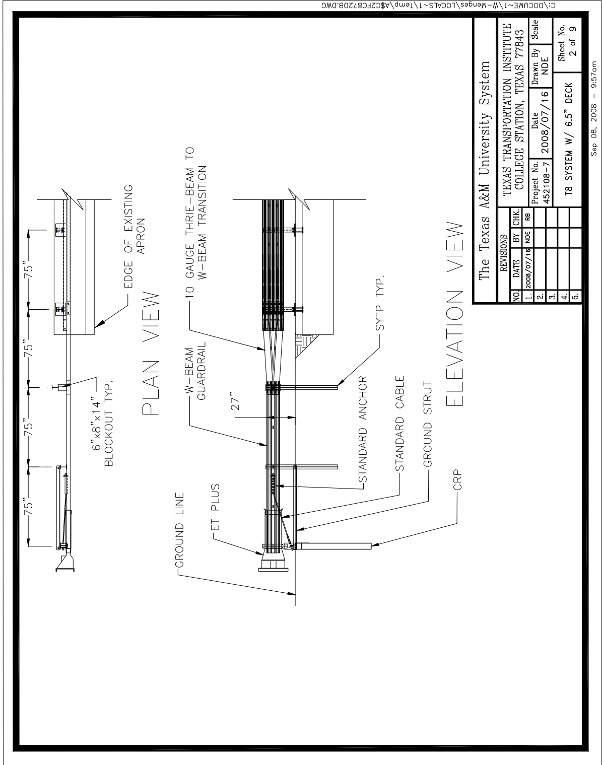
Figure 2.2. Details of the T8 Bridge Rail Installation – Terminal Details.
