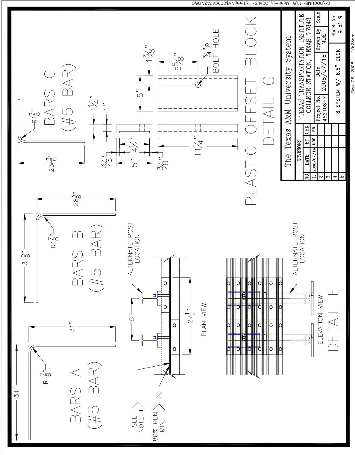
Figure 2.9. Details of the T8 Bridge Rail Installation – Miscellaneous Details.
