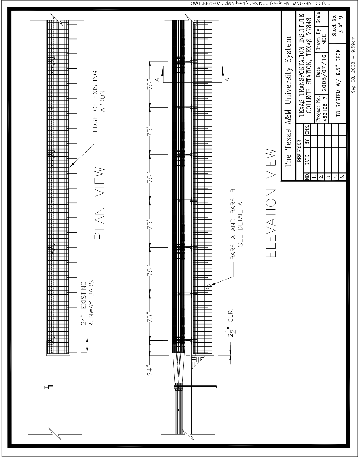
Figure 2.3. Details of the T8 Bridge Rail Installation – Rebar Detail.
