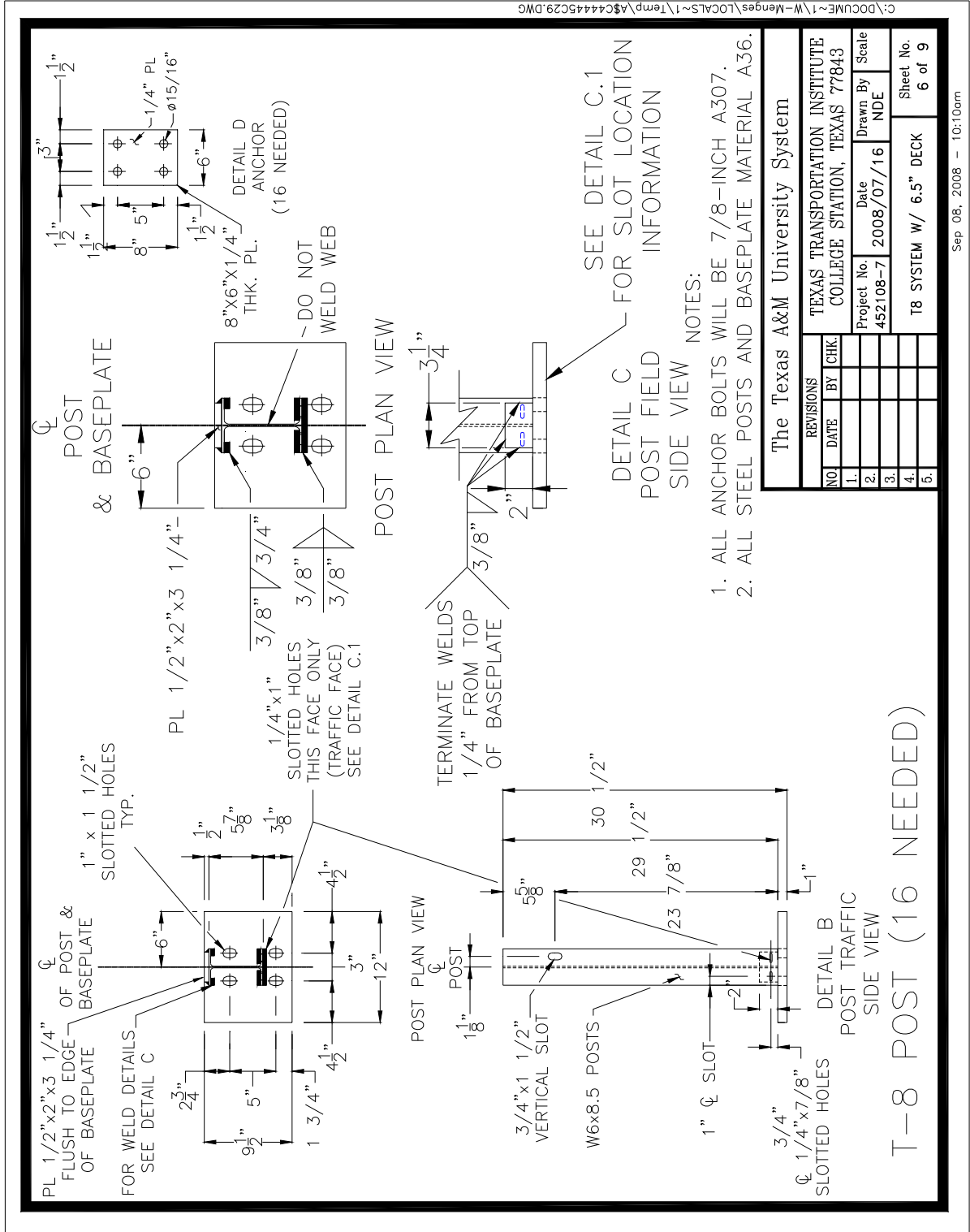
Figure 2.6. Details of the T8 Bridge Rail Installation – Post Details.
