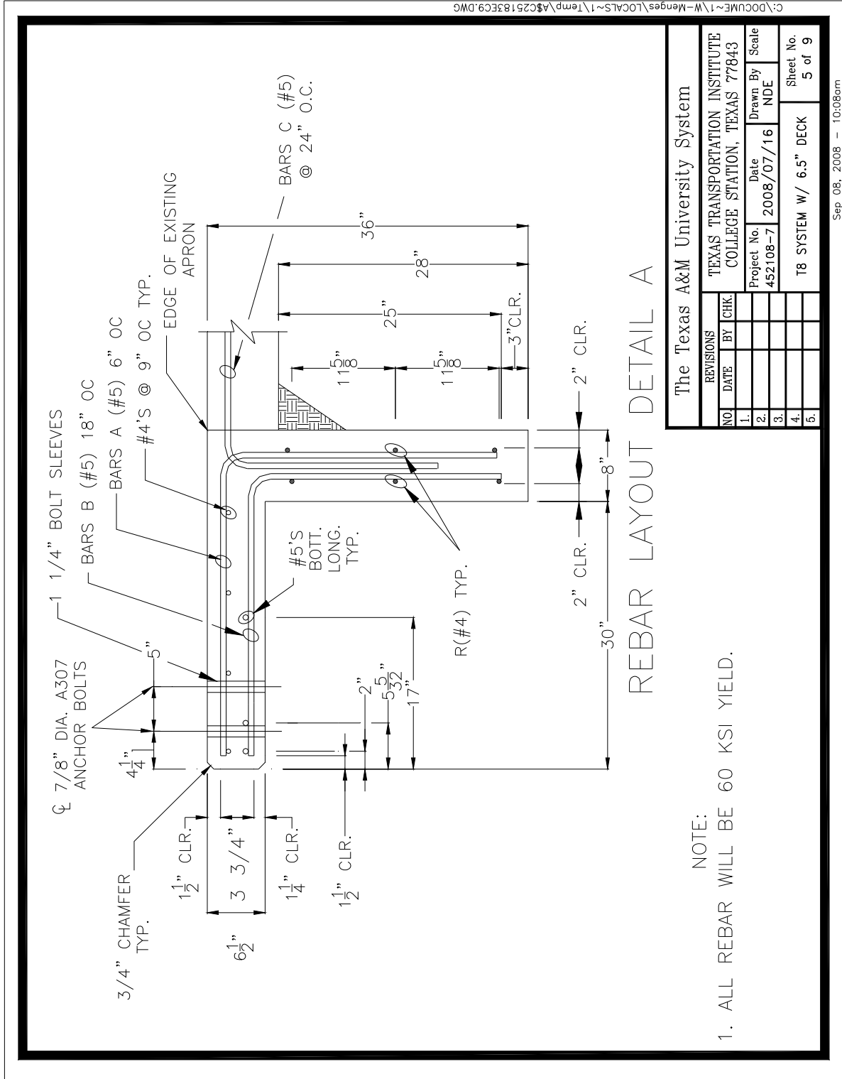
Figure 2.5. Details of the T8 Bridge Rail Installation – Rebar Layout.
