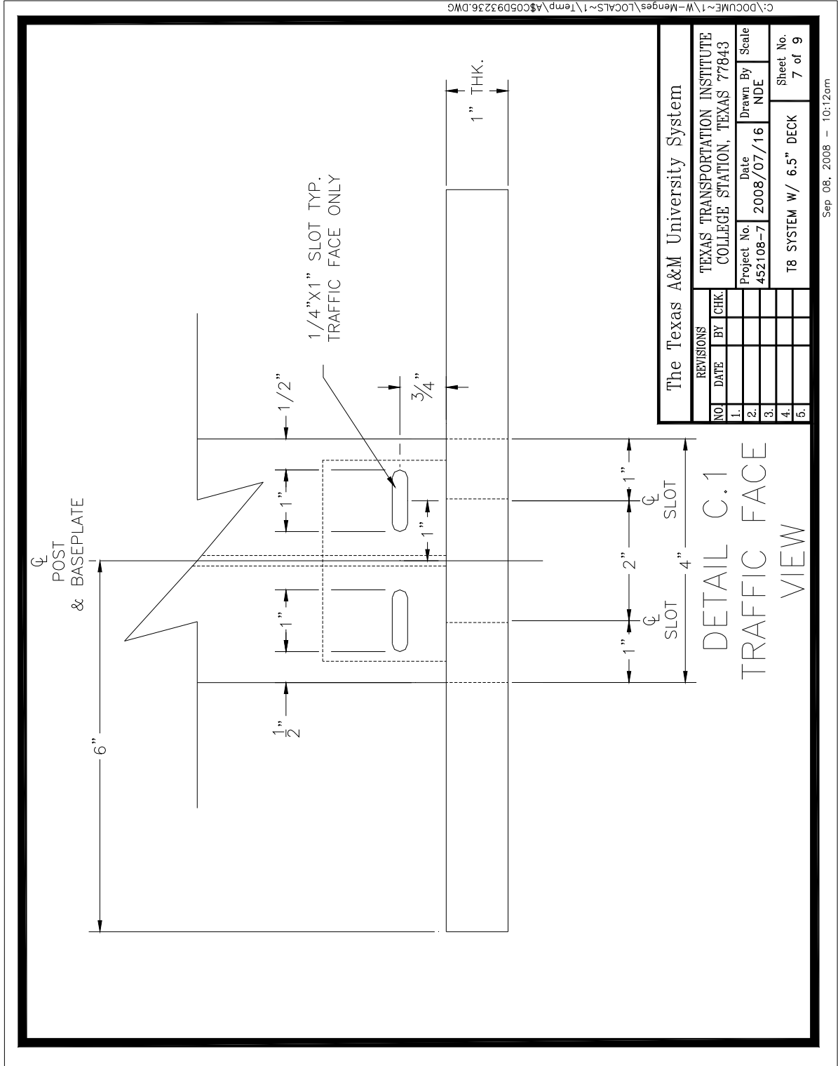
Figure 2.7. Details of the T8 Bridge Rail Installation – Slot Details.
