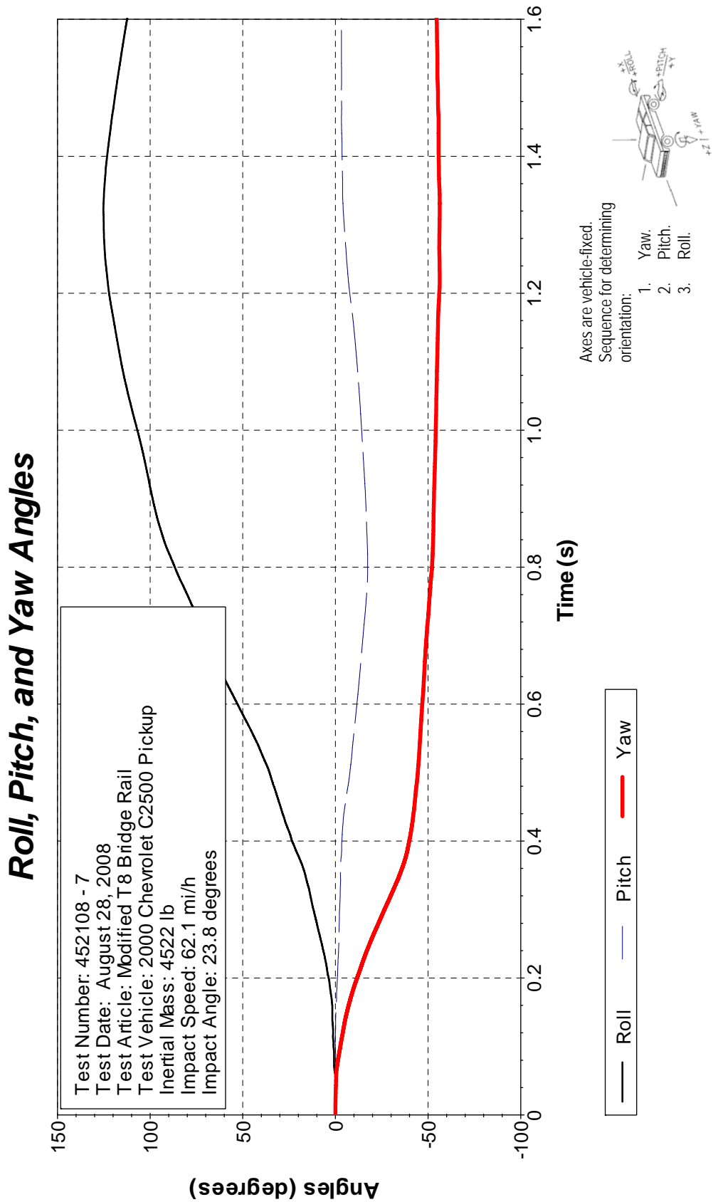
Figure D1. Vehicle Angular Displacements for Test 452108-7.
