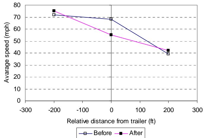
Figure 4. Condition-Responsive Speed Display and Its Effect on Average Speed. 13
