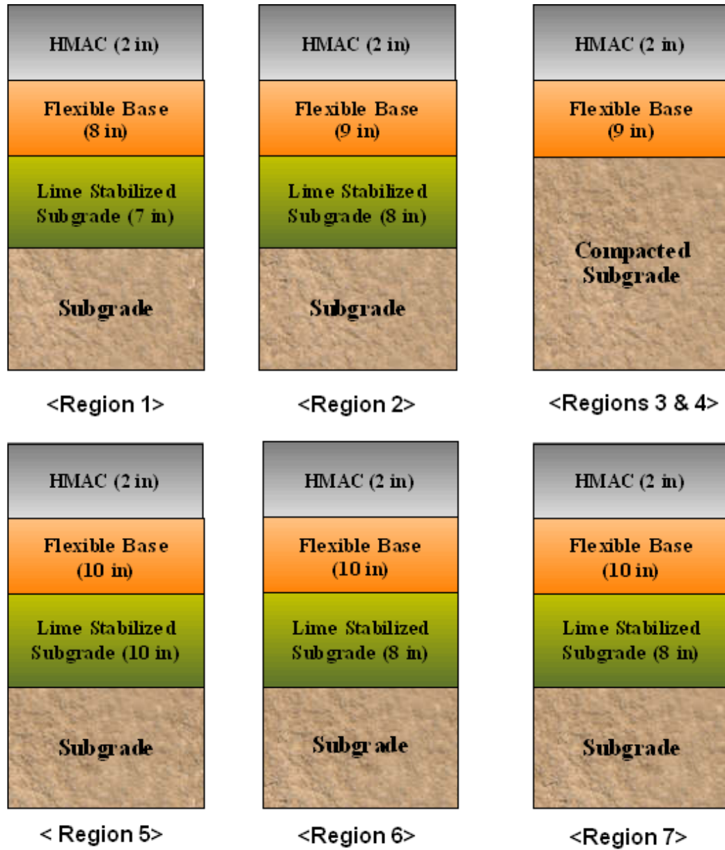
Figure 4.1. Typical Pavement Structures for FM Roads in Different Climatic Regions.
