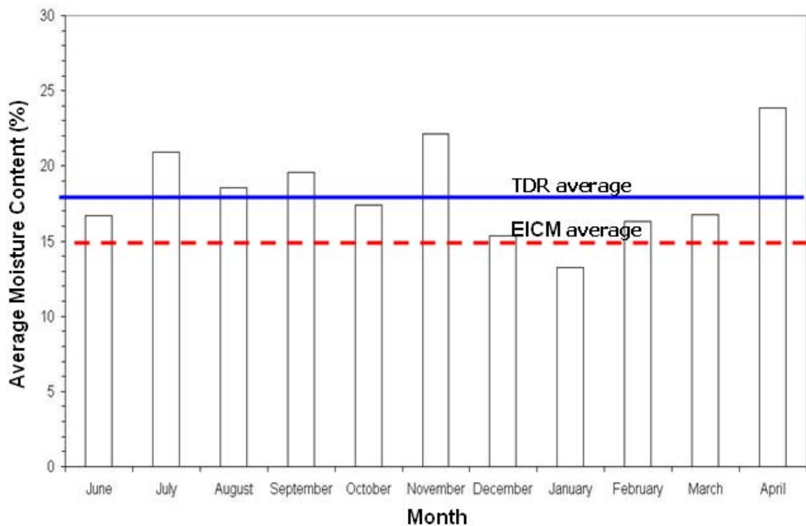
Figure 4.5. Comparison of EICM Predictions with TDR Measurements from Base Layer of Flexible Pavement Test Section in Brownsville.
