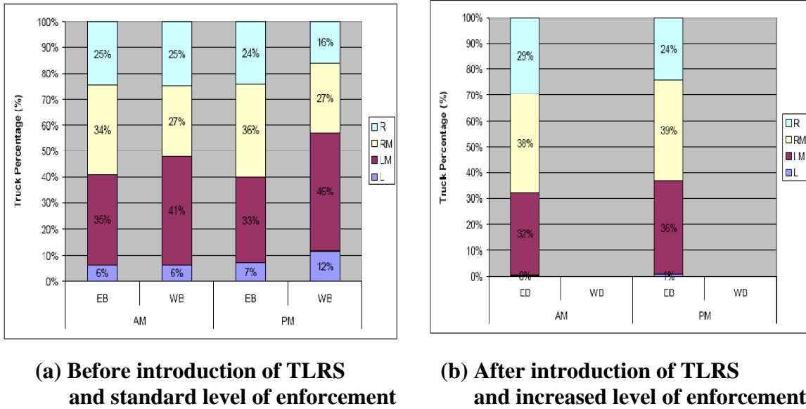
Figure 7 Impact of TLRS and enforcement on lane distributions of trucks on I-20 (Sims and Royester, 2006)
