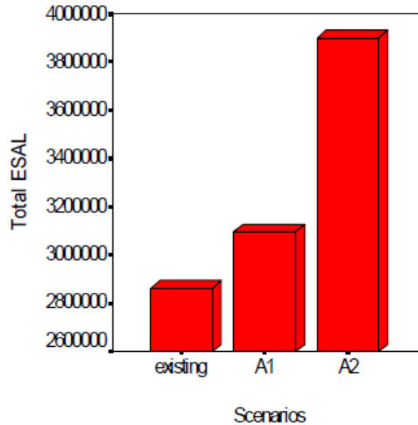
Figure 9 Impact of TLRs on pavement damage (Yang and Regan, 2007)
