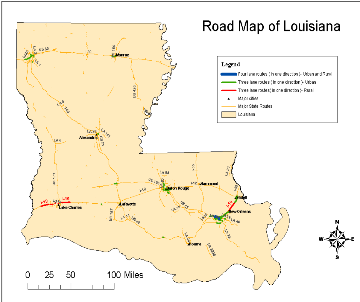
Figure 10 Routes in Louisiana with more than two lanes in each direction (Note: Only red sections represent candidate sites for TLRS implementation and all require thorough analysis before implementation)
