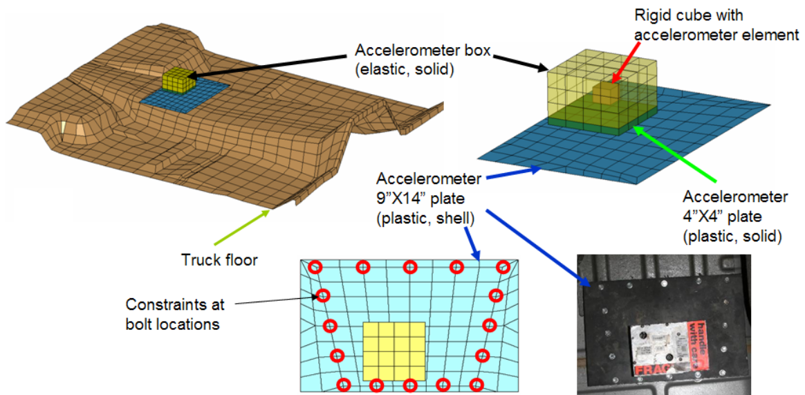
Figure 2.10. Explicit Accelerometer Assembly Model.
