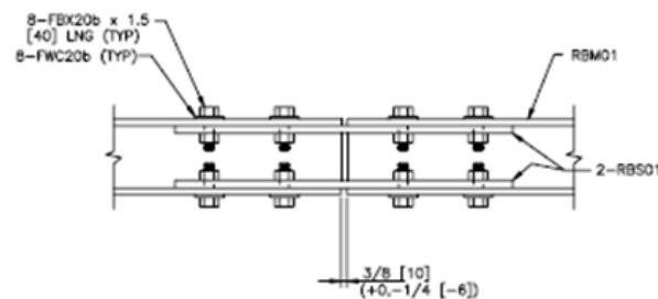
Figure 3.2. Detailed Drawings of (a) Box Beam Guardrail System; (b) Weak Steel Post; and (c) Splice Connections.
