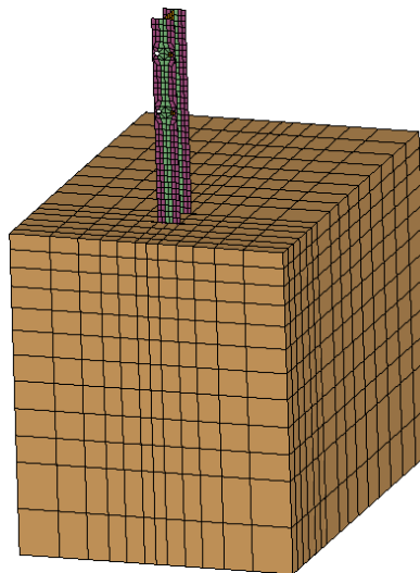
Figure 2.6. Post-Soil Interaction Model.
