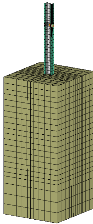
(a) Soil and post
