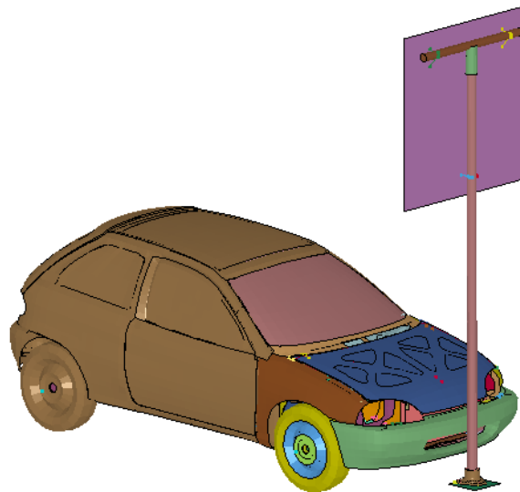
Figure 5.7. Finite Element Model of the Single Slip-Base Sign Support System.
