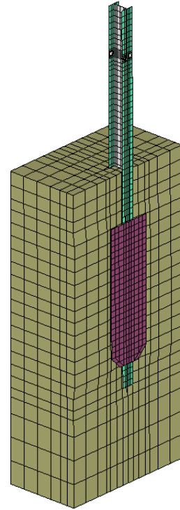
(b) Soil plate attached to post
