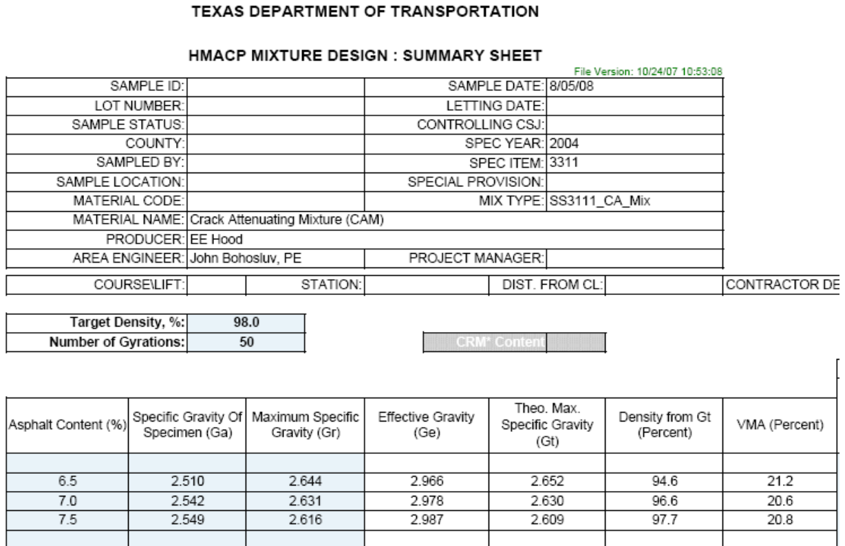
Figure 48. SS3109 CAM Mix Volumetric Design Results.
