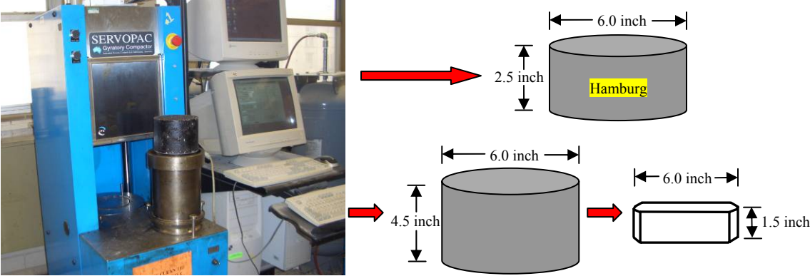
Figure 51. Molding Samples.
