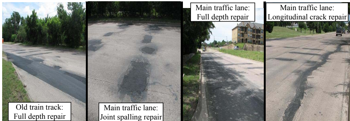
Figure 23. Repairs of Existing Distresses Before the HMA Overlay.
