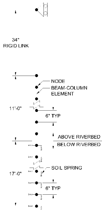
Figure 31. Analytical full-scale model of single pile.
