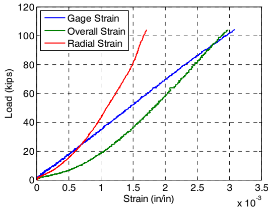
Figure 18. Typical monotonic strains.
