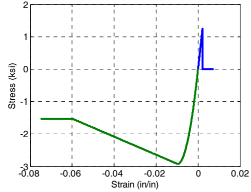
Figure 38. Analytical uniaxial constitutive relationship.
