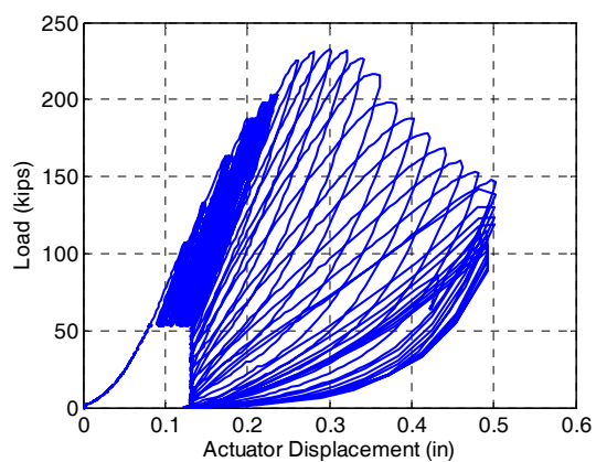
Figure C-17. Specimen SP7 load verses actuator displacement.
