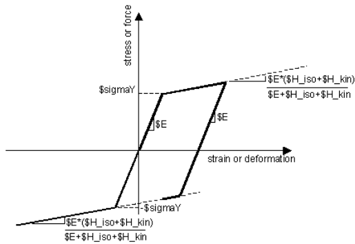
Figure 41. OpenSees Hardening material model (OpenSees, 2009).
