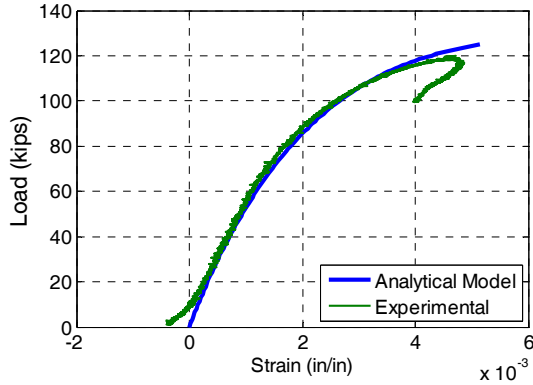
Figure 37. Strain in extreme tension fiber of compression-flexure test.
