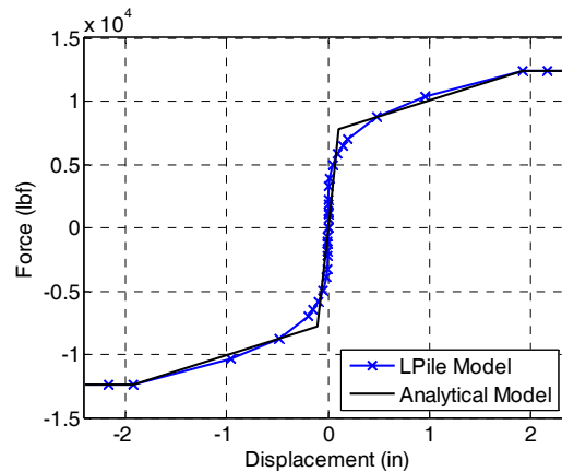
Figure 40. Typical geotechnical and computer model load-deformation response of lateral soil spring.
