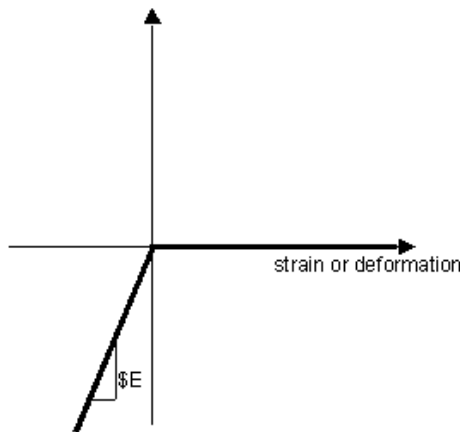
Figure 43. OpenSees Elastic-No Tension material model (OpenSees, 2009).
