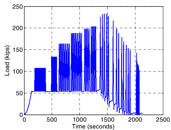
Figure C-18. Specimen SP7 load verses time.
