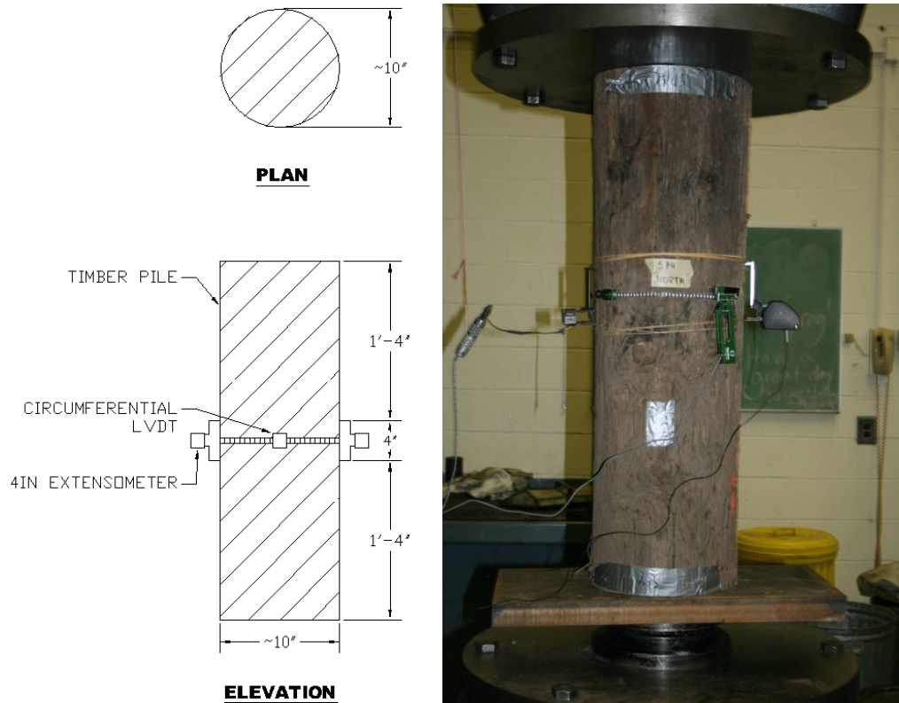
Figure 14. Experimental test instrumentation.
