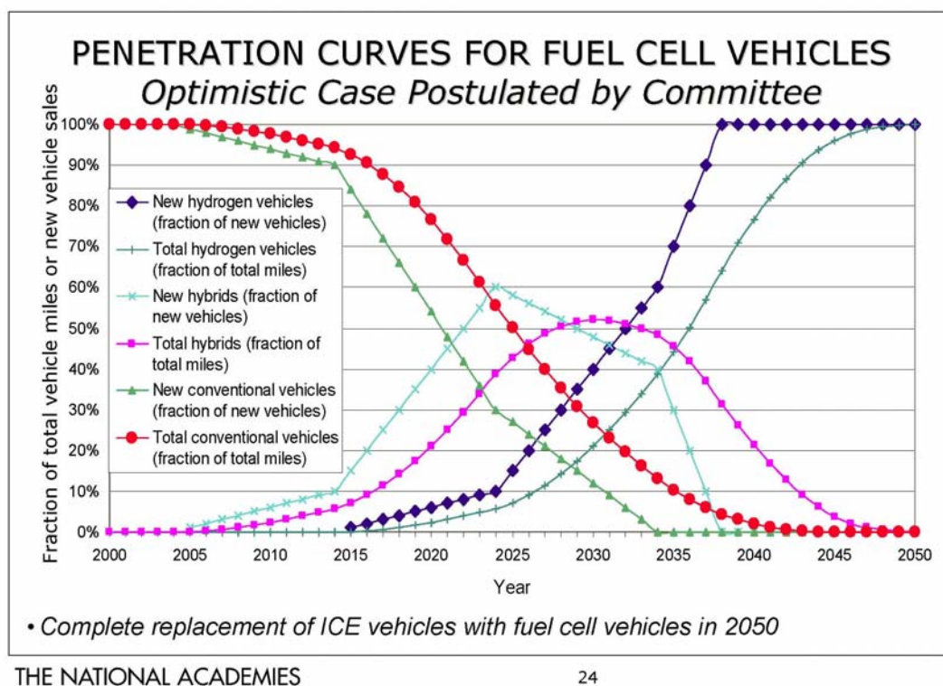
Figure 4. Penetration Curves for Hydrogen Fuel Cell Vehicles
