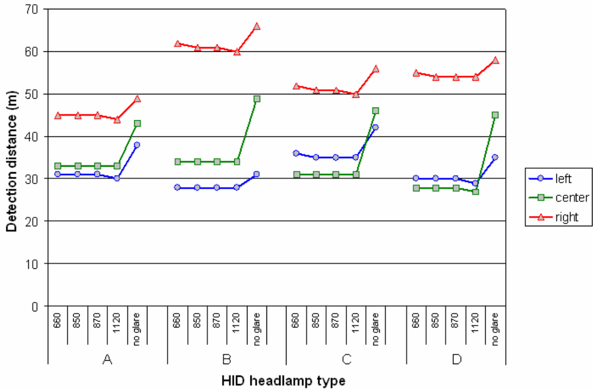
(a) HID headlamps
