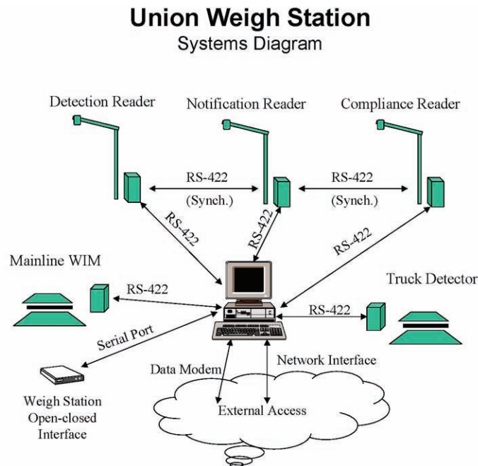
Source: Kentucky Transportation Center FIGURE II-2. "MODEL MACS"- THE MAINLINE AUTOMATED CLEARANCE SYSTEM: SYSTEM OVERVIEW AND IMPLEMENTATION GUIDE
