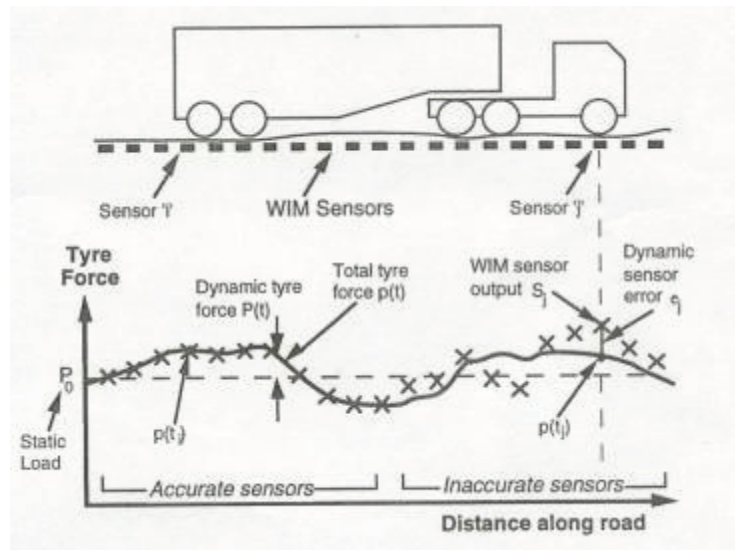
FIGURE A-3. VARIATION IN WIM SENSOR OUTPUT
