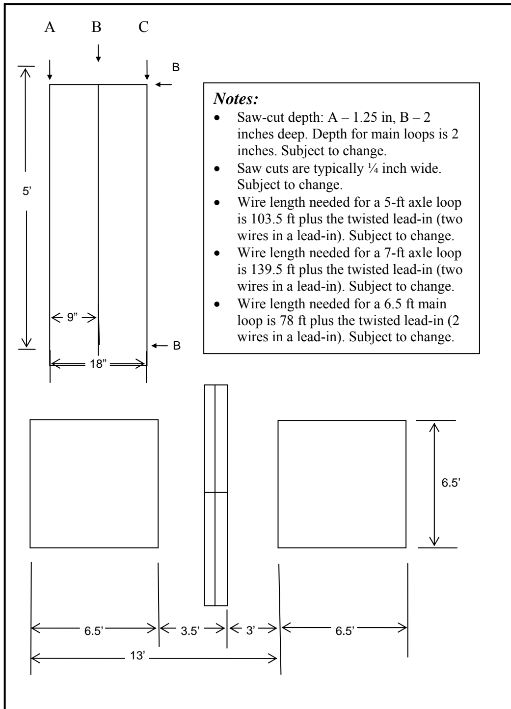
Figure 21: ADR-6000 Loop Layout
