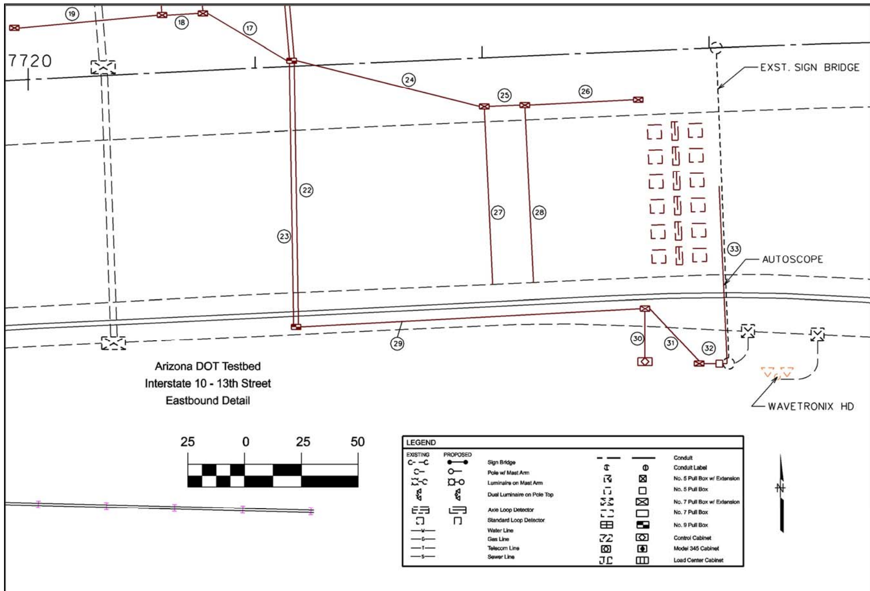
Figure 22b: Arizona DOT Testbed – Eastbound Direction
