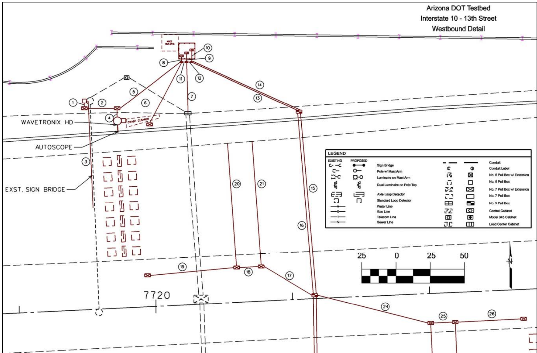
Figure 22a: Arizona DOT Testbed – Westbound Direction
