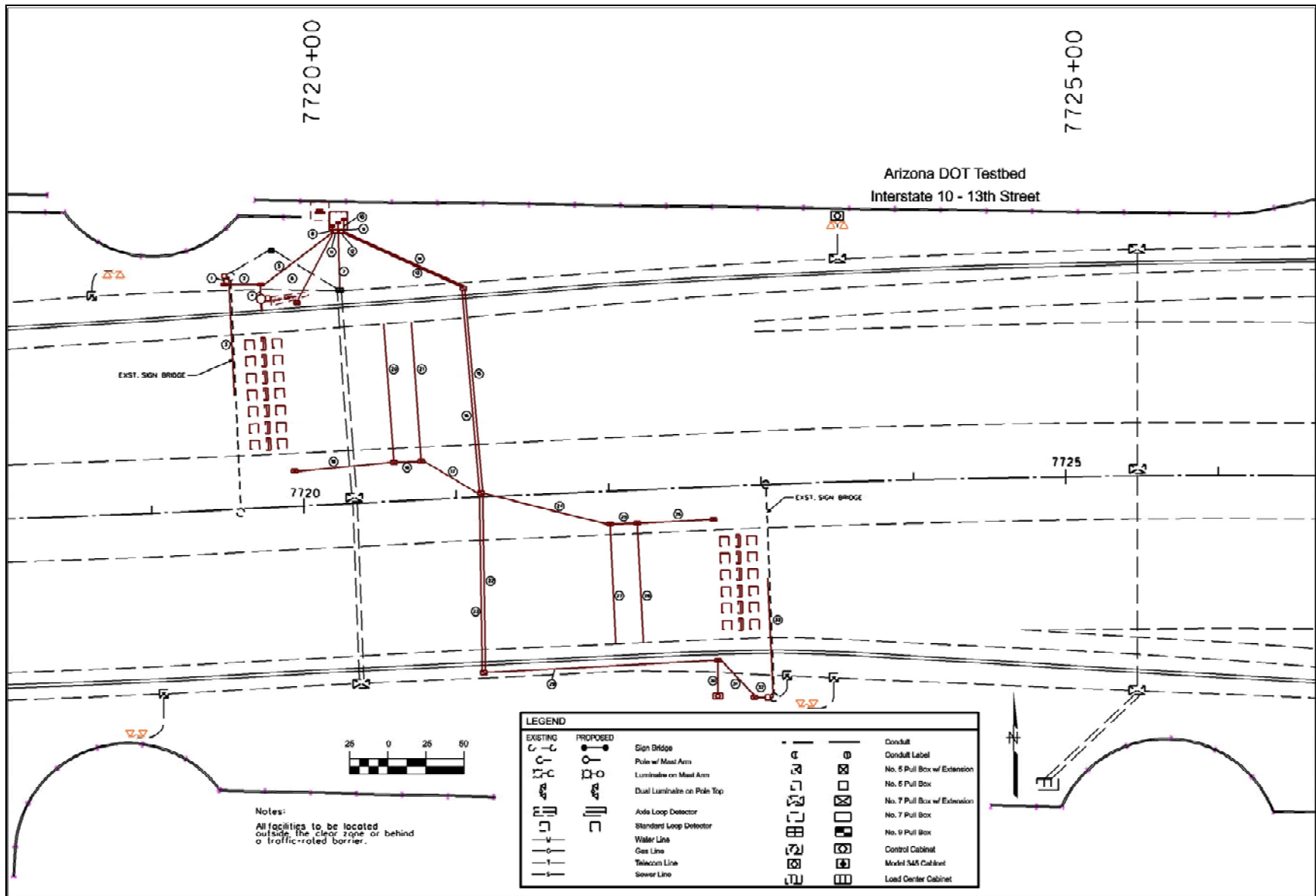
Figure 22: Arizona DOT Testbed – General Arrangement
