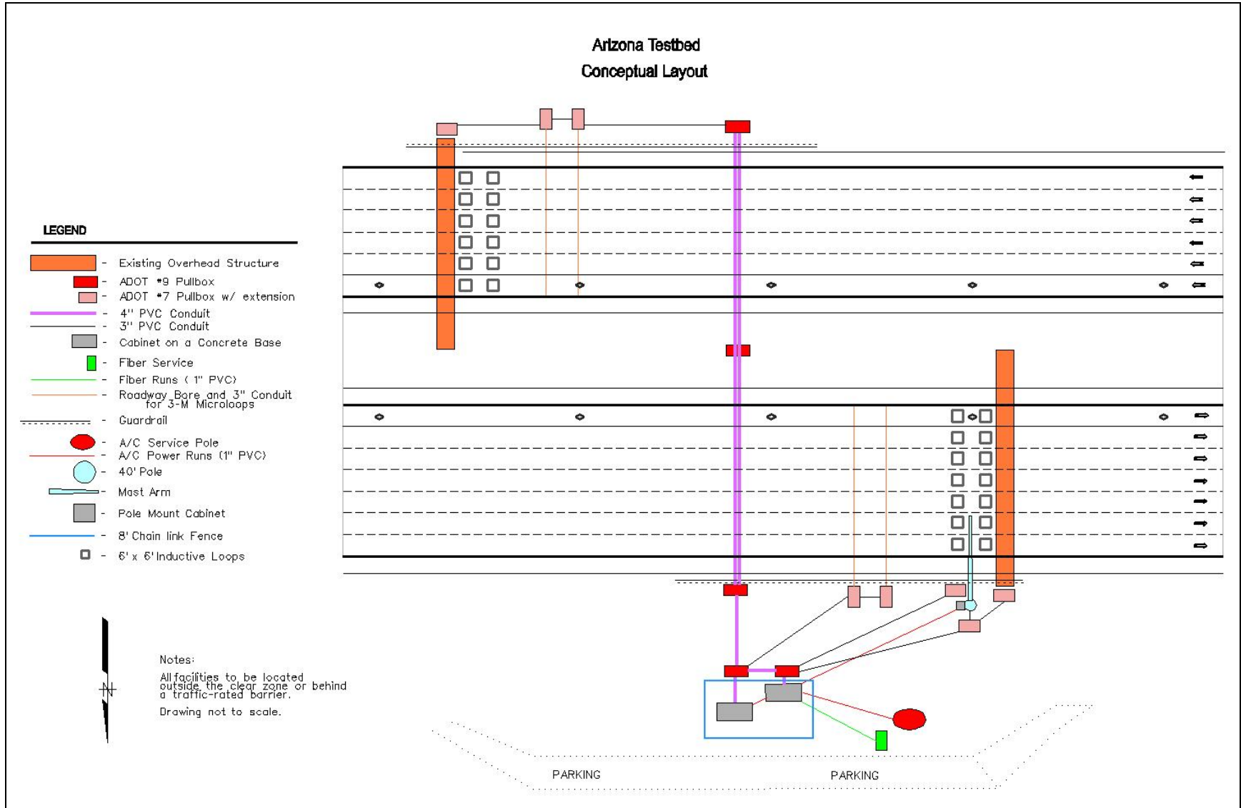
Figure 19: Conceptual Testbed Design
