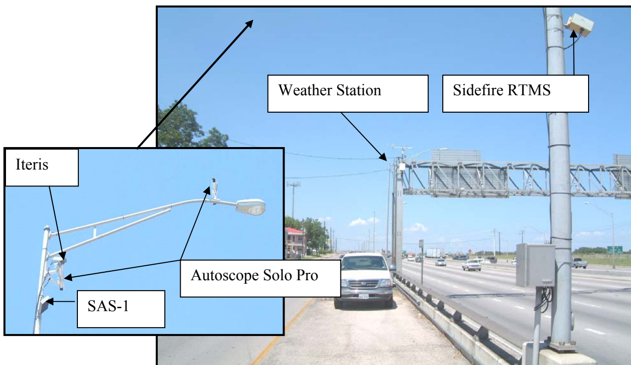
Figure 13: Views of I-35 Testbed
