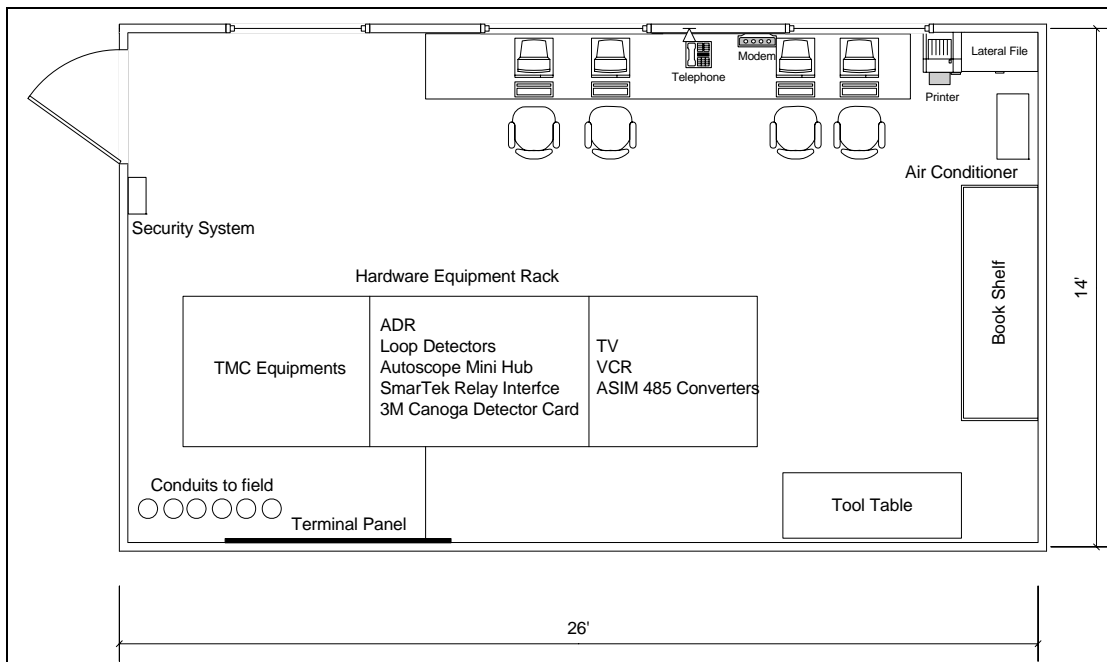
Figure 11: MnDOT Shelter Schematic Layout
