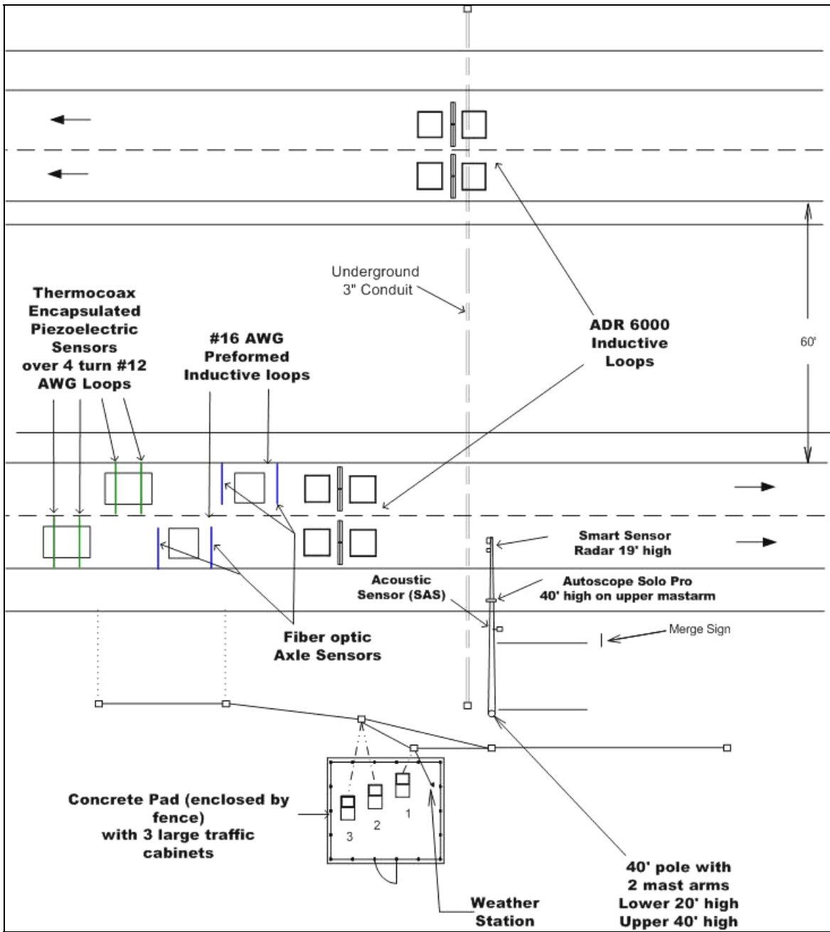
Figure 14: Layout of S.H. 6 College Station Testbed
