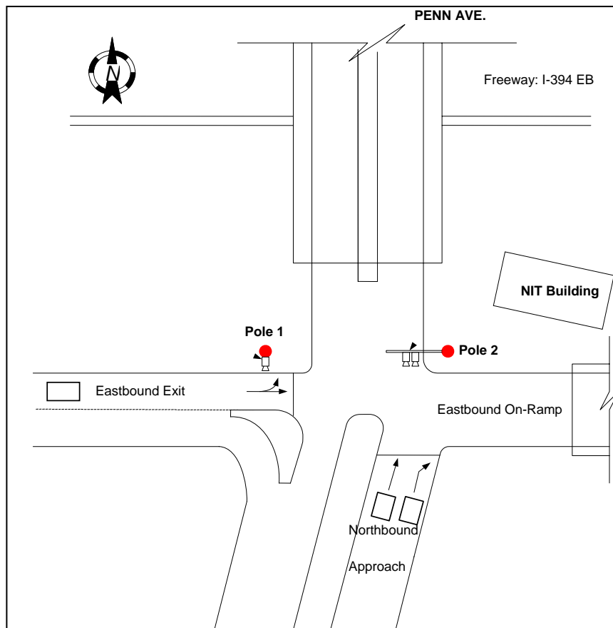
Figure 7: MnDOT NIT Site Layout
