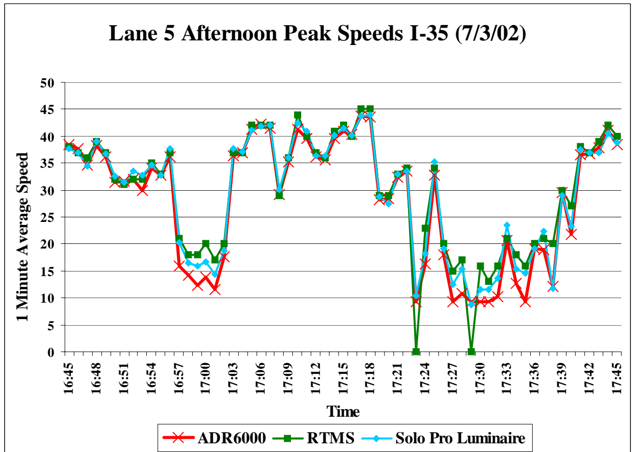
Figure 5: Speed Comparison of ADR-6000, Doppler Radar, and Video Imaging System
