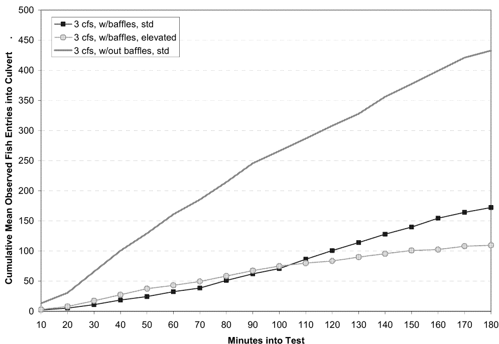
Figure 20. Real-Time Observations of Fish Entries into the Culvert from the Tailwater Tank, Cumulative Entries at 3 cfs
