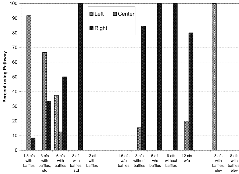
Figure 33. Percentage of Fish Observed Holding Between Baffle 1 and Baffle 2
