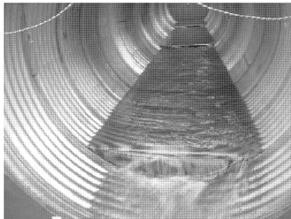
Figure 5. Standard Baffle Configuration
