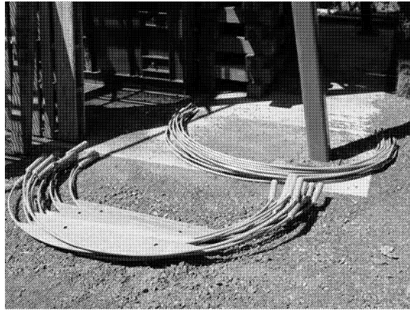
Figure 4. Two-Piece Baffles
