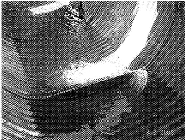
Figure 2. Washington Department of Fish and Wildlife Culvert-Retrofit Baffle Installation
