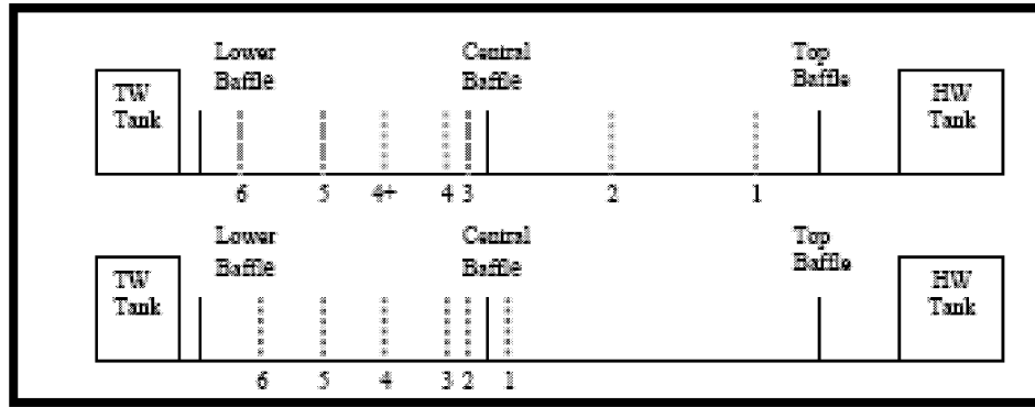
Figure 7. Hydraulic Measurement Locations. Water flows from right to left. Solid lines are baffles; dotted green line = fine grid; dotted red lines = coarse grid; dotted blue lines = super-fine grid.
