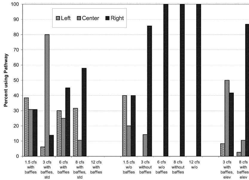
Figure 34. Percentage of Fish Observed Holding Between Baffle 2 and Baffle 3
