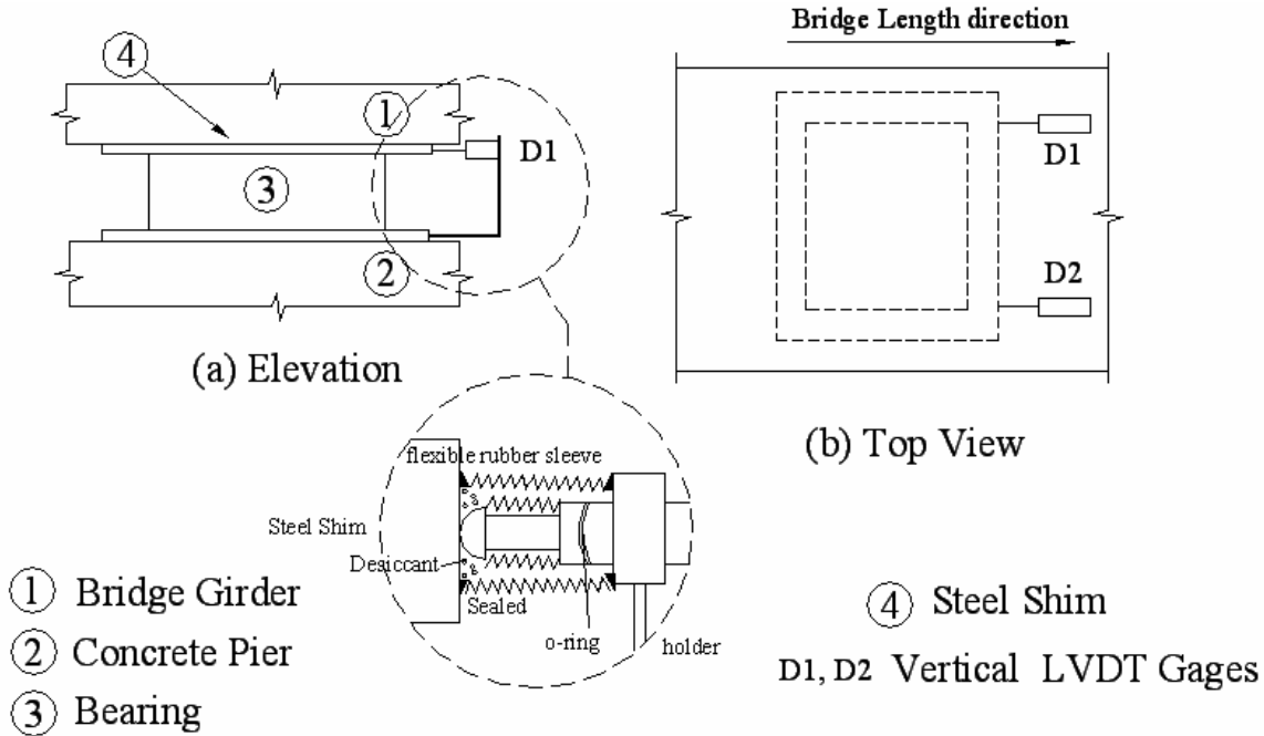
Figure 2.14. Instrumentation Design for Bearing Movements
