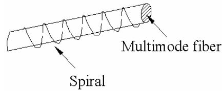
Figure 2.4. Fiber Optic Sensing Element
