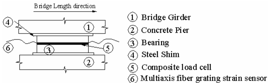
Figure 2.5. Bearing with Integrated Multi-Axis Fiber Grating Strain Sensors
