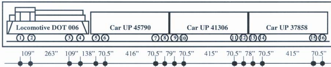
Figure 7. Test train axle spacing post-strengthening tests
