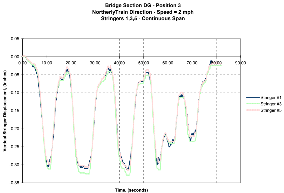
FIGURE 21-A. Transverse Response @ 2 mph
