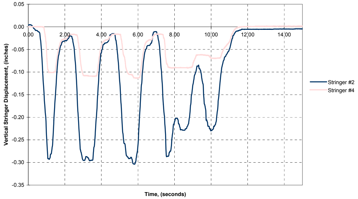
FIGURE 22-B. Transient Response @ 20 mph
