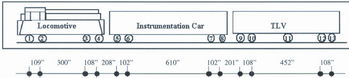
Figure 6. Test train axle spacing pre-strengthening tests
