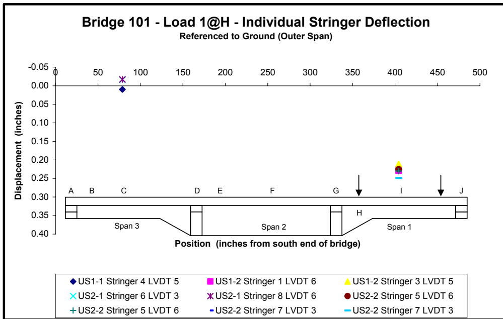
Figure 9. Transducer deflection measurements referenced to ground of Bridge 101 for load 1@H.
