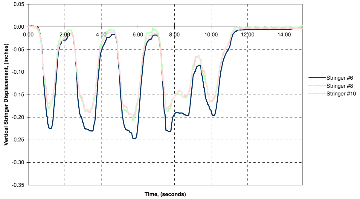
FIGURE 23-B. Transient Response @ 20 mph
