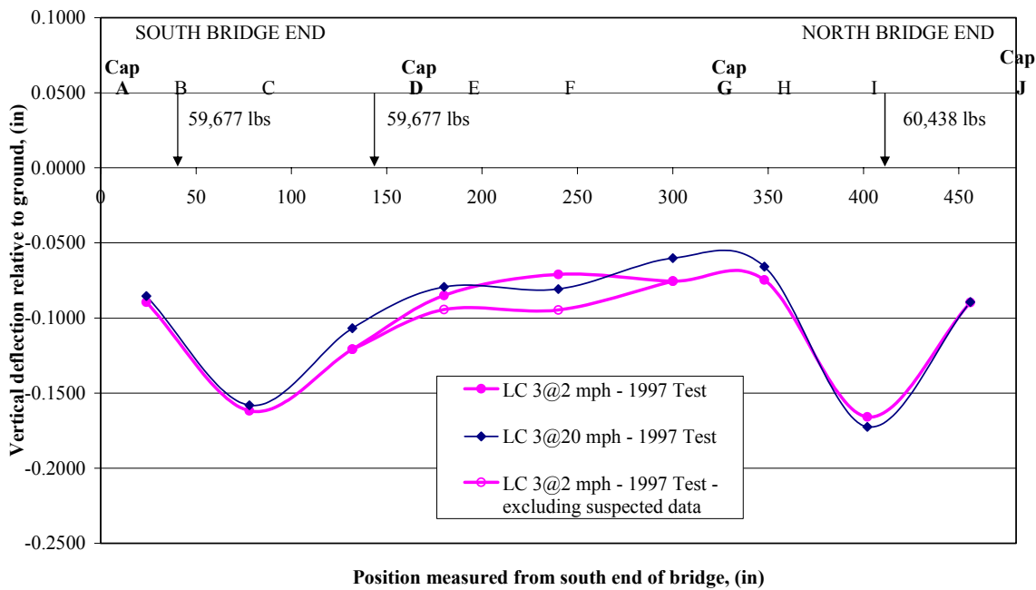
FIGURE 16. Load Case 3 - Post-Strengthening Test @ 2 mph and 20 mph
