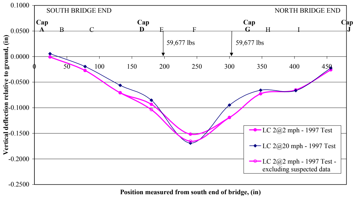
FIGURE 15. Load Case 2- Post-Strengthening Ttest @ 2 mph and 20 mph
