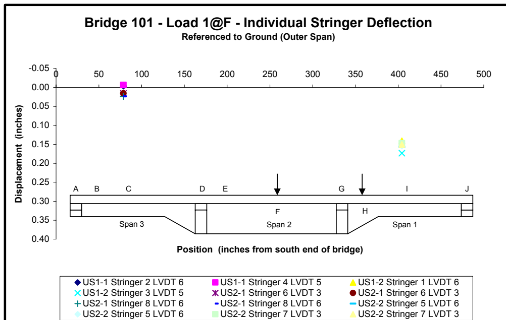
Figure 10. Transducer deflection measurements referenced to ground of Bridge 101 for load 1@F.
