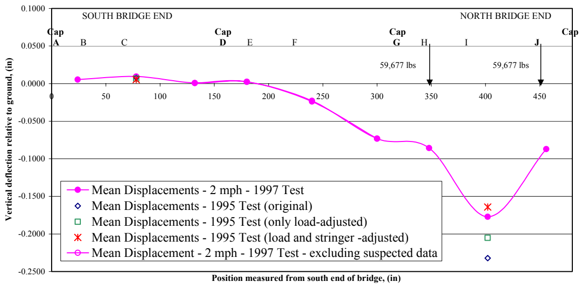
FIGURE 18. Load Case 1 (Load 1 @ H) Post-Strengthening Test vs. Pre-Strengthening Test
