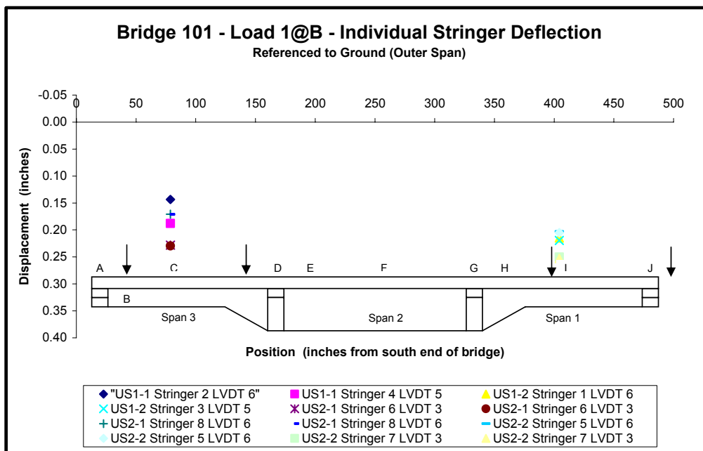
Figure 12. Transducer deflection measurements referenced to ground of Bridge 101 for load 1@B.
