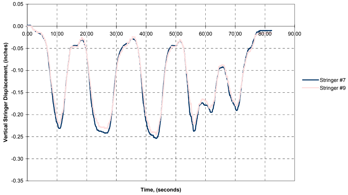
FIGURE 24-A. Transient Response @ 2 mph
