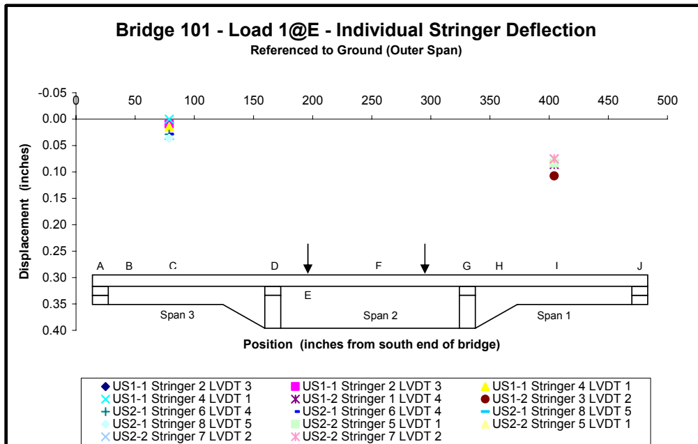
Figure 11. Transducer deflection measurements referenced to ground of Bridge 101 for load 1@E.
