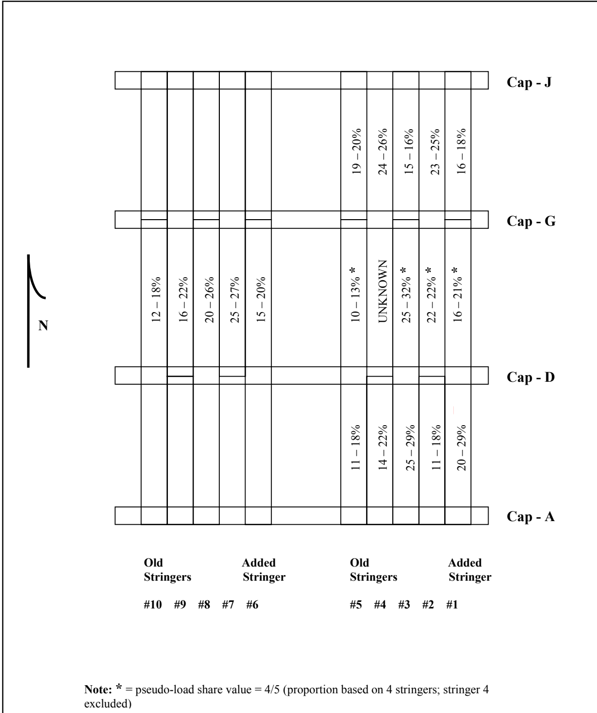
FIGURE 20. Bridge No. 101 - Load Share Ranges Based on the Post-Strengthening Measurements
