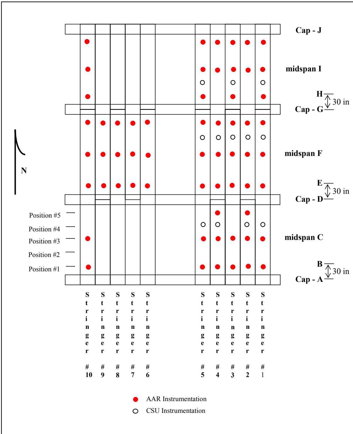
FIGURE 8. Bridge No. 101 - Plan View
