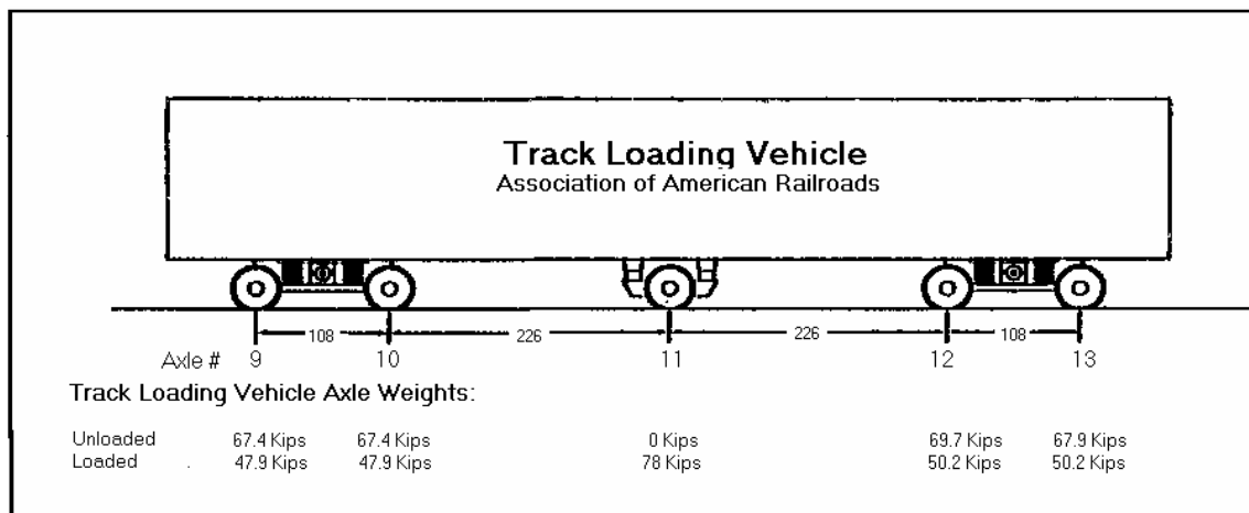
FIGURE 4. Track Loading Vehicle Schematic
