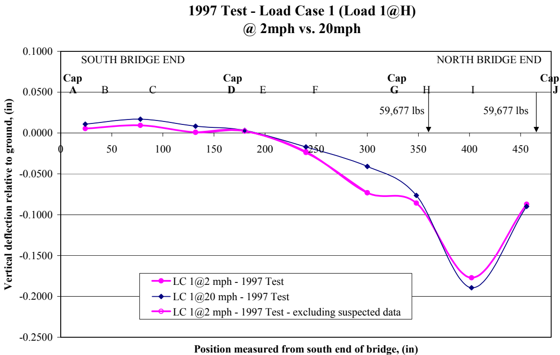
FIGURE 14. Load Case 1- Post-Strengthening Test @ 2 mph and 20 mph
