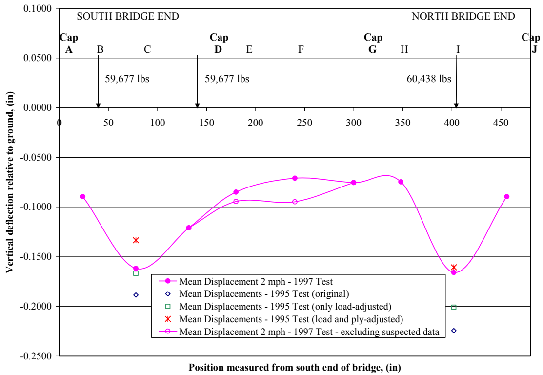
FIGURE 19. Load Case 3 (Load 1 @ B) Post-Strengthening Test vs. Pre-Strengthening Test
