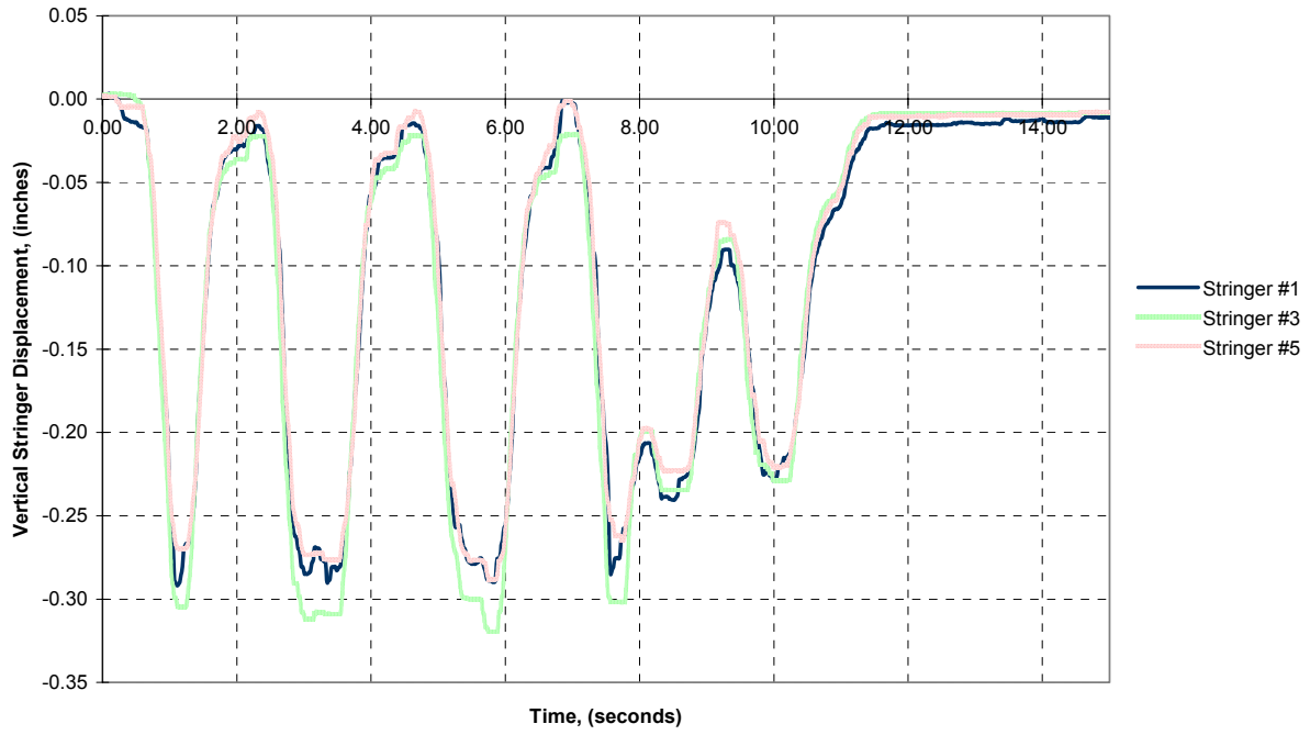
FIGURE 21-B. Transverse Response @ 20 mph
