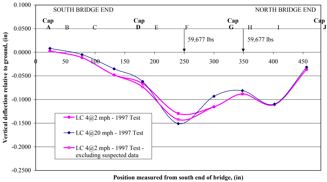
FIGURE 17. Load Case 4 Post-Strengthening Test @ 2 mph and 20 mph
