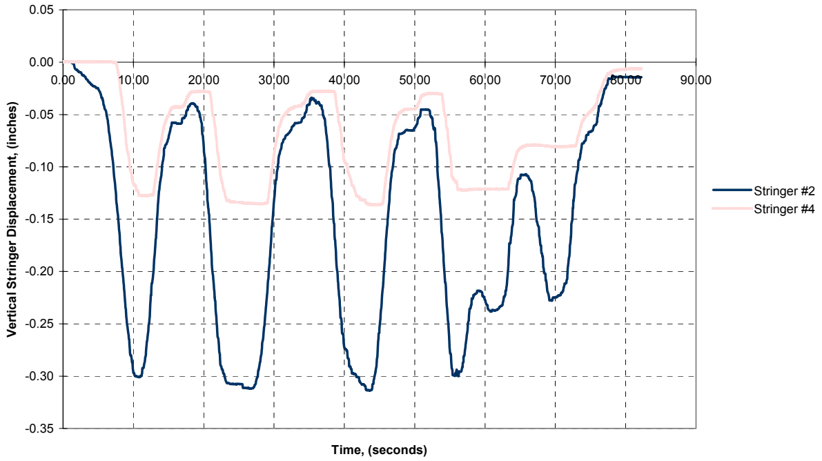
FIGURE 22-A. Transient Response @ 2 mph
