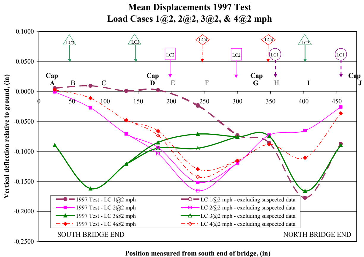
FIGURE 13. Mean Displacements Post-Strengthening Load Cases 1@2, 2@2, 3@2, and 4@2 mph.
