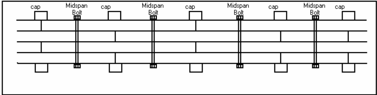
FIGURE 3. Typical placement of Members of Staggered Stringer Construction
