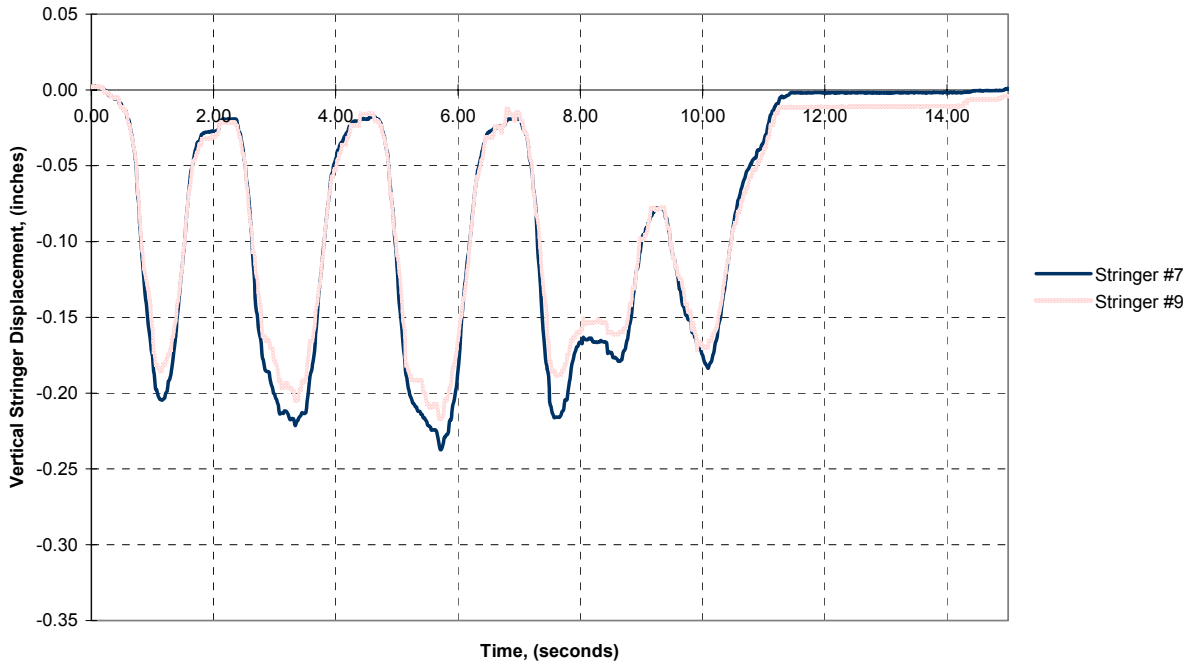
FIGURE 24-B. Transient Responses @ 20 mph
