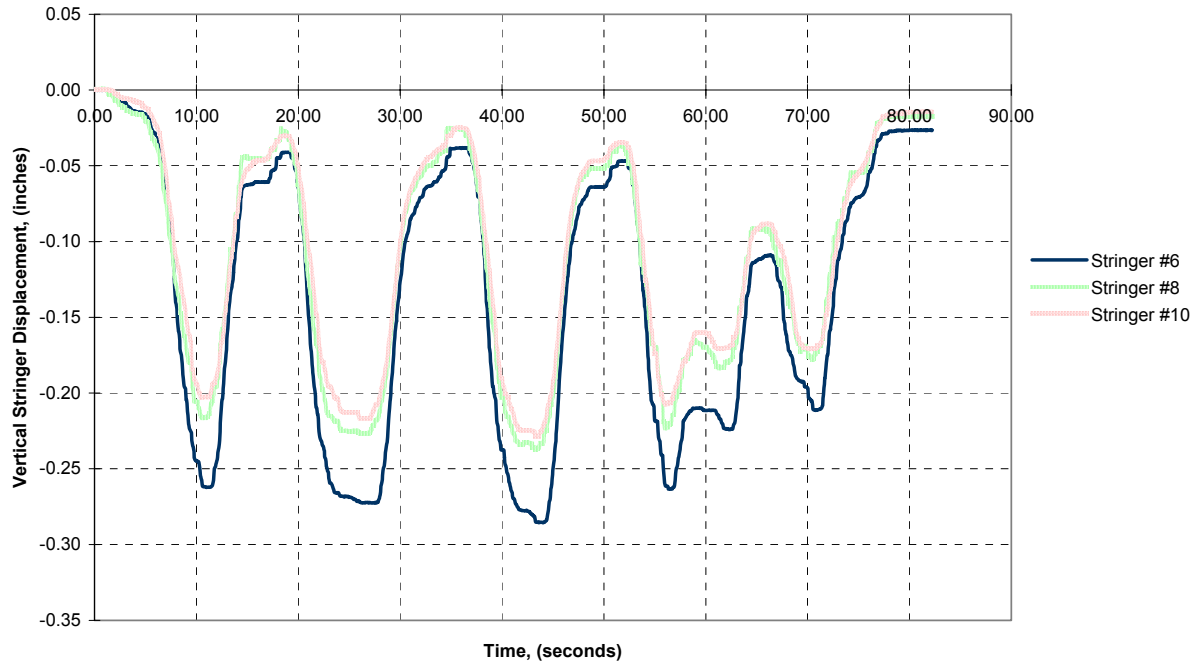
FIGURE 23-A. Transient Response @ 2 mph
