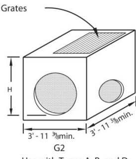
G2 Use with Types A, B, and D dikes when outlet pipe O.D. exceeds 24".
