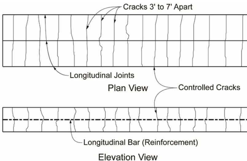
Continuously Reinforced Concrete Pavement (CRCP)
