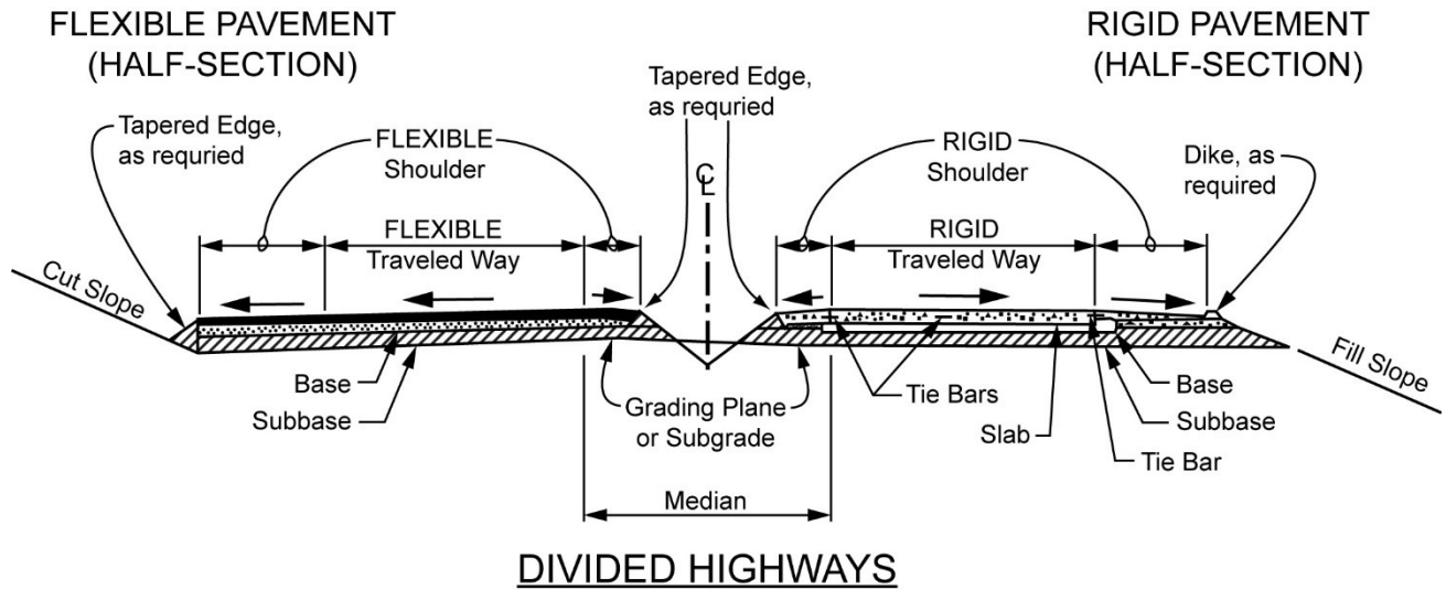
Figure 602.1 Basic Pavement Layers of the Roadway
