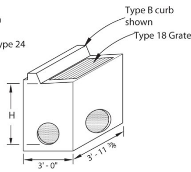
G5 Use with Types A and B curbs when height of inlet is 6' - 0" or less.
