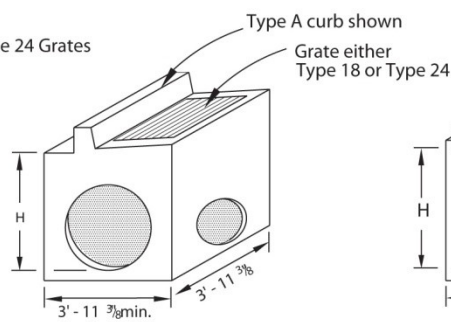
G4 Use with Types A and B curbs when outlet pipe O.D. exceeds 24".
