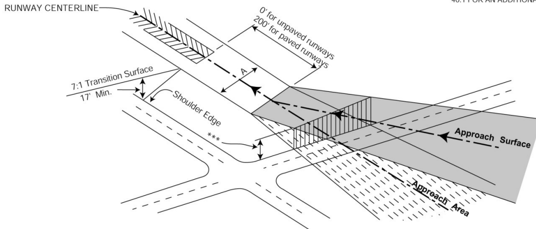
ISOMETRIC VIEW OF SECTION A-A
