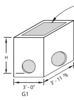
G1 Used when height of inlet is 6' - 0" or less.
