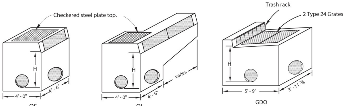
OL Curb opening lengths 7', 10', 14' and 21'. Use only with Type A and B curbs.
