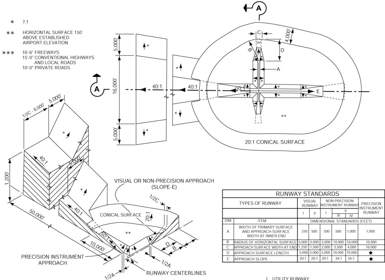
ISOMETRIC VIEW OF SECTION A-A
