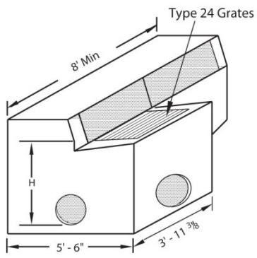
GOL Curb opening lengths 7' and 10'. Use with Types A and B curbs.
