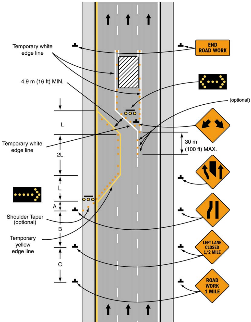
Typical Application 38
