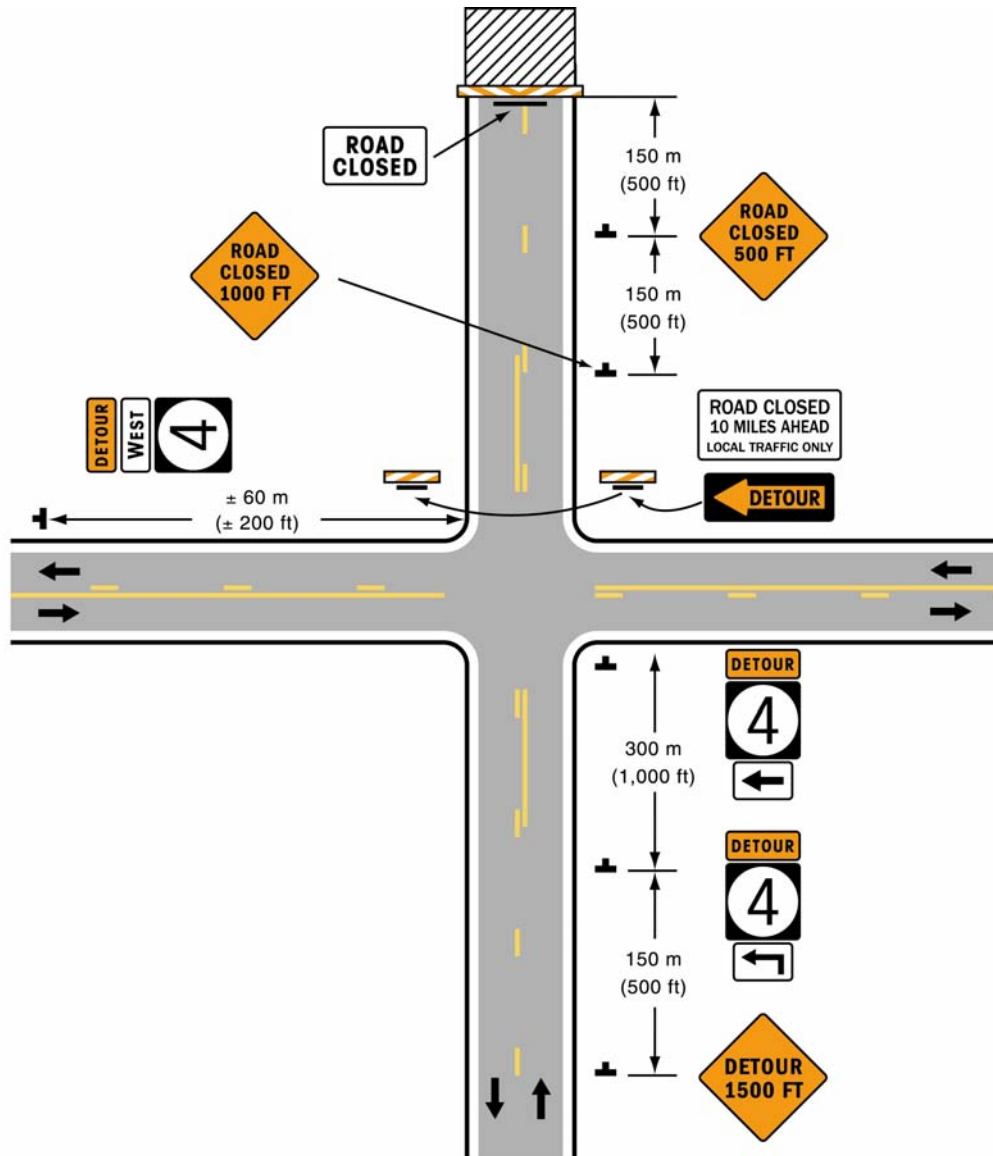
Typical Application 8
