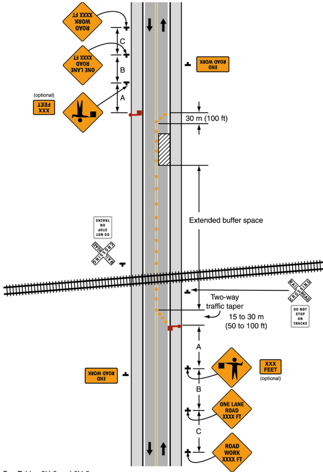
Typical Application 46
