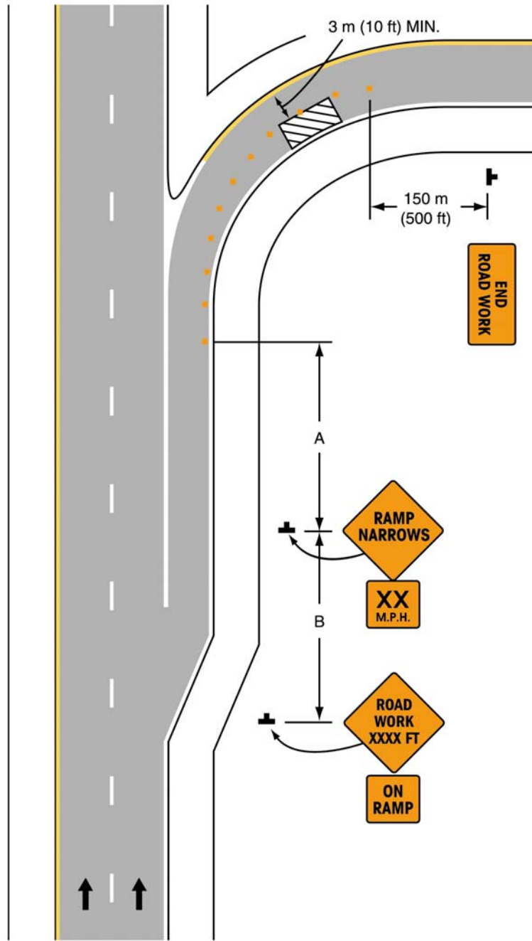
Typical Application 43
