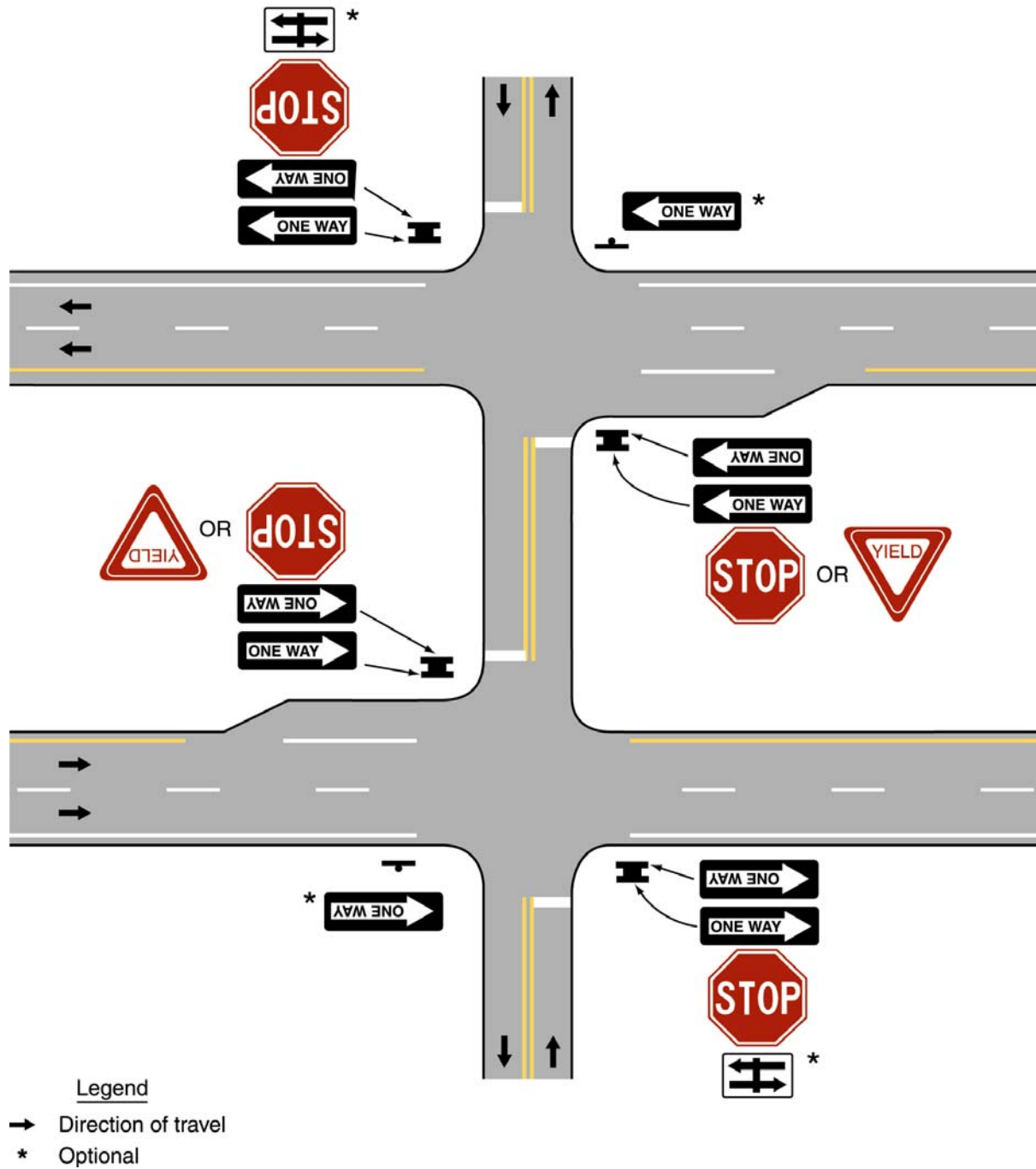
Figure 2A-4. Typical ONE WAY Signing for Divided Highways with Medians Greater Than 9 m (30 ft)
