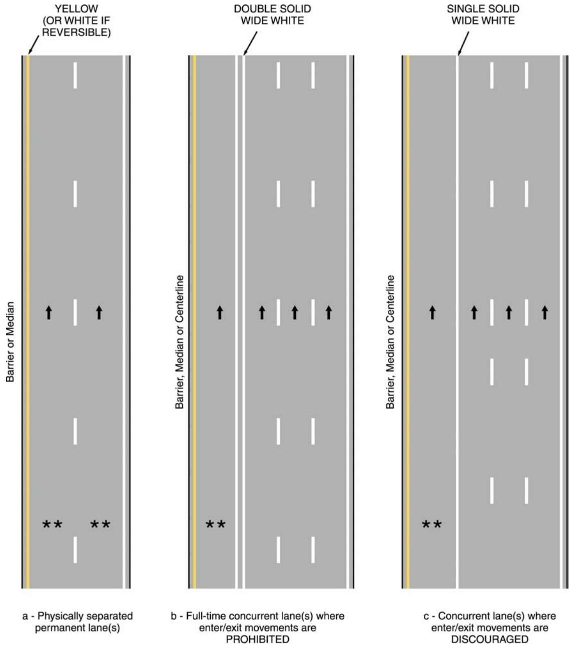
Figure 3B-25. Typical Markings for Preferential Lanes for Motorized Vehicles (Sheet 1 of 2)
