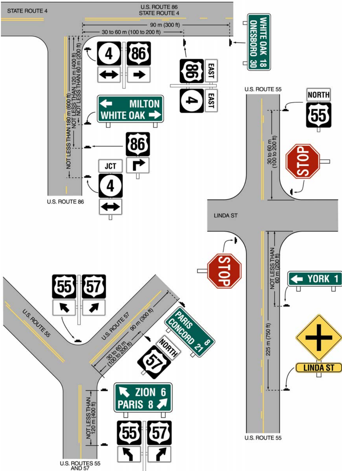
Figure 2D-2. Illustration of Directional Assemblies and Other Route Signs (For One Direction of Travel Only) (Sheet 3 of 3)
