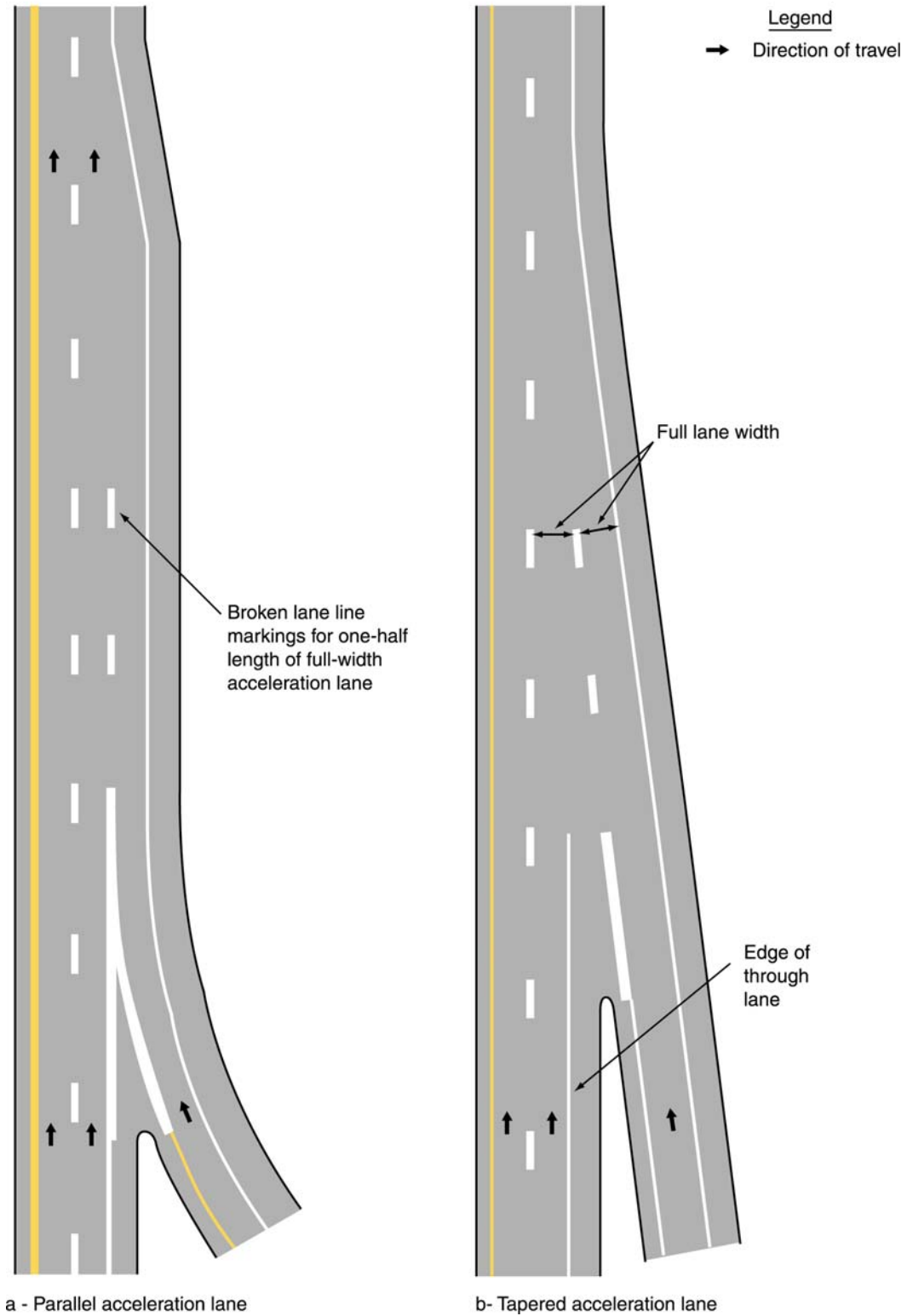
Figure 3B-9. Typical Entrance Ramp Markings
