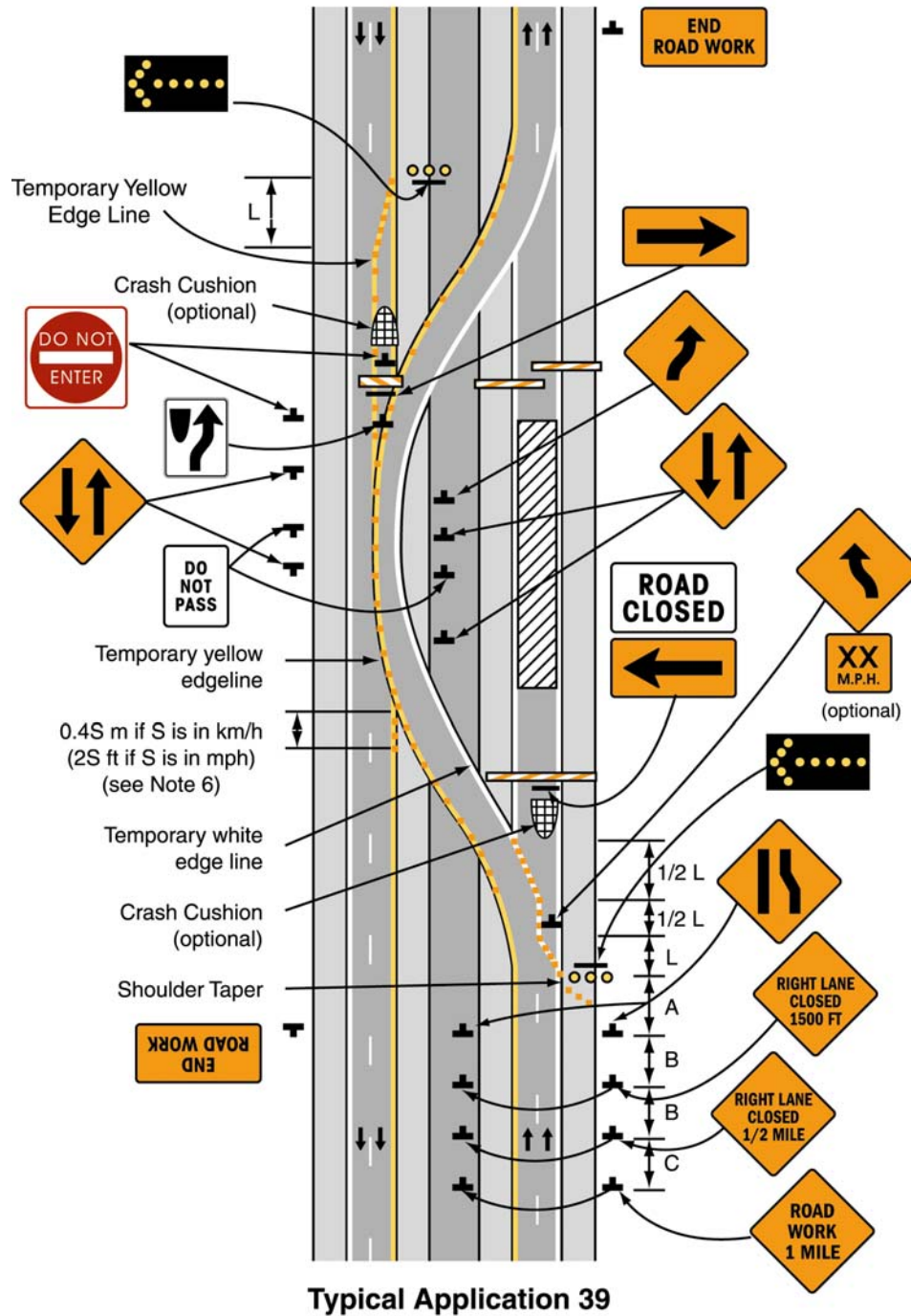
Figure 6H-39. Median Crossover on Freeway (TA-39)
