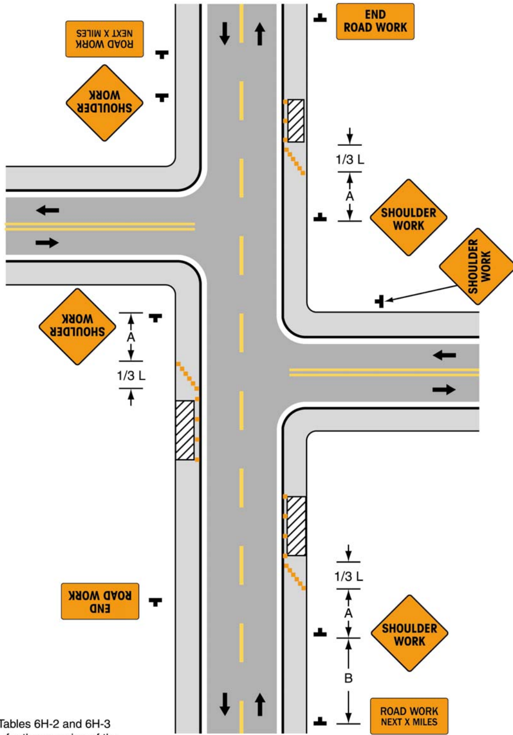
Typical Application 3
