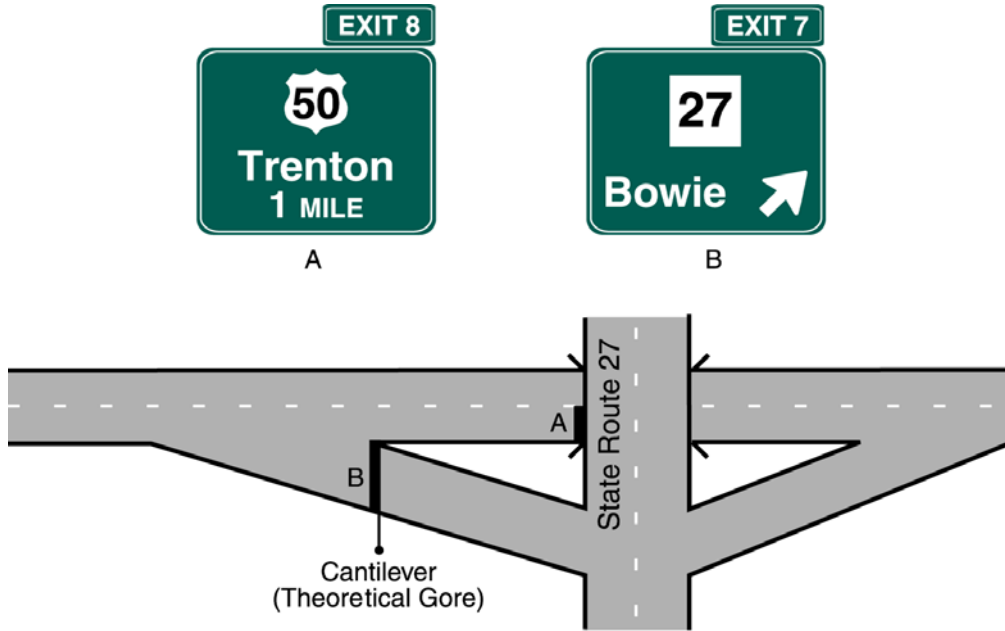
Figure 2E-1. Example of Guide Sign Spreading
