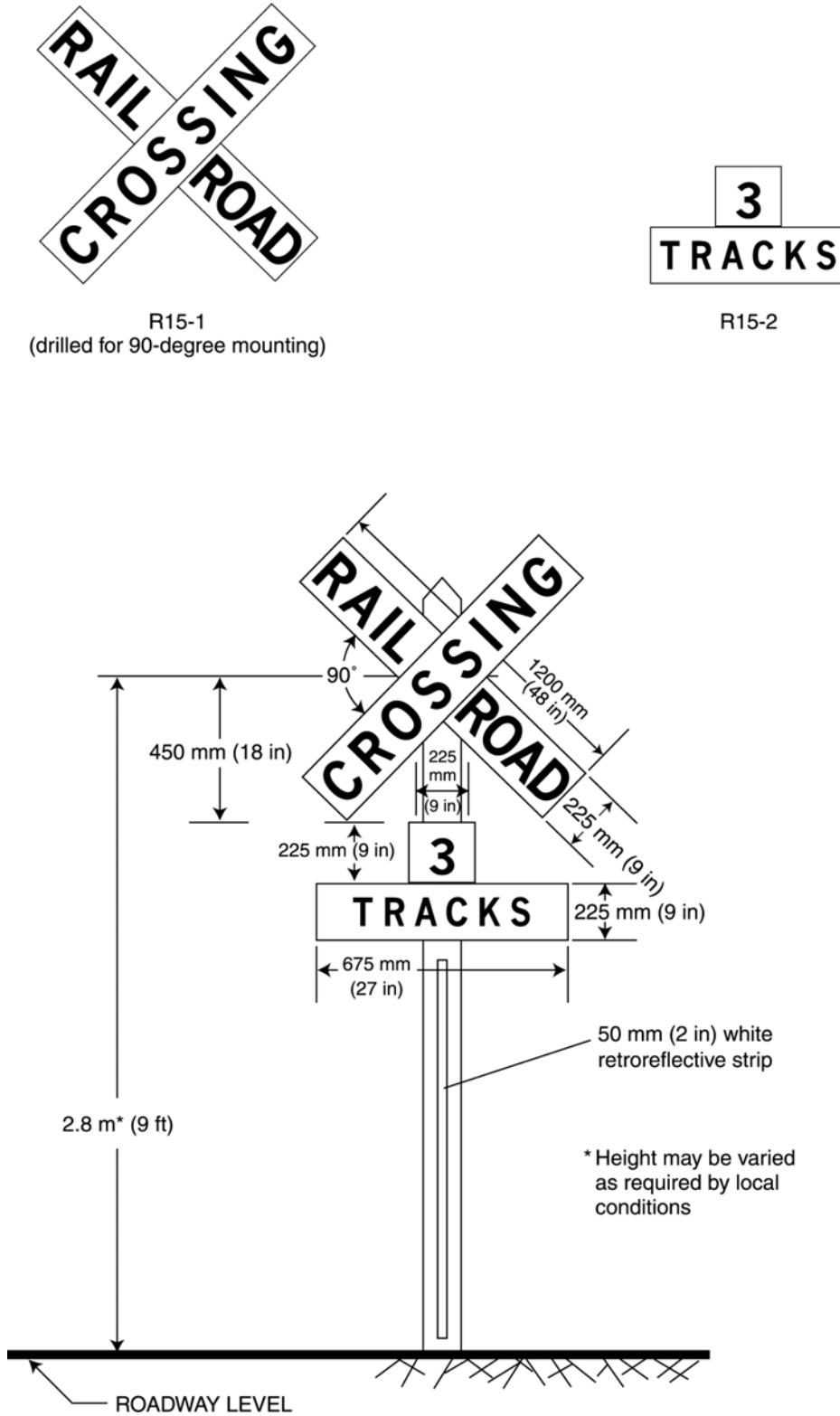
Figure 8B-1. Highway-Rail Grade Crossing (Crossbuck) Signs
