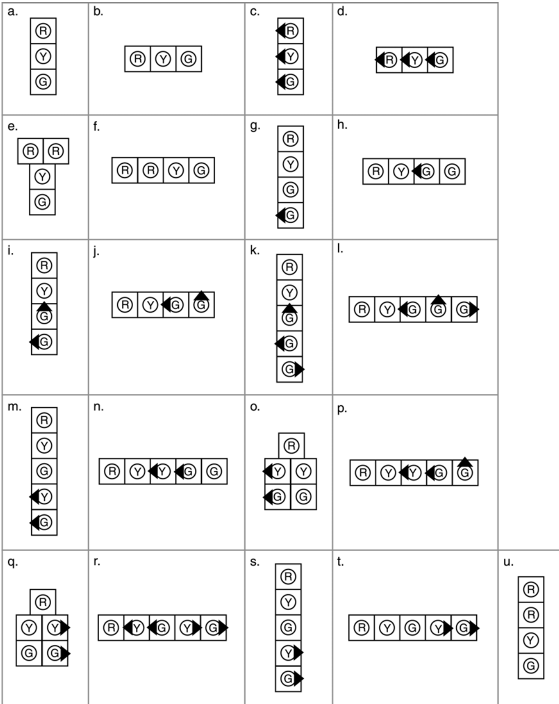
Figure 4D-3. Typical Arrangement of Signal Lenses in Signal Faces
