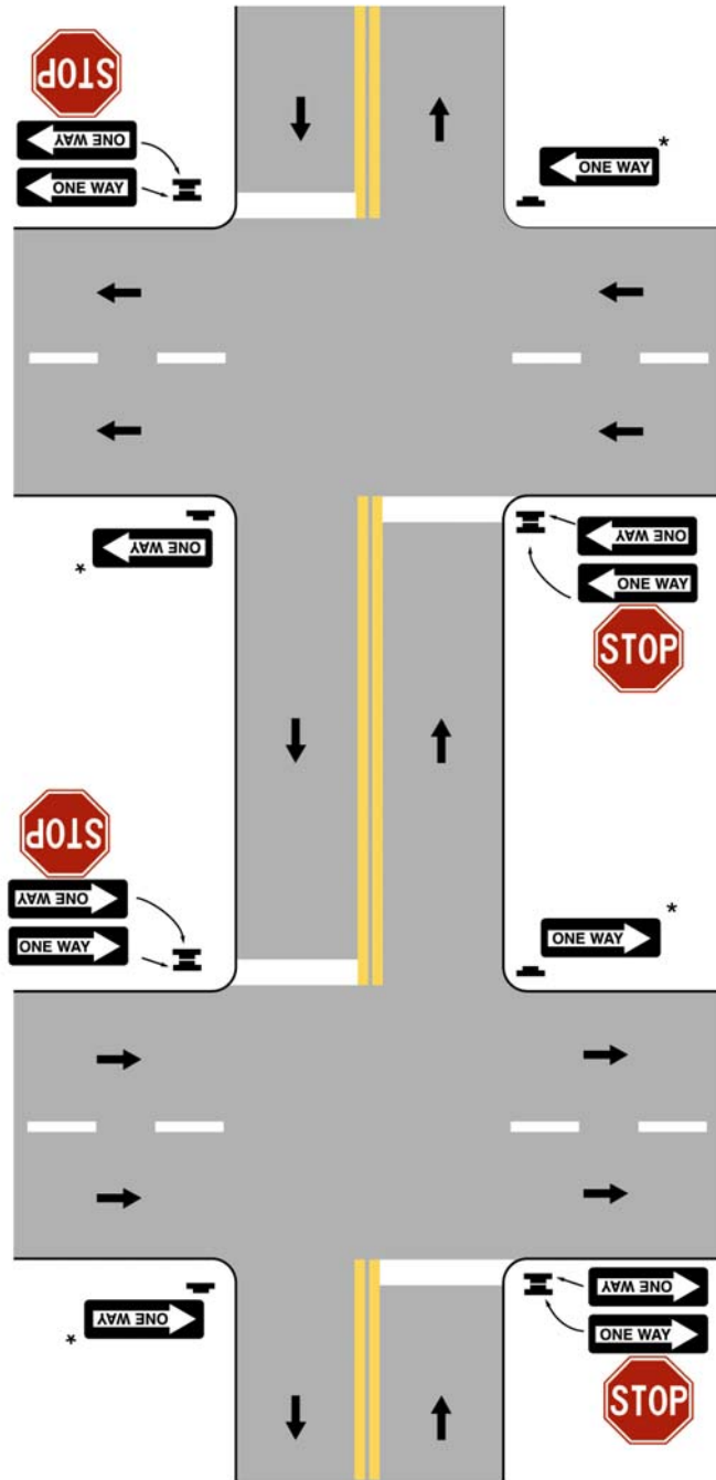
Figure 2A-5. Typical Locations of ONE WAY Signs
