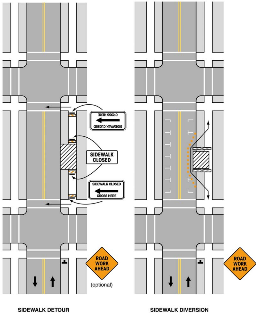
Figure 6H-28. Sidewalk Detour or Diversion (TA-28)
