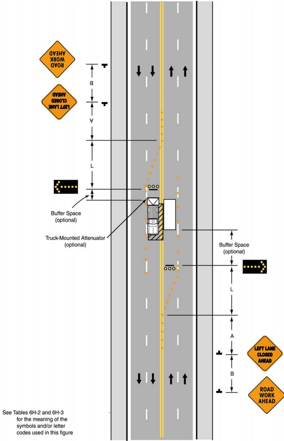
Typical Application 30
