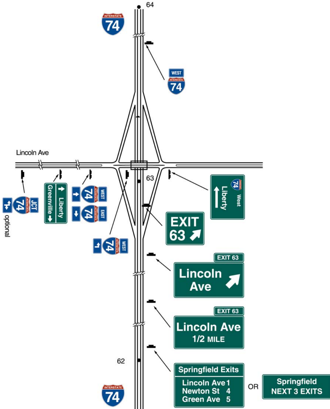
Figure 2E-29. Typical Urban Diamond Interchange Signs
