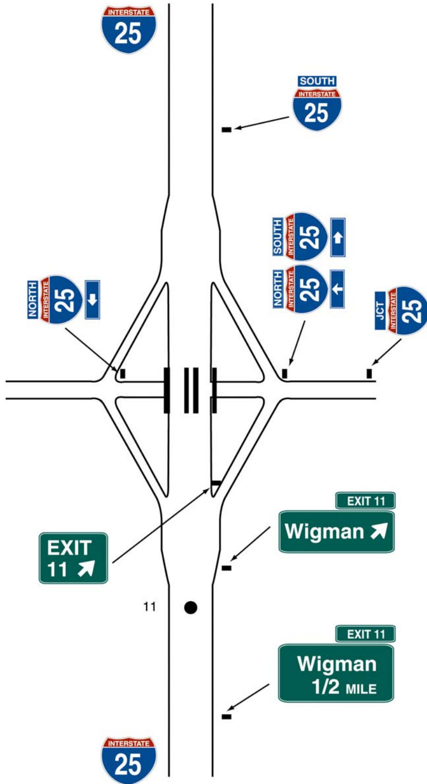
Figure 2E-30. Typical Minor Interchange Guide Signs
