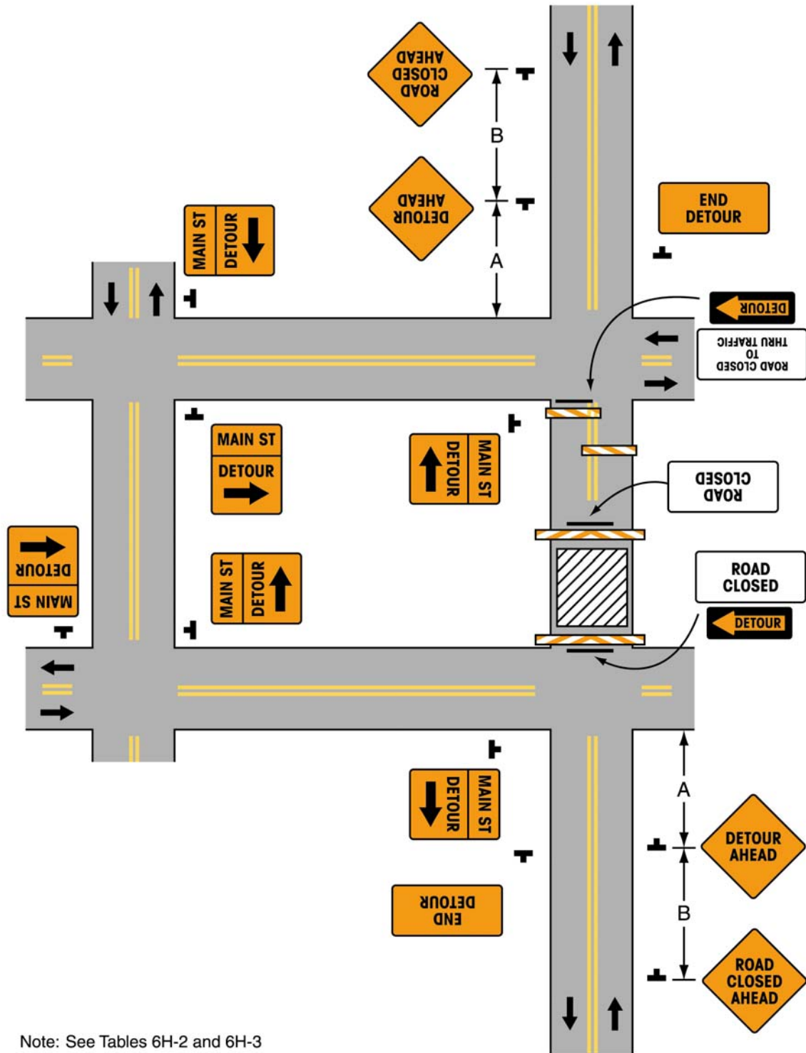
Typical Application 20
