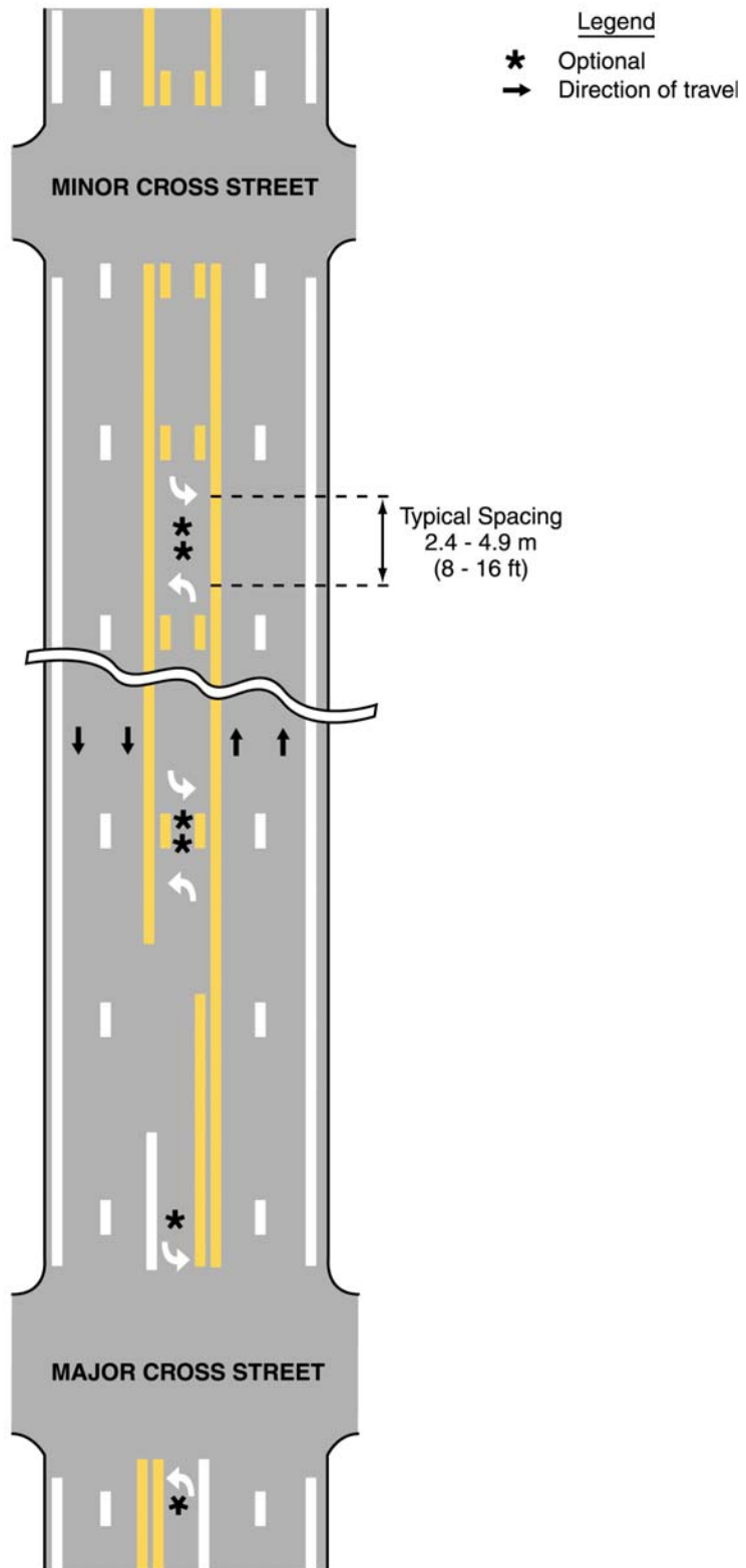
Figure 3B-7. Typical Two-Way Left-Turn Marking Applications
