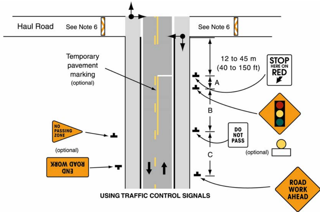
Figure 6H-14. Haul Road Crossing (TA-14)
