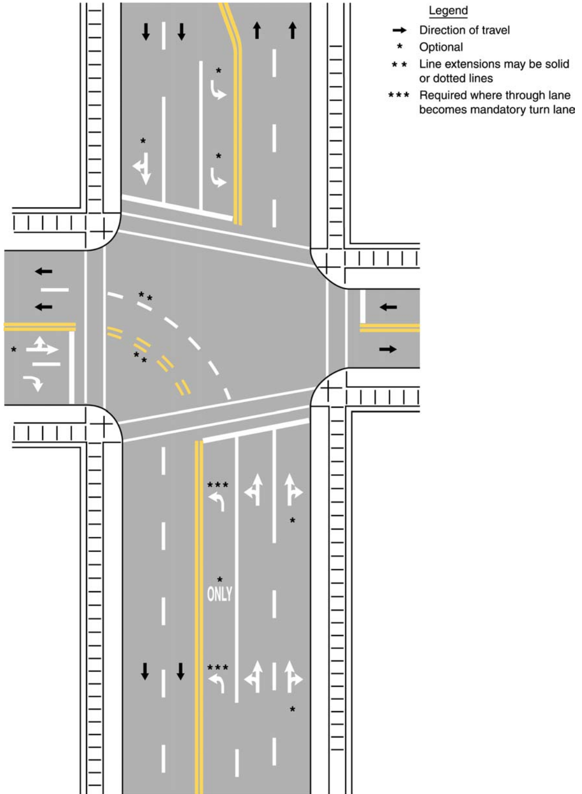
Figure 3B-21. Typical Lane Use Control Word and Symbol Markings
