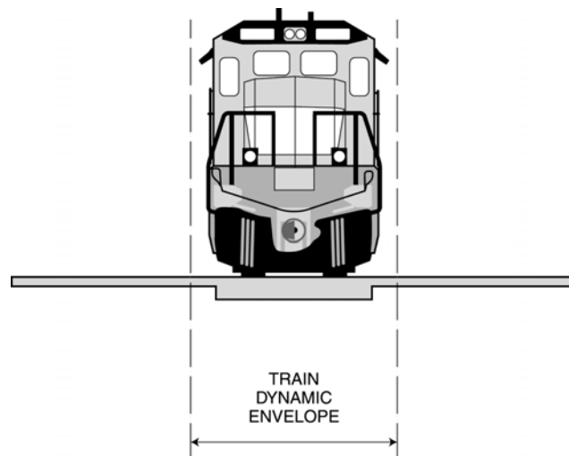
Figure 8A-1. Train Dynamic Envelope Delineation
