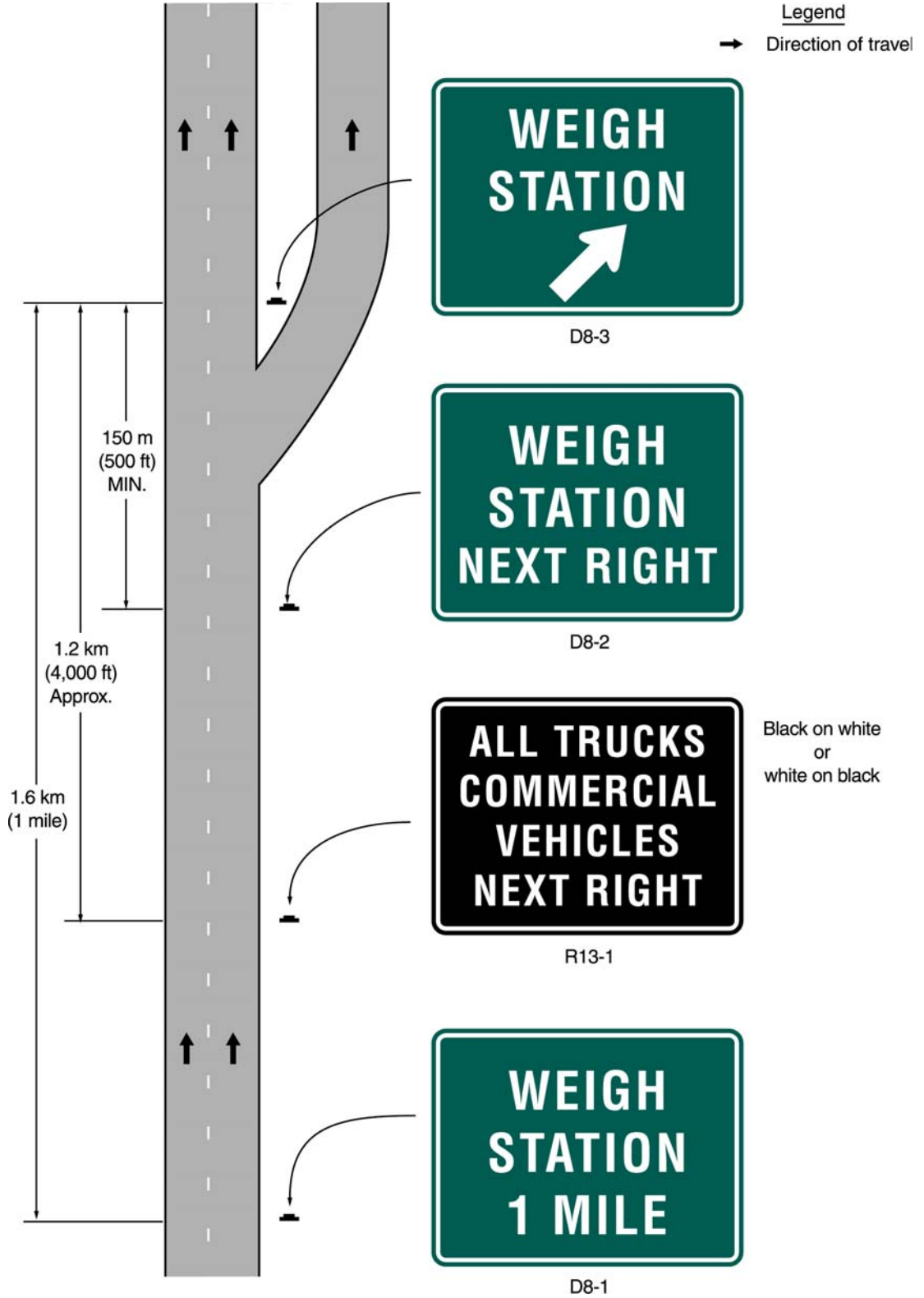
Figure 2D-3. Typical Weigh Station Signing
