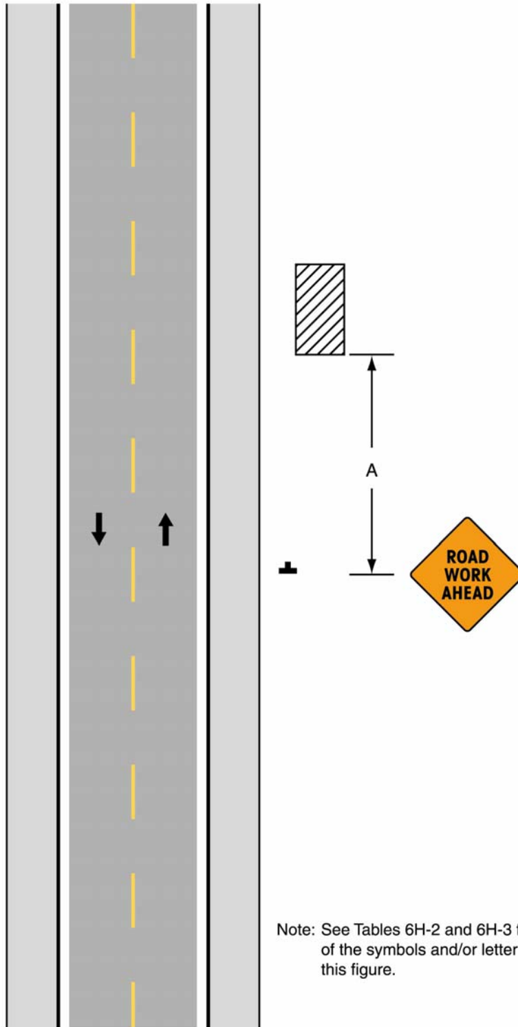
Typical Application 1
