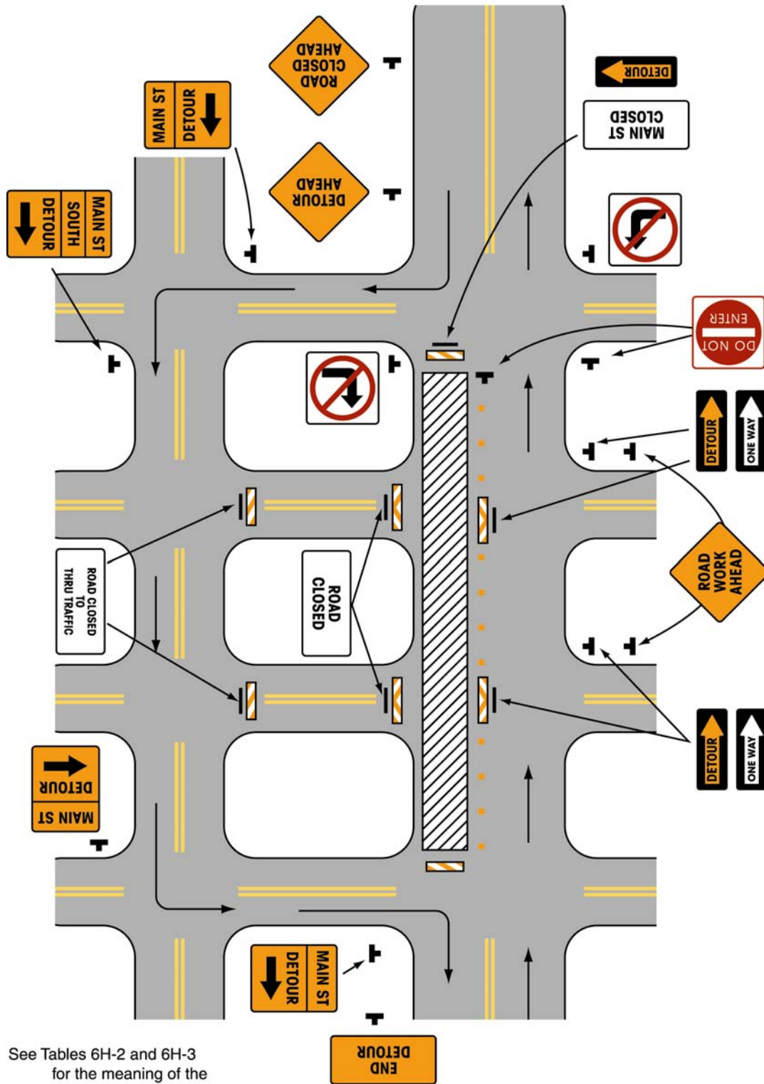
Figure 6H-19. Detour for One Travel Direction (TA-19)
