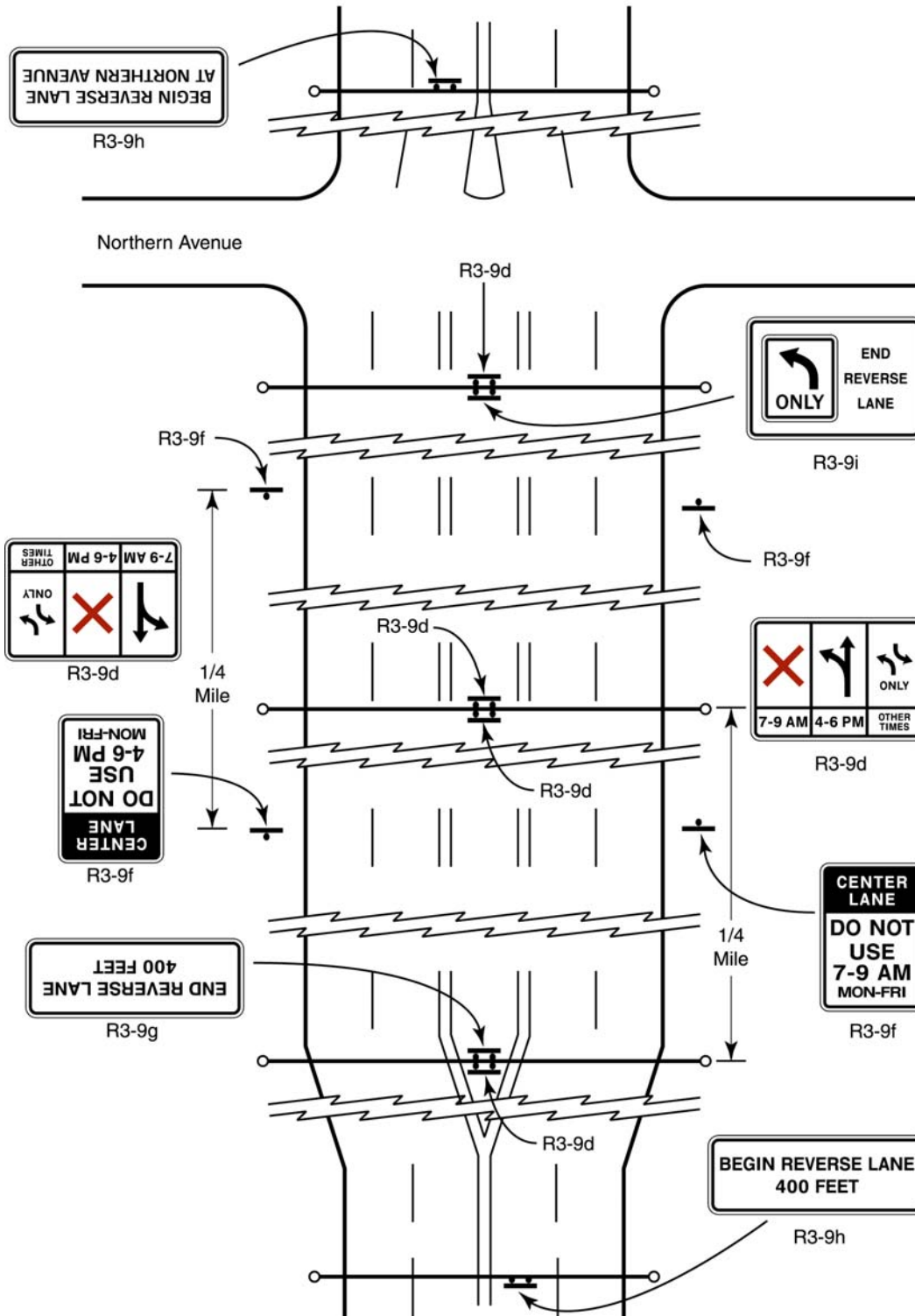
Figure 2B-1. Location of Reversible Two-Way Left-Turn Signs
