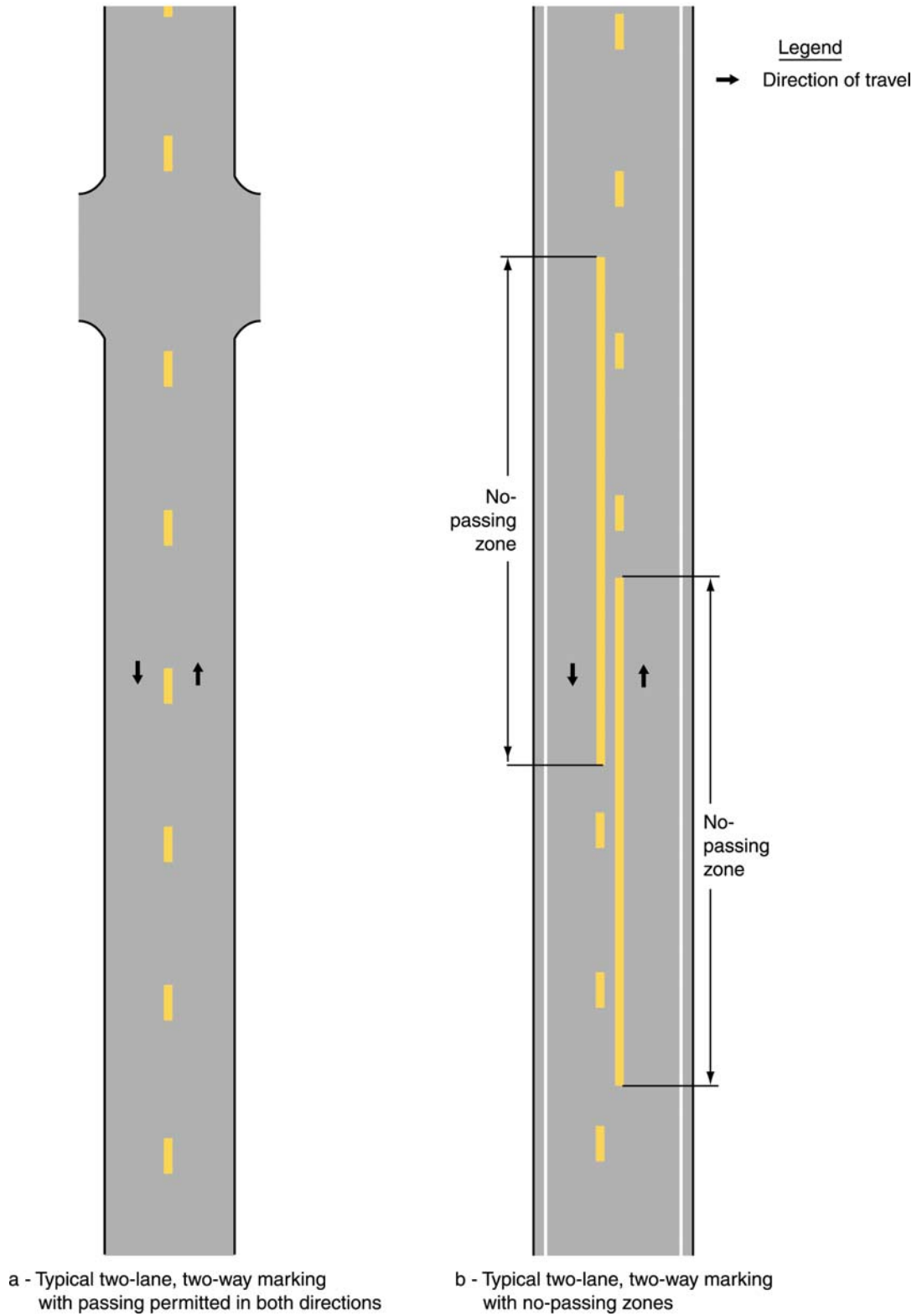
Figure 3B-1. Typical Two-Lane, Two-Way Marking Applications
