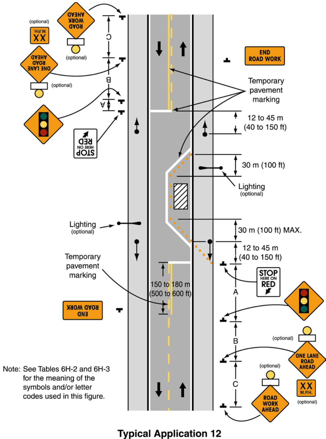
Figure 6H-12. Lane Closure on Two-Lane Road Using Traffic Control Signals (TA-12)
