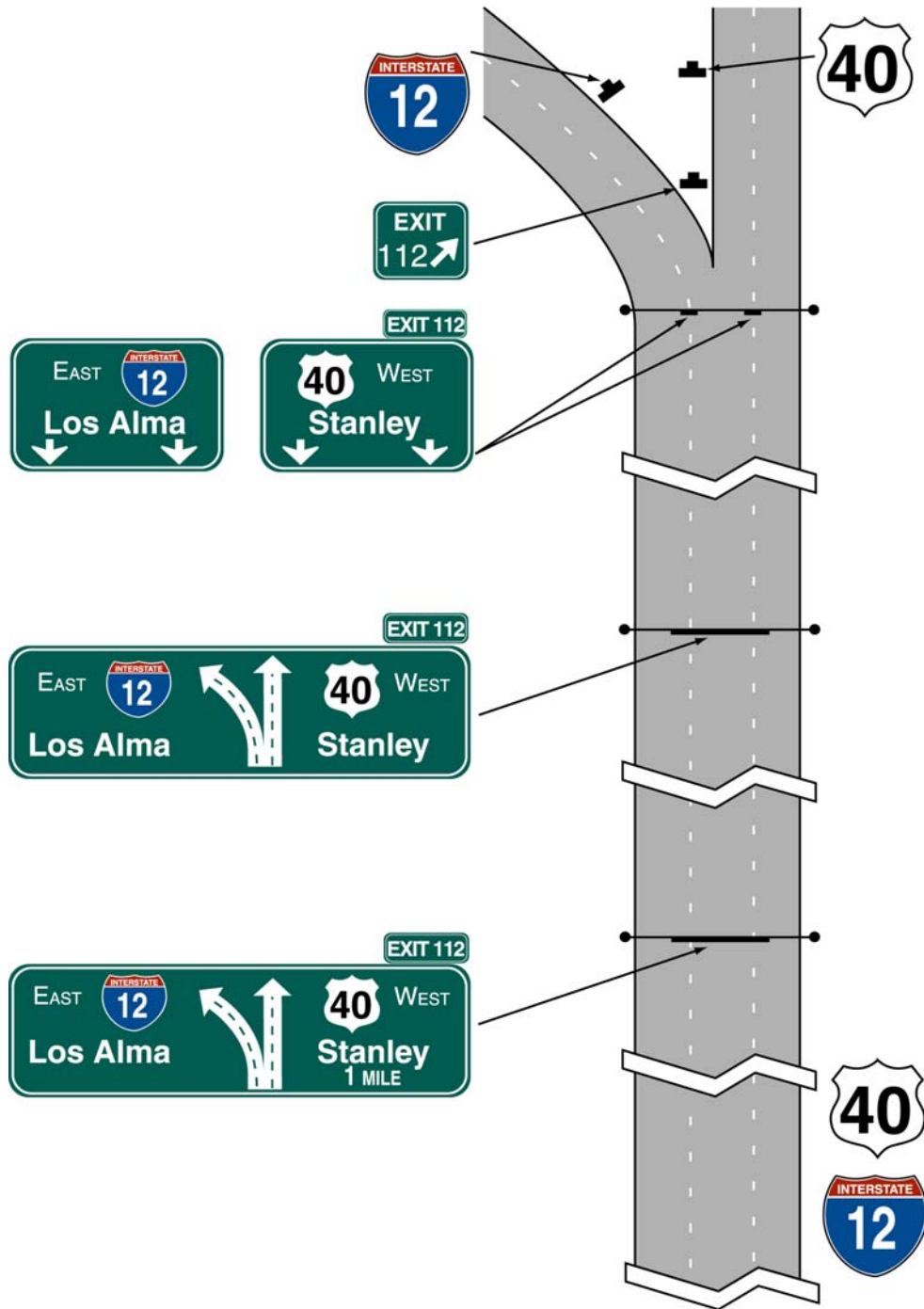
Figure 2E-6. Diagrammatic Signs for Two-Lane Exit with Optional Lane
