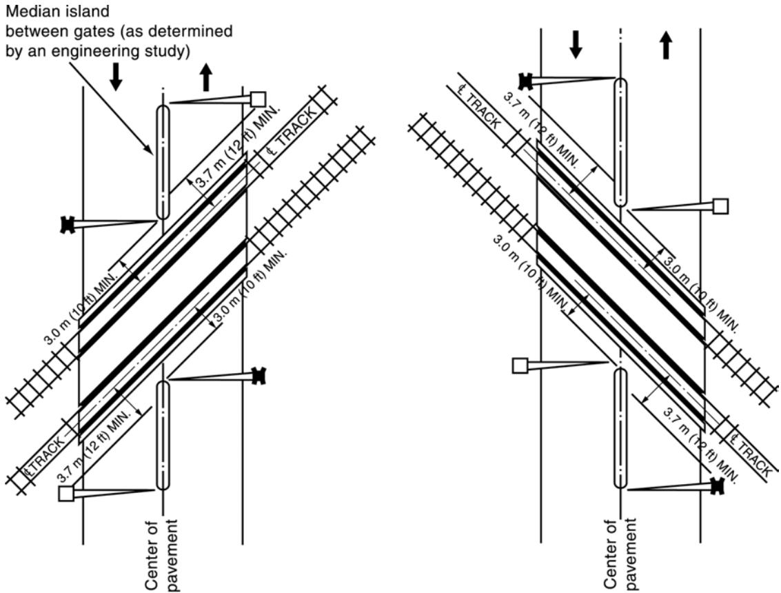
Figure 8D-2. Typical Location Plan for Flashing-Light Signals and Four-Quadrant Gates
