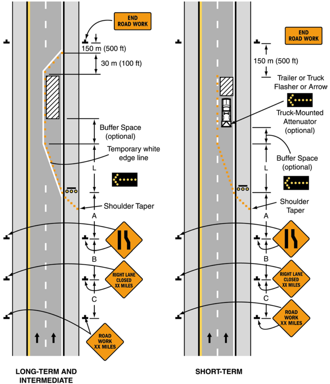
Figure 6H-33. Stationary Lane Closure on Divided Highway (TA-33)
