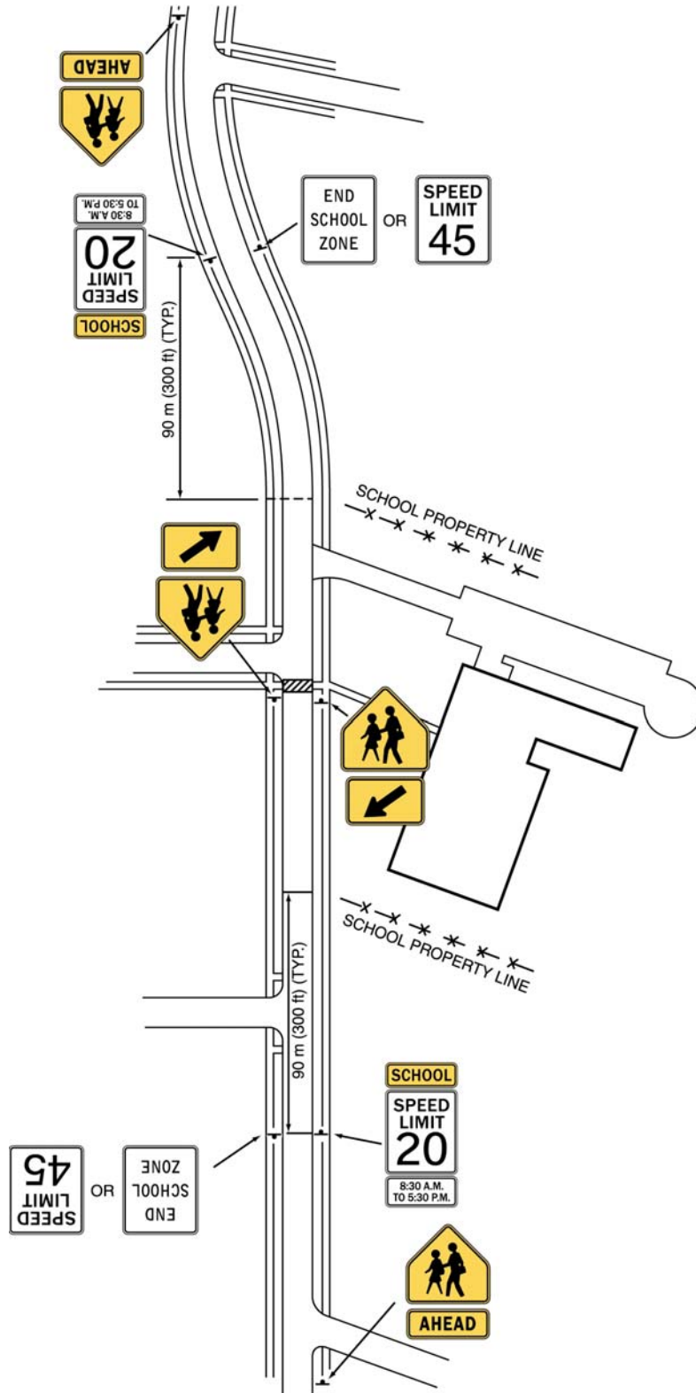
Figure 7B-1. Typical Signing for School Area Traffic Control
