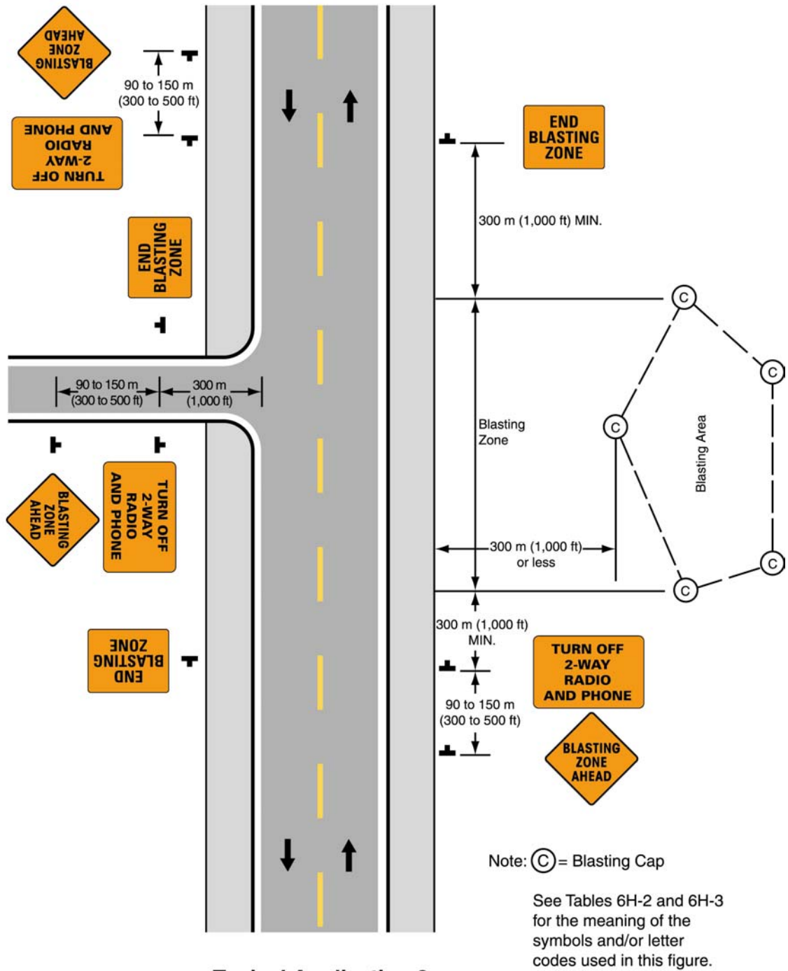
Typical Application 2
