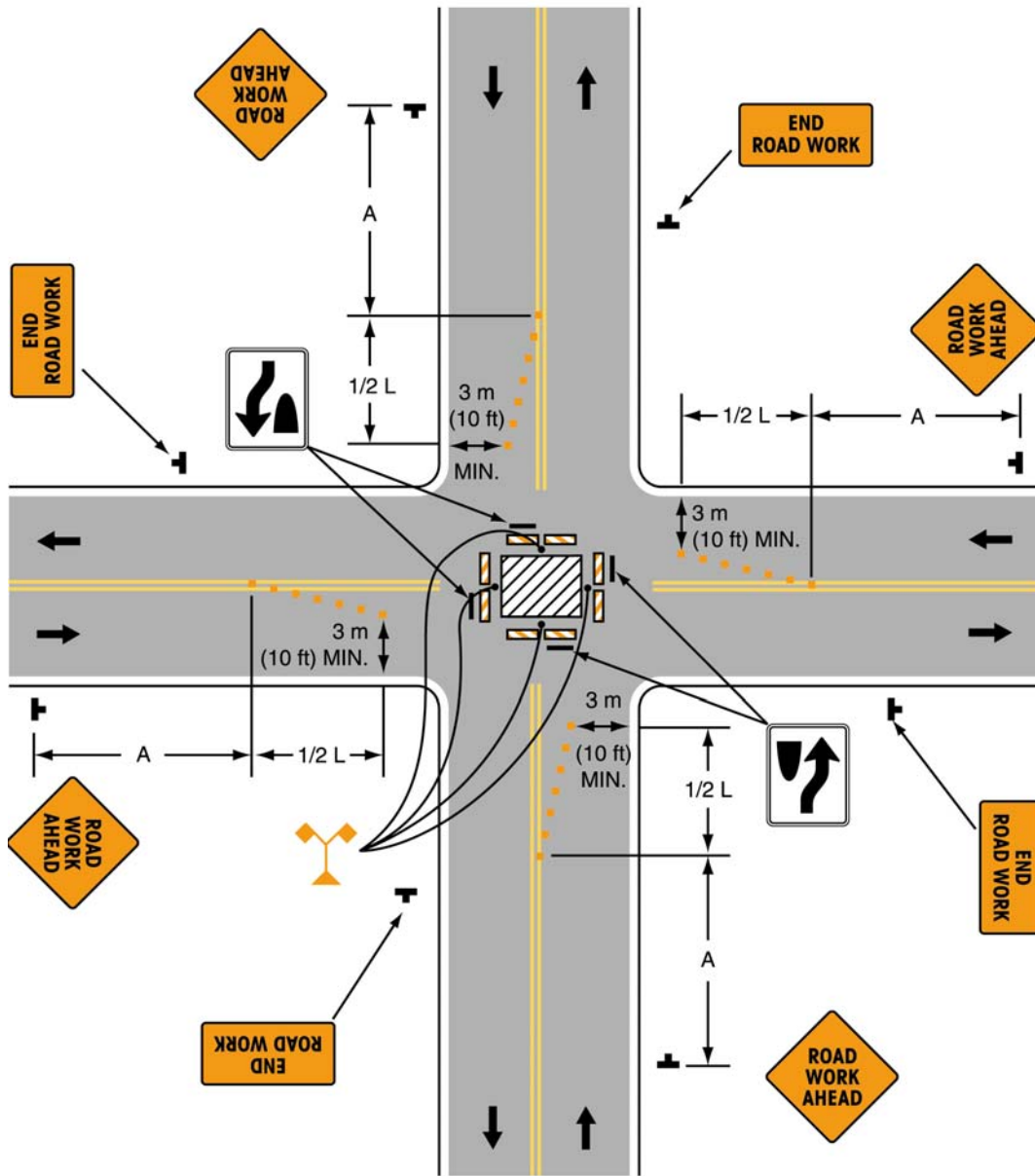
Typical Application 26
