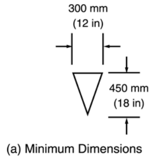
Figure 3B-14. Typical Yield Line Layout for Streets and Highways
