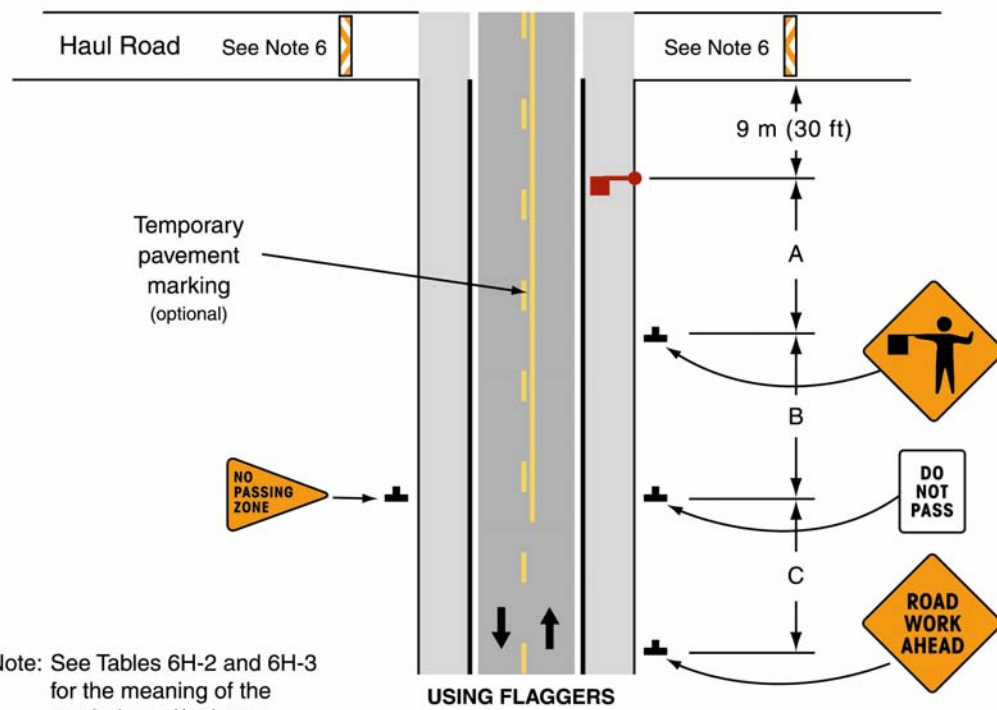
Typical Application 14
