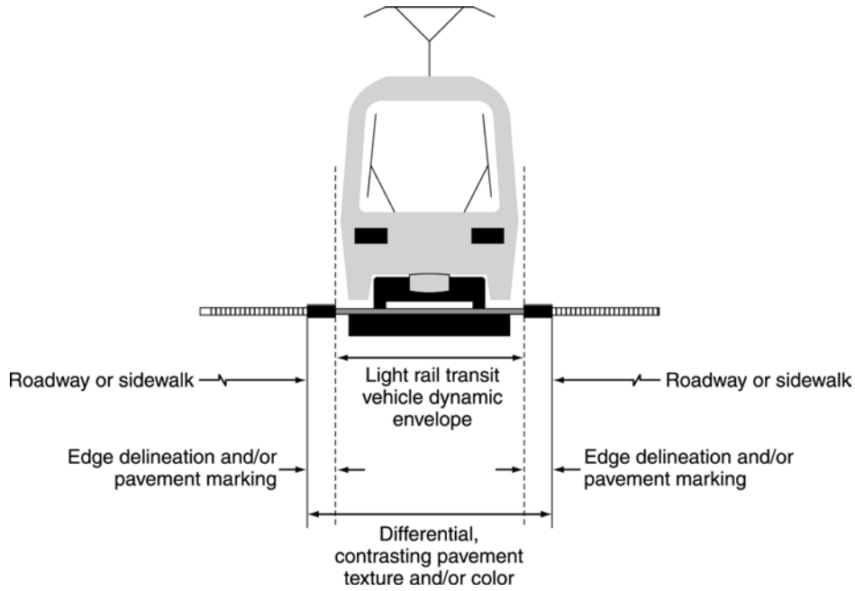
Figure 10C-2. Typical Light Rail Transit Vehicle Dynamic Envelope Delineation Pavement Markings
