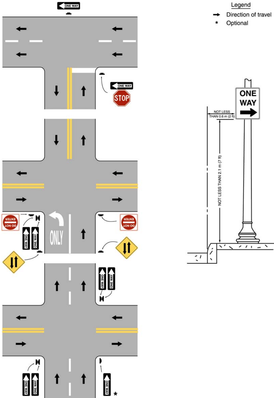
Figure 2A-6. Typical Locations of ONE WAY Signs
