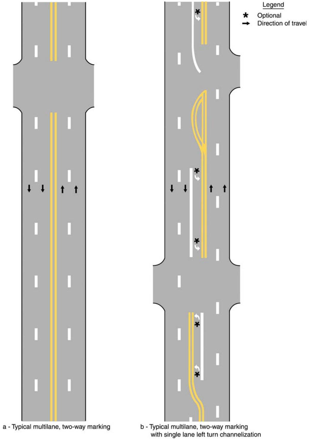
Figure 3B-2. Typical Four-or-More Lane, Two-Way Marking Applications
