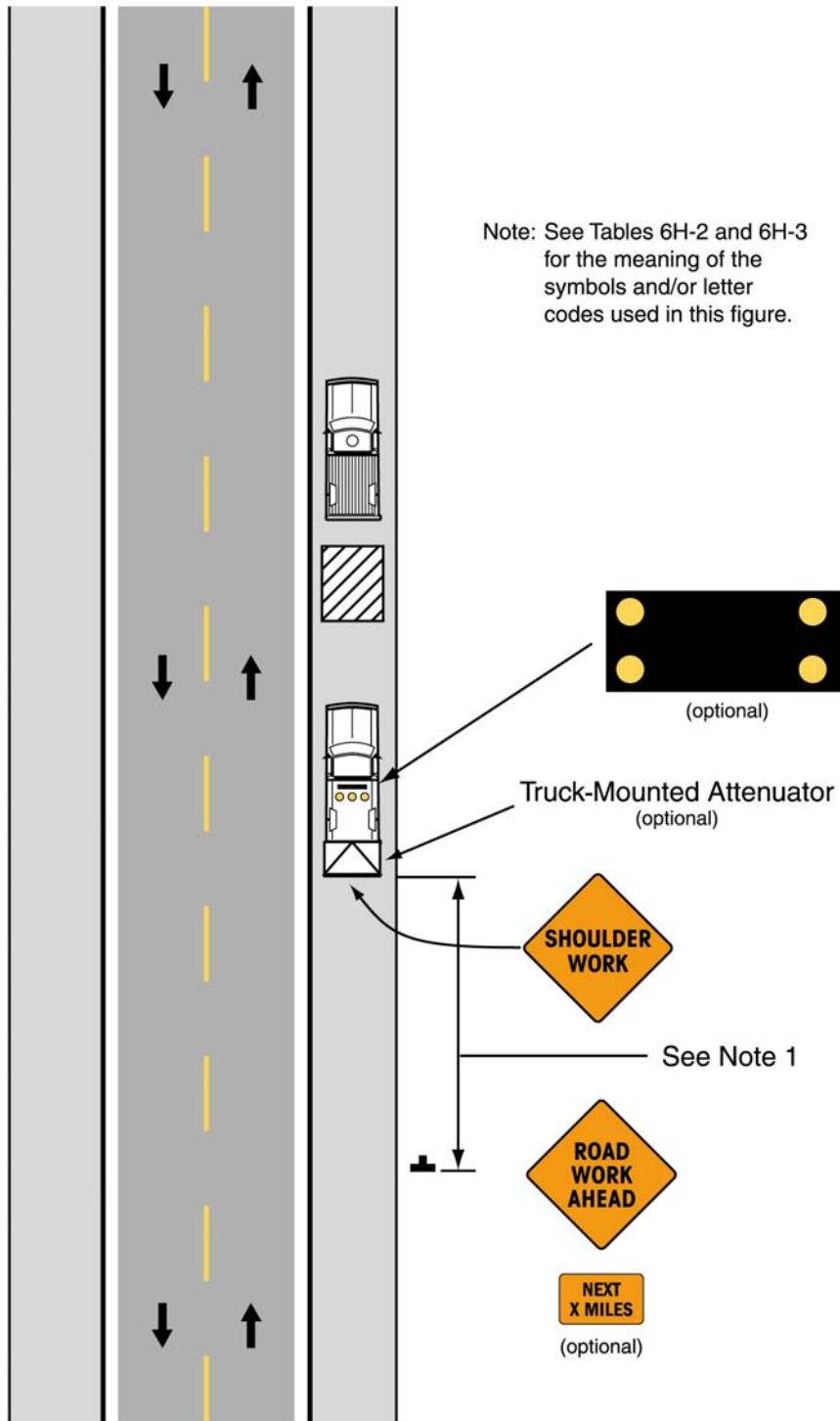
Typical Application 4
