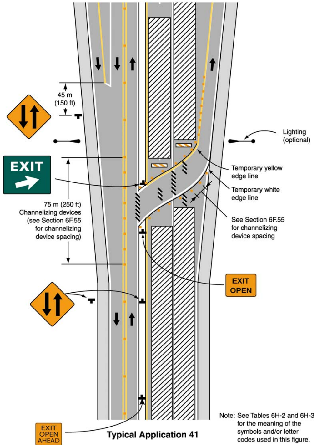
Figure 6H-41. Median Crossover for Exit Ramp (TA-41)
