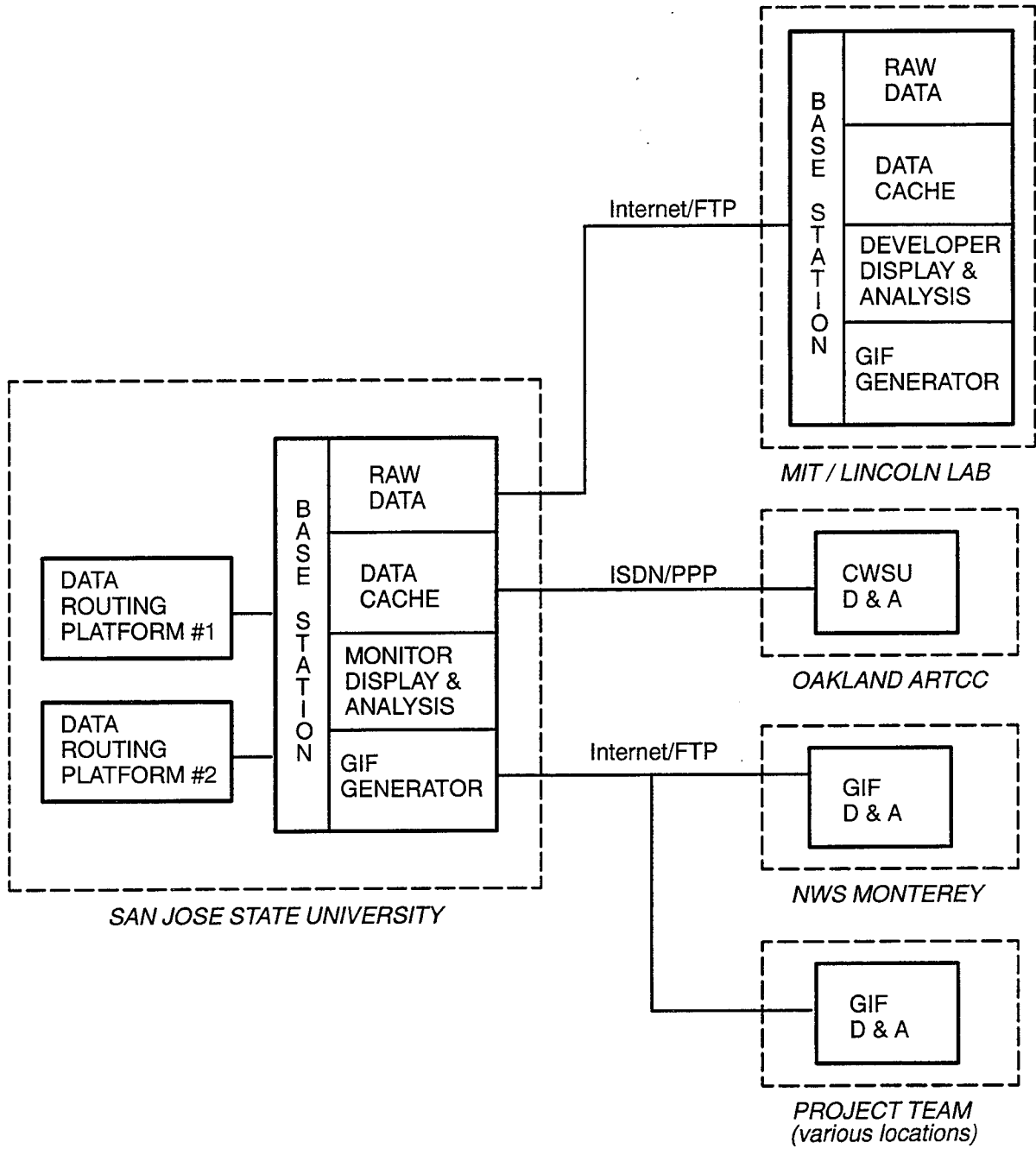
Figure 15. Current system configuration.
