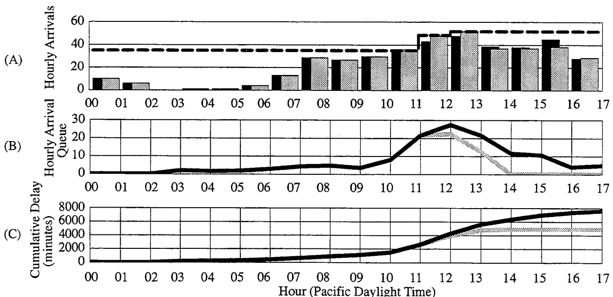
Figure 4. A) Hourly traffic count showing actual hourly arrivals (black) on 4 August 95, and adjusted hourly arrival assuming optimal use of available capacity (grey). Dashed line indicates optimal available capacity. B) Hourly arrival queue (number of planes) from model using actual (black) and adjusted hourly arrival counts. C) Hourly cumulative delay (minutes) from queuing model using actual (black) and adjusted (grey) hourly arrival counts.
