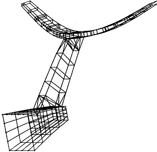
FIGURE 27. MODE 6 OF TAIL STRUCTURE ( f_n = 26.2 Hz)
