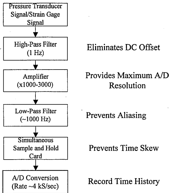
FIGURE 12. SCHEMATIC OF SIGNAL CONDITIONING AND RAW DATA RECORDING
