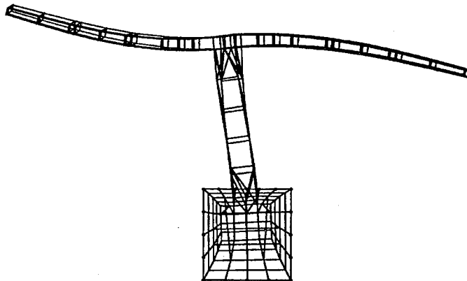
FIGURE 26. MODE 4 OF TAIL STRUCTURE ( f_n = 24.2 Hz)
