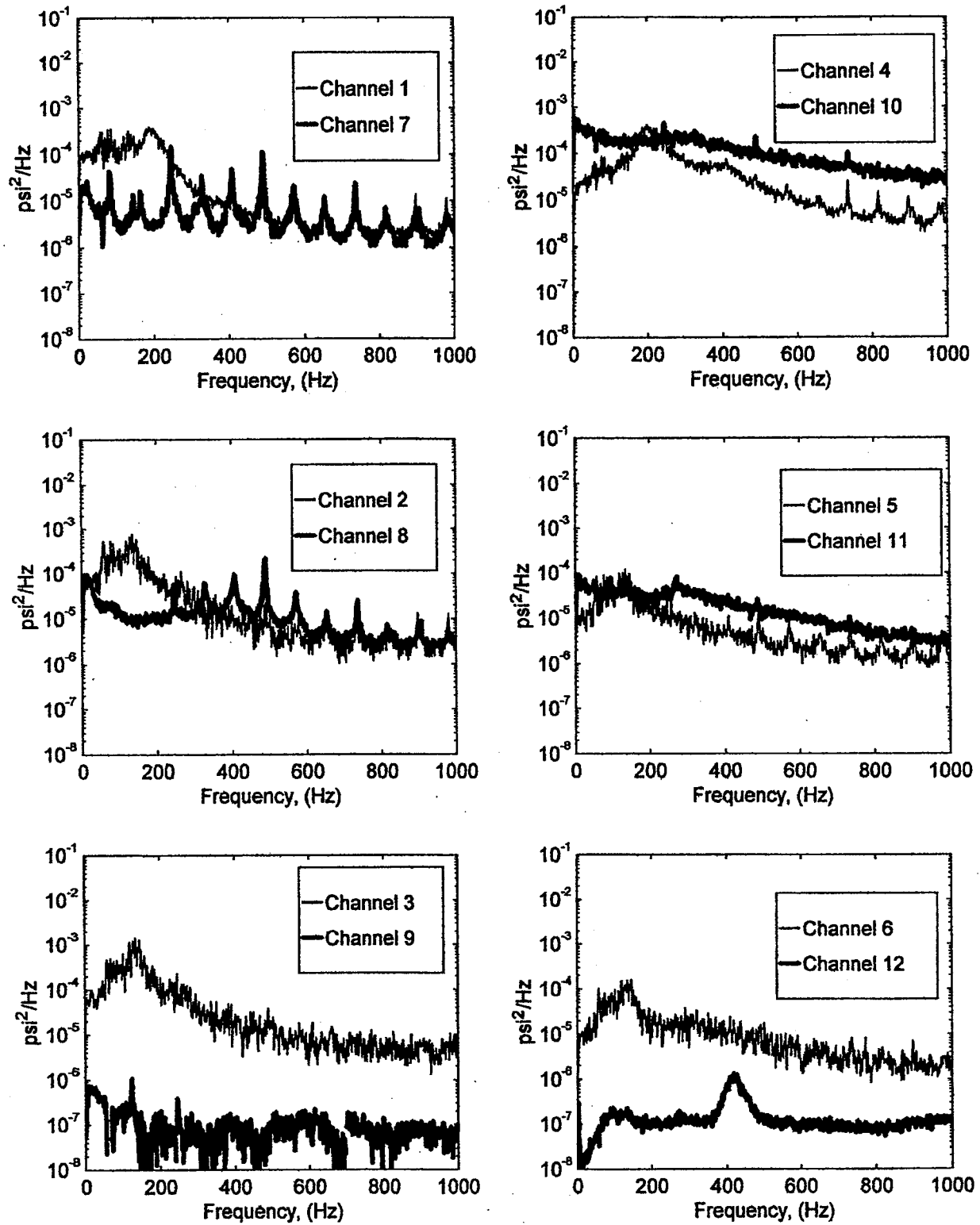
FIGURE B-22. PRESSURE POWER SPECTRAL DENSITY (RUN 8, POINT 4) (\bar{q} = 25 \text{ psf}, \alpha = 10^\circ, \psi = -10^\circ)
