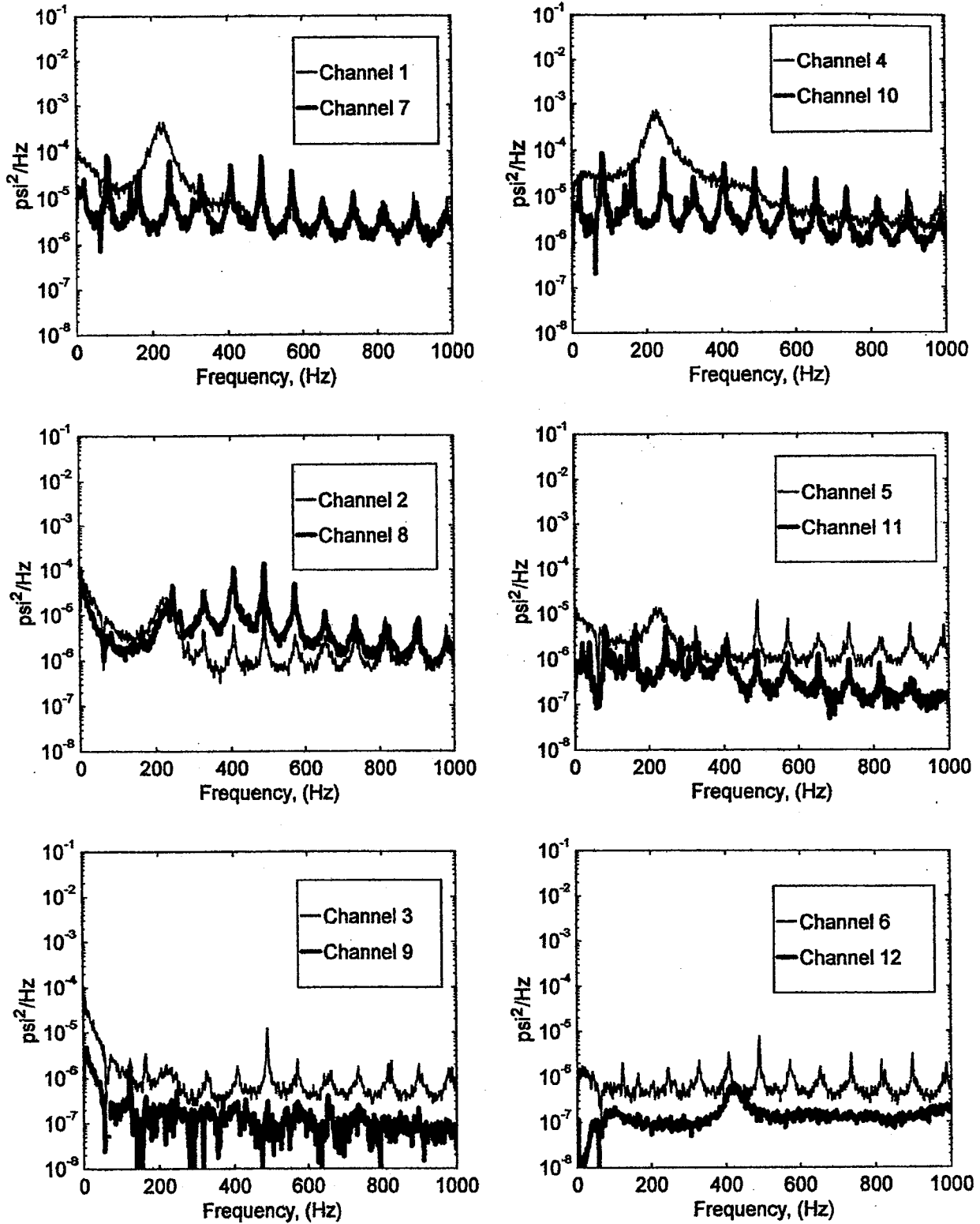
FIGURE B-20. PRESSURE POWER SPECTRAL DENSITY (RUN 8, POINT 2) (\bar{q} = 25 \text{ psf}, \alpha = 0^\circ, \psi = -10^\circ)
