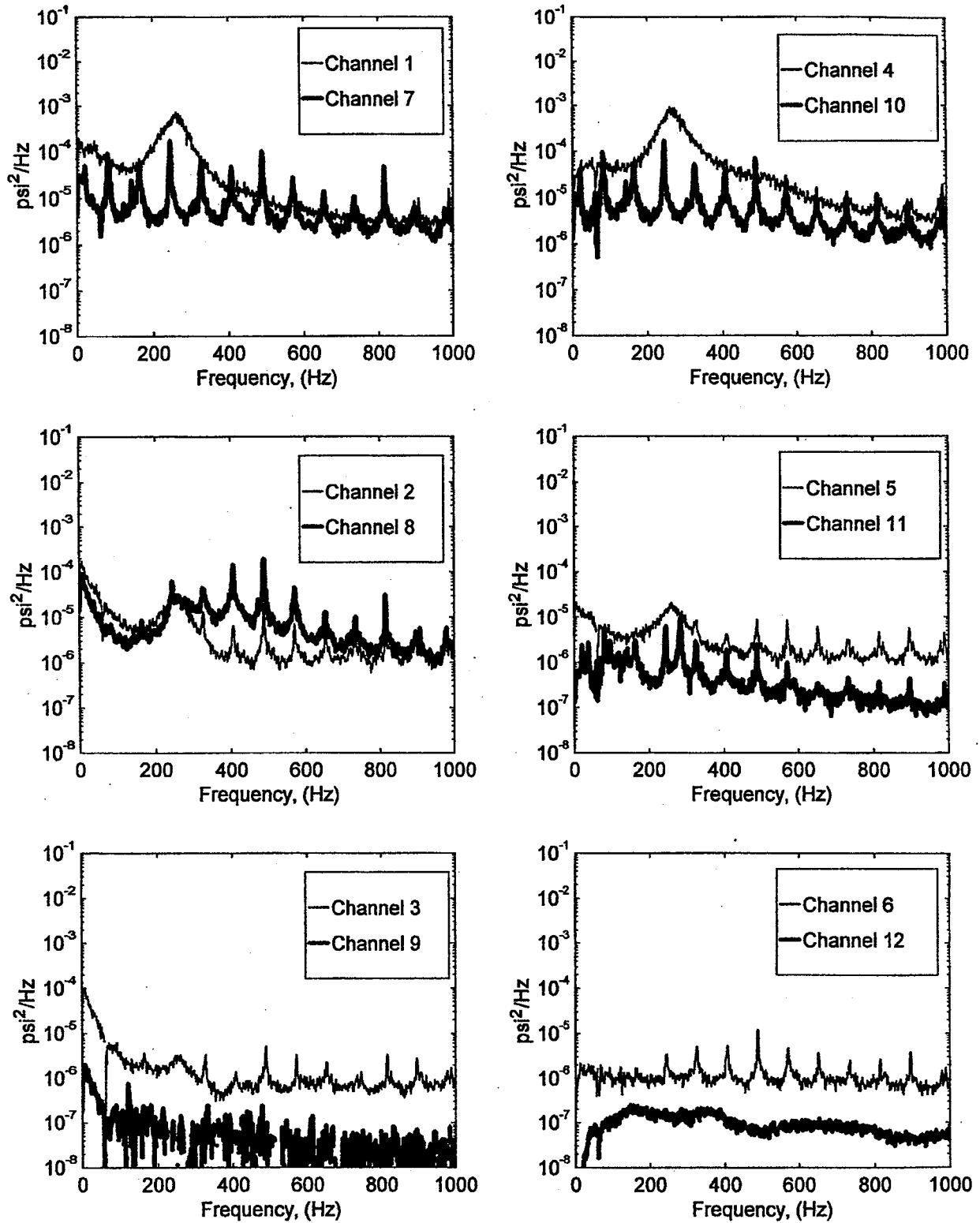
FIGURE B-26. PRESSURE POWER SPECTRAL DENSITY (RUN 9, POINT 2) (\bar{q} = 35 \text{ psf}, \alpha = 0^\circ, \psi = -10^\circ)
