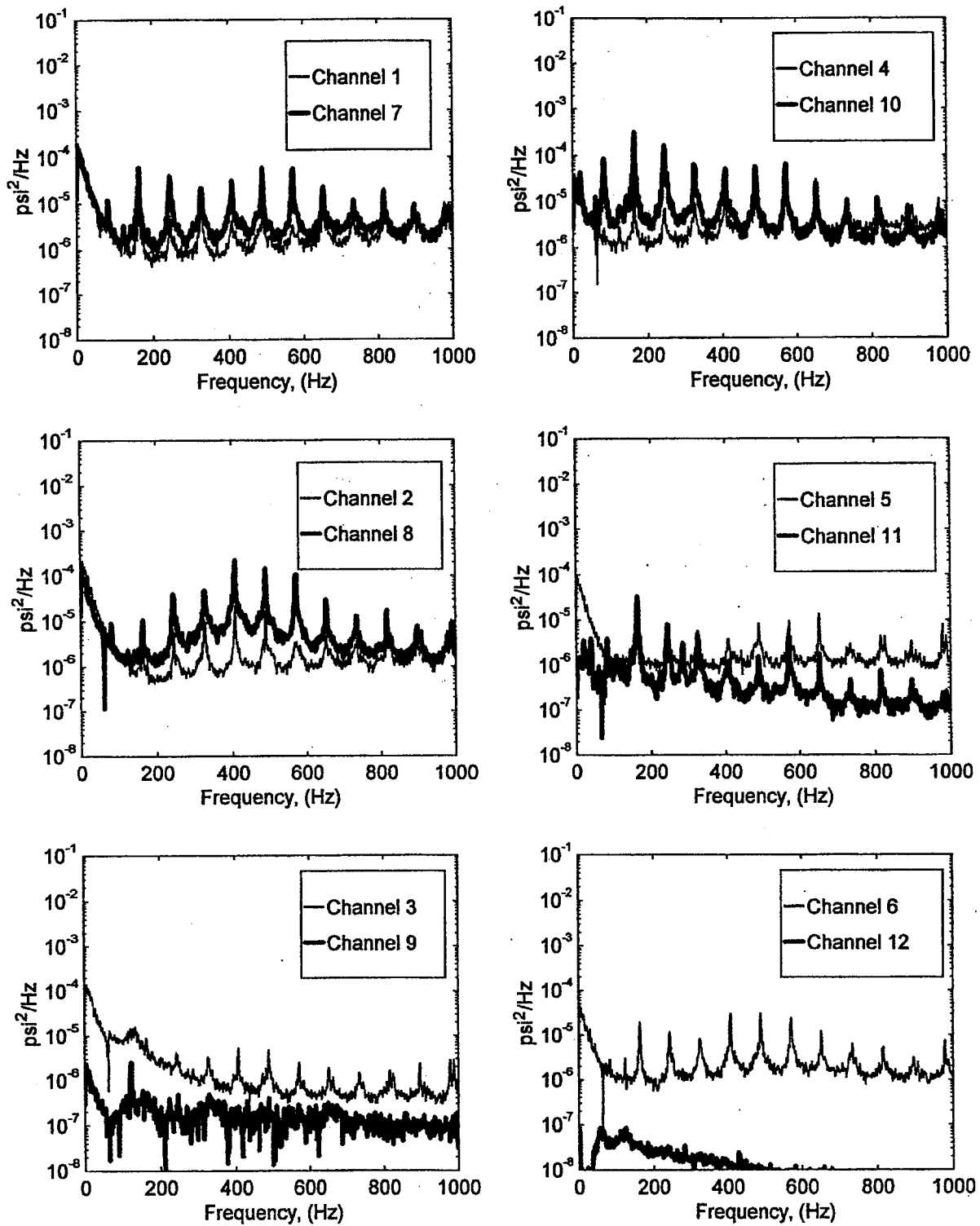
FIGURE B-8. PRESSURE POWER SPECTRAL DENSITY (RUN 6, POINT 2) (\bar{q} = 35 \text{ psf}, \alpha = 0^\circ, \psi = 0^\circ)
