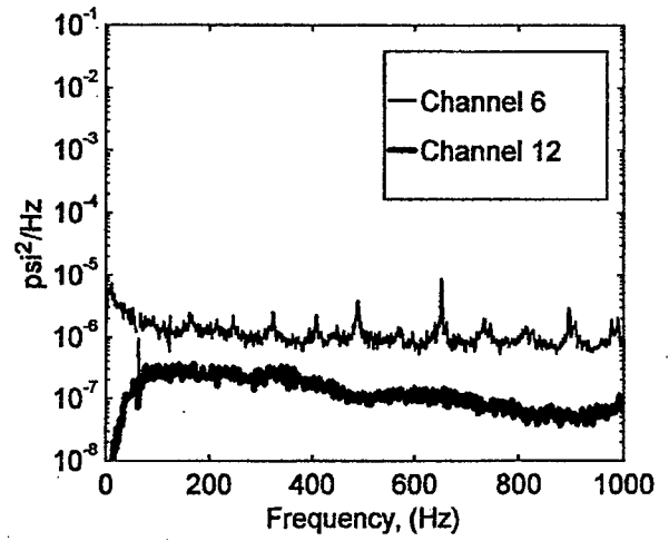
FIGURE B-27. PRESSURE POWER SPECTRAL DENSITY (RUN 9, POINT 3) (\bar{q} = 35 \text{ psf}, \alpha = 5^\circ, \psi = -10^\circ)
