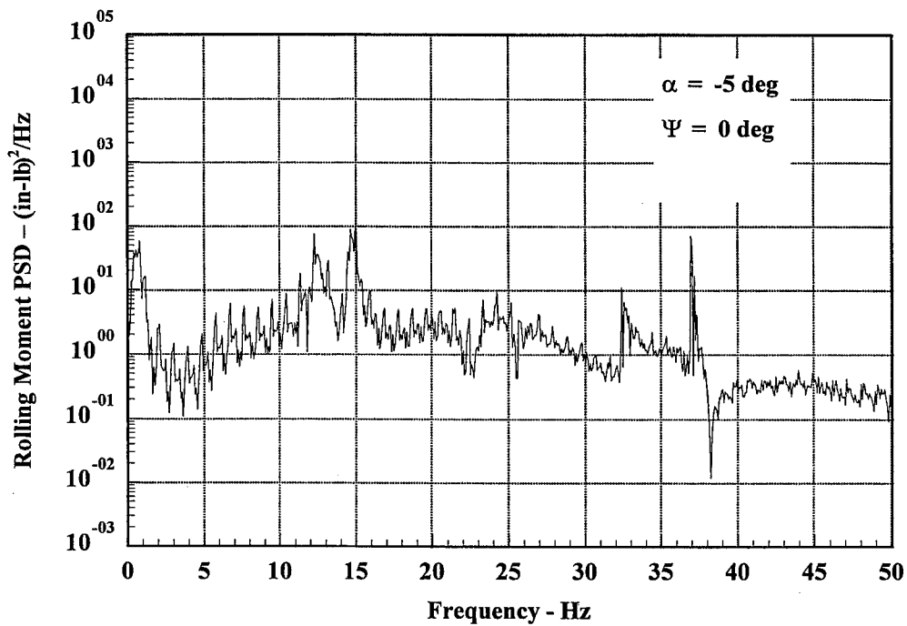
FIGURE 29a. POWER SPECTRAL DENSITY OF PREDICTED ROLLING MOMENT (Q = 25 psf)
