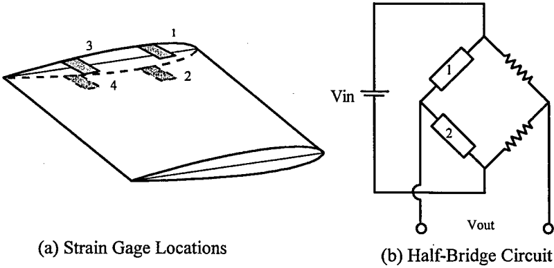
FIGURE 11. STRAIN GAGE LOCATIONS AND CIRCUITRY
