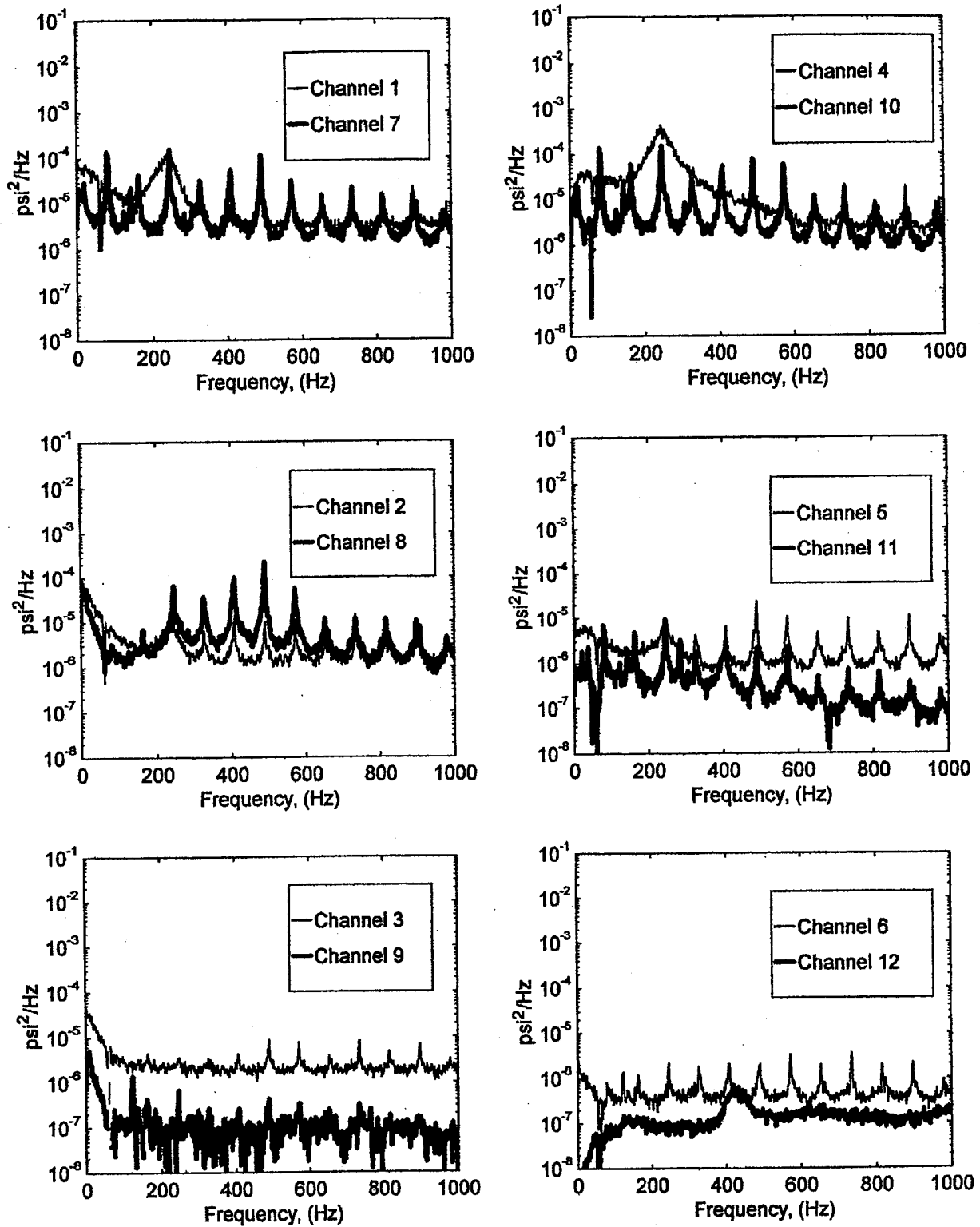
FIGURE B-19. PRESSURE POWER SPECTRAL DENSITY (RUN 8, POINT 1) (\bar{q} = 25 \text{ psf}, \alpha = -5^\circ, \psi = -10^\circ)
