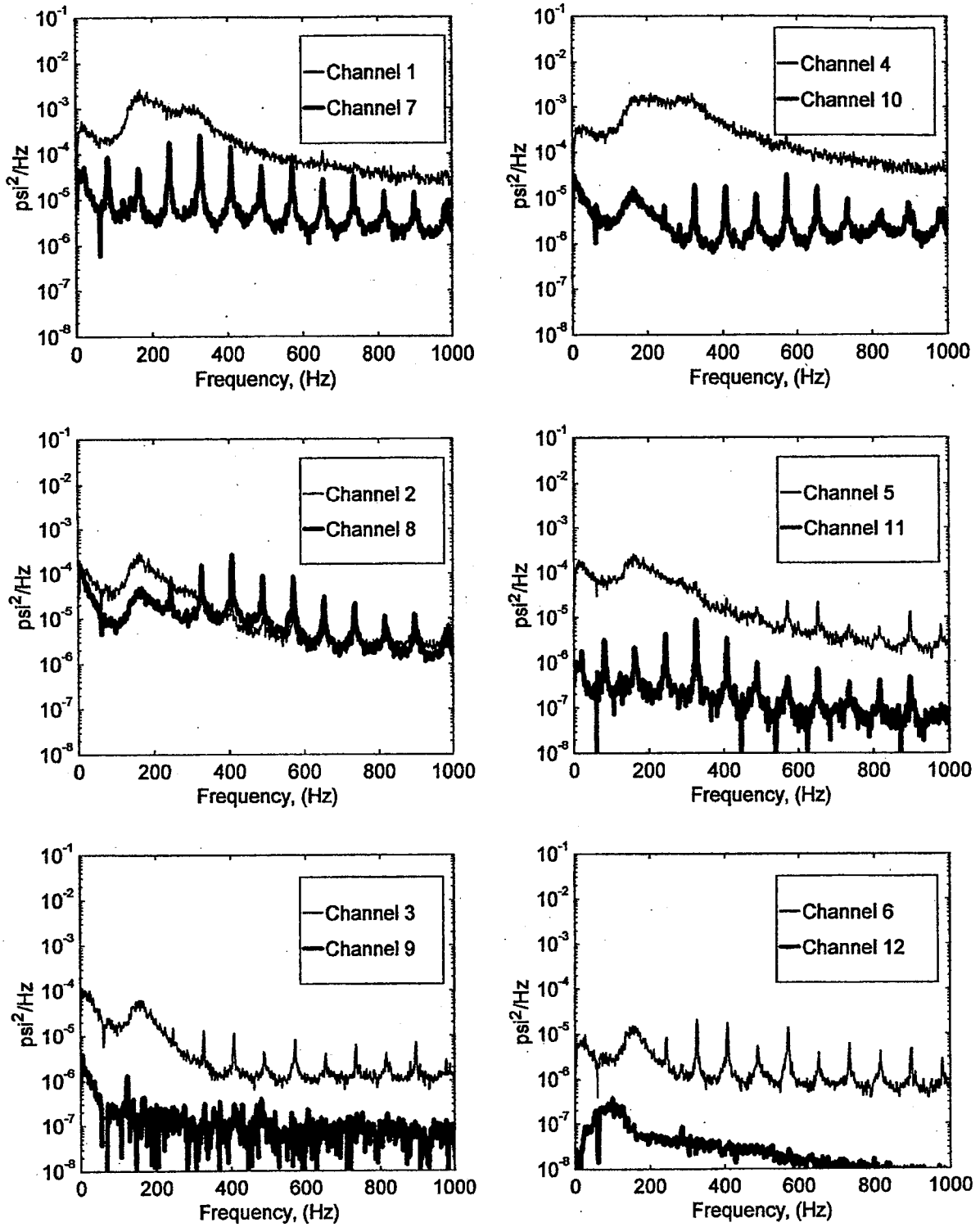
FIGURE B-43. PRESSURE POWER SPECTRAL DENSITY (RUN 12, POINT 1) (\bar{q} = 35 \text{ psf}, \alpha = -5^\circ, \psi = -20^\circ)
