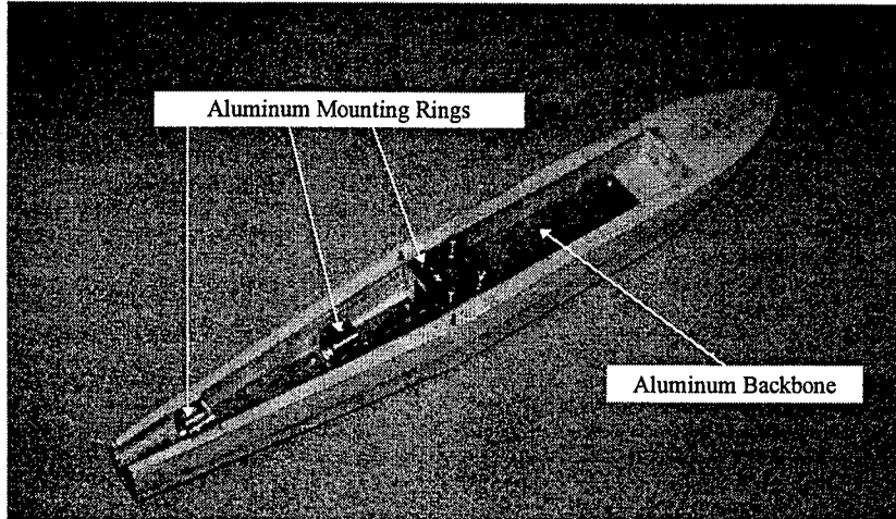
FIGURE 5. TOP OF FUSELAGE WITH STING MOUNT/ALUMINUM BACKBONE
