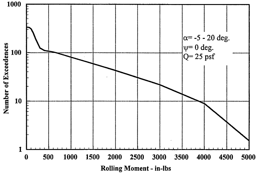
FIGURE 31, PREDICTION OF NUMBER OF EXCEEDENCES FOR A GIVEN STALL EVENT
