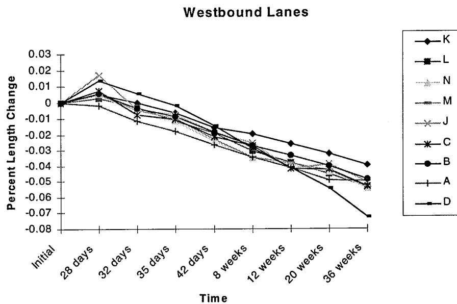
Figure 4.1 Graph of length change versus age of concrete
