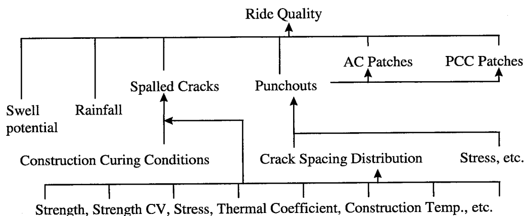
Figure 6.3 Interactions between different condition variables for CRCP
