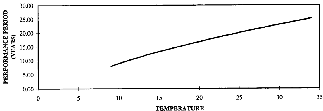
PERFORMANCE PERIOD VS. TEMPERATURE
