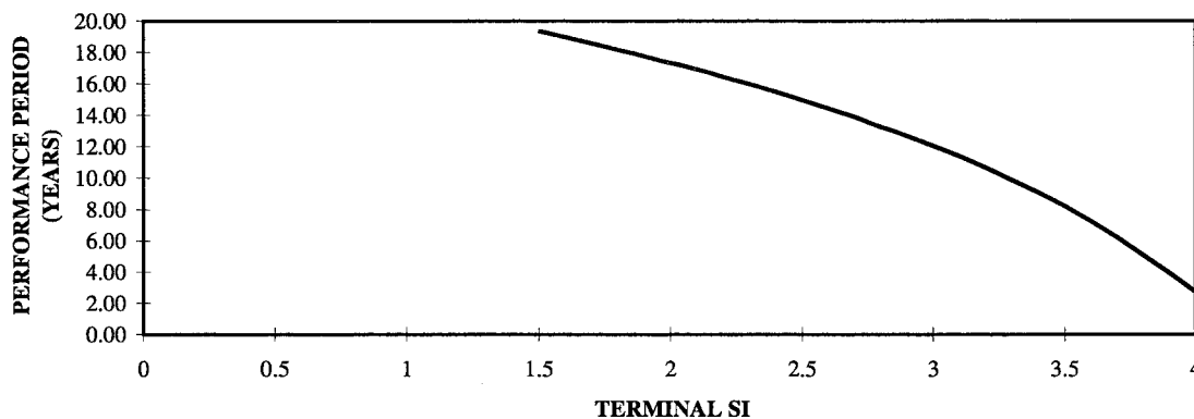
PERFORMANCE PERIOD VS. TERMINAL SI
