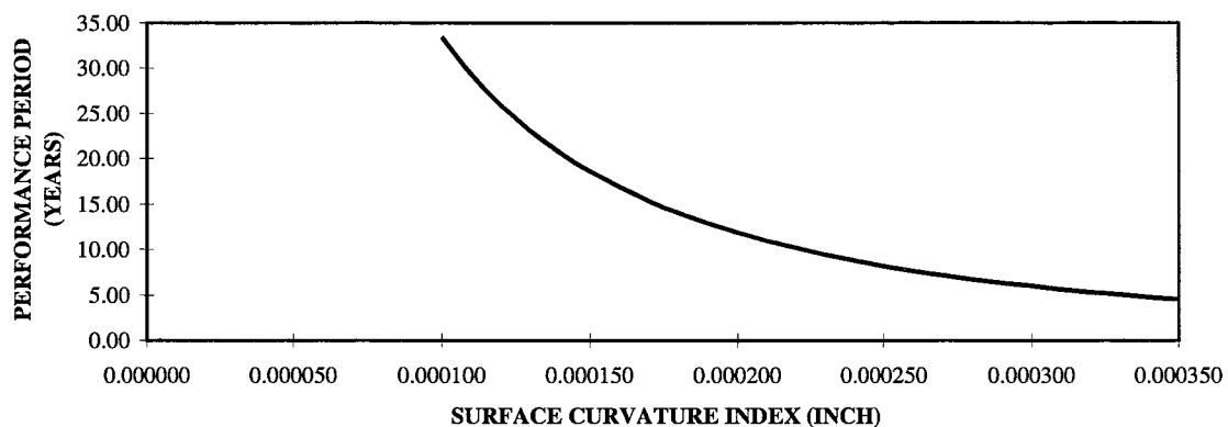
PERFORMANCE PERIOD VS. SURFACE CURVATURE INDEX
