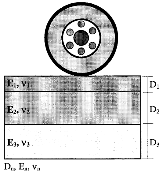
Figure 3.2 Typical three-layer elastic mode
