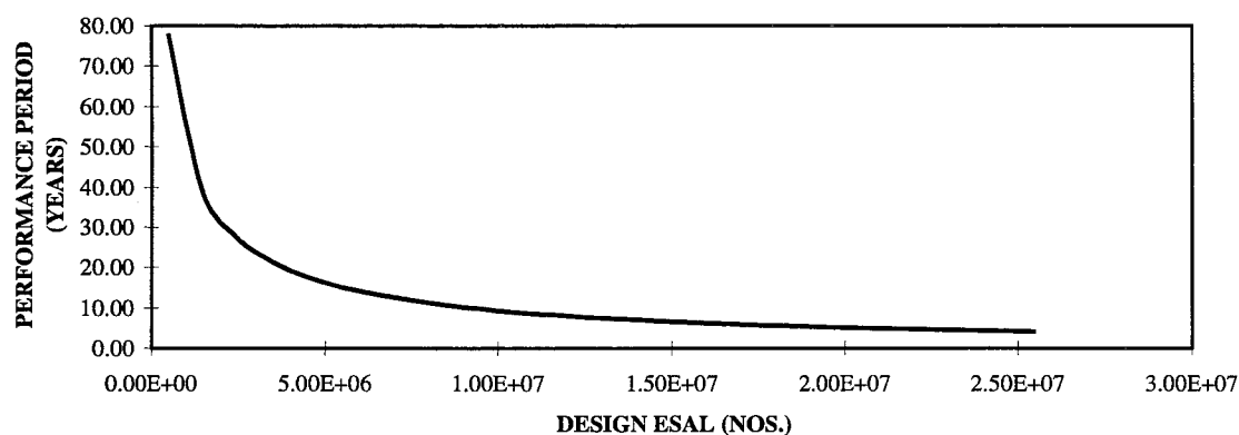
PERFORMANCE PERIOD VS. DESIGN ESAL
