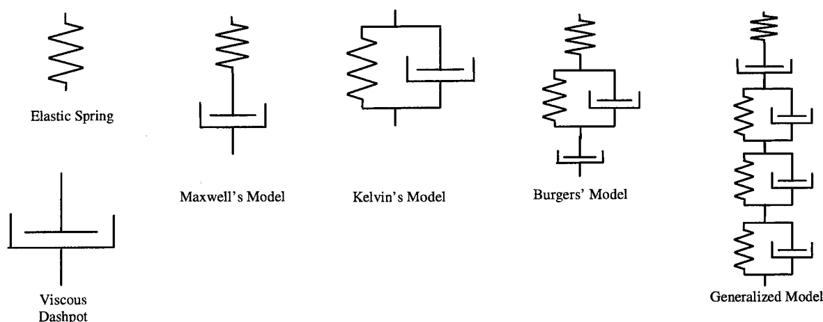
Figure 3.3 Typical visco-elastic models
