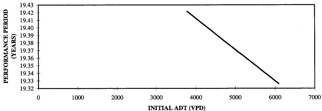
PERFORMANCE PERIOD VS. INITIAL ADT
