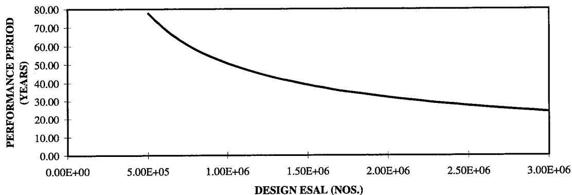
PERFORMANCE PERIOD VS. DESIGN ESAL
