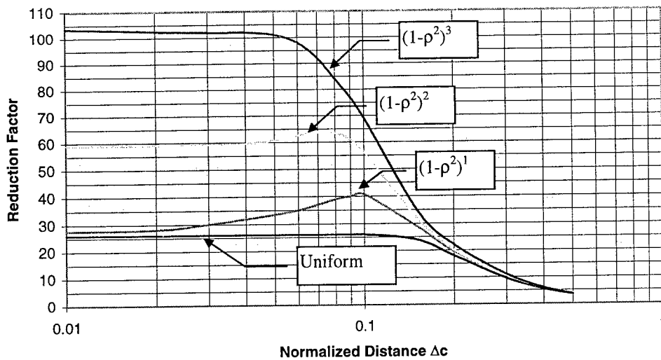
FIGURE 4 NEAR-FIELD CORRECTION FACTORS FOR CIRCULAR APERTURES
