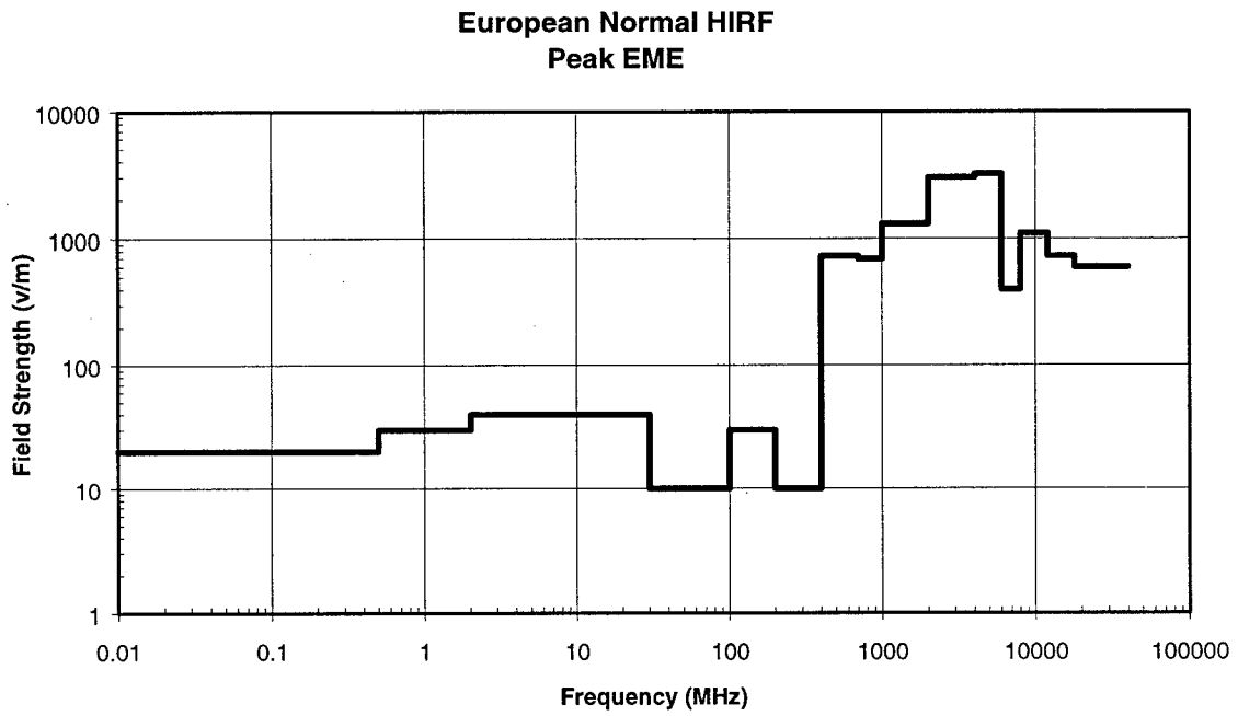
FIGURE 23 PEAK EUROPEAN NORMAL ENVIRONMENT
