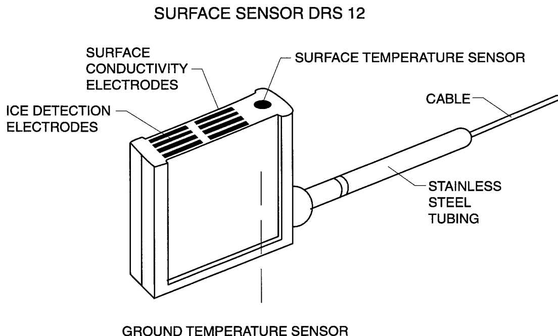
Figure 3.1 DRS 12 Road Surface Sensor
