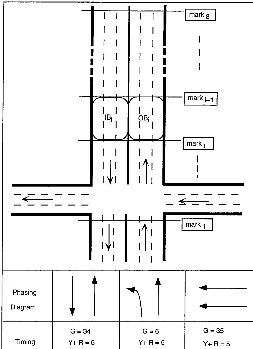
Figure 5.1. Geometry diagram at the signalized intersection
