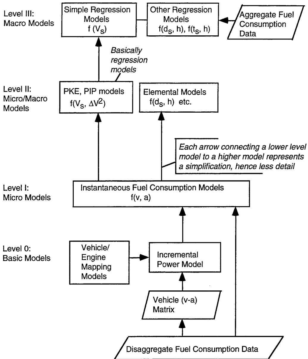
Figure 2.1 Hierarchy of vehicle fuel consumption models
