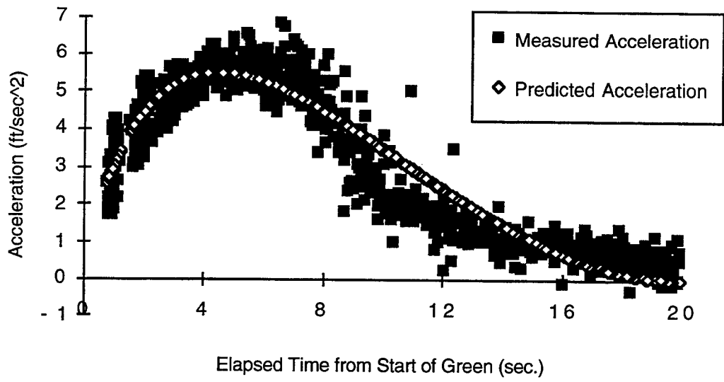
Figure 5.4. Measured and predicted vehicle acceleration trajectories
