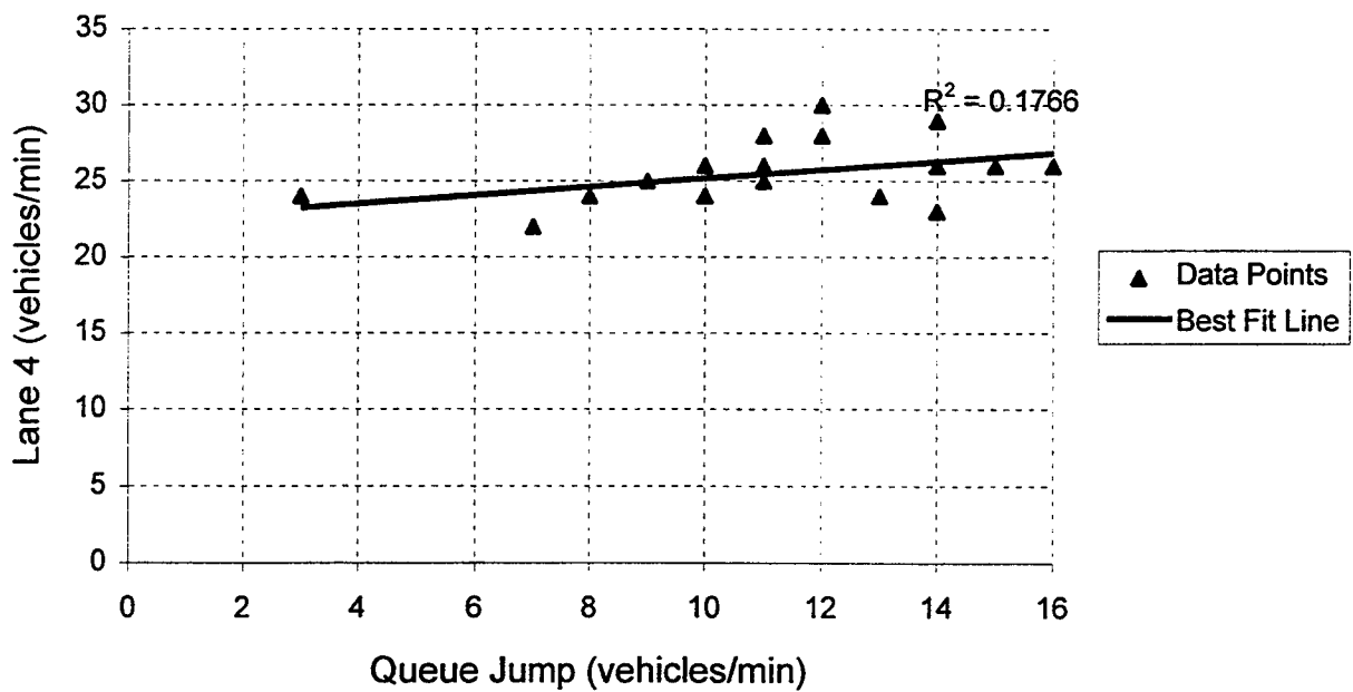
Figure 6. Queue Jump Analysis - WB LBJ IH635 Lane Closures
