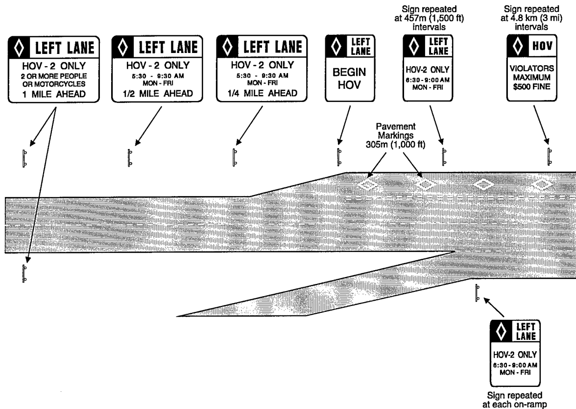
Figure 28. Standard HOV Signing Layout
