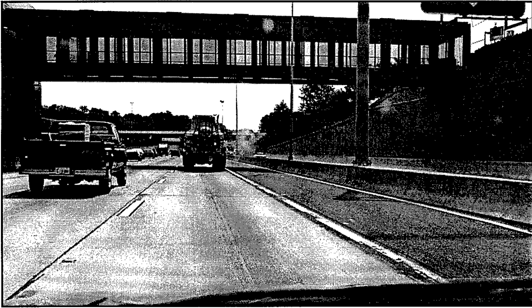
Figure 10. Shoulder Lane Pavement Configuration on I-66
