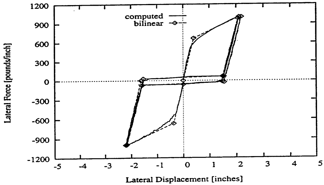
Figure 3. A typical p - y curve for the near-field spring, shown as lateral force per length of pile (pounds/inch) versus displacement (inches).
