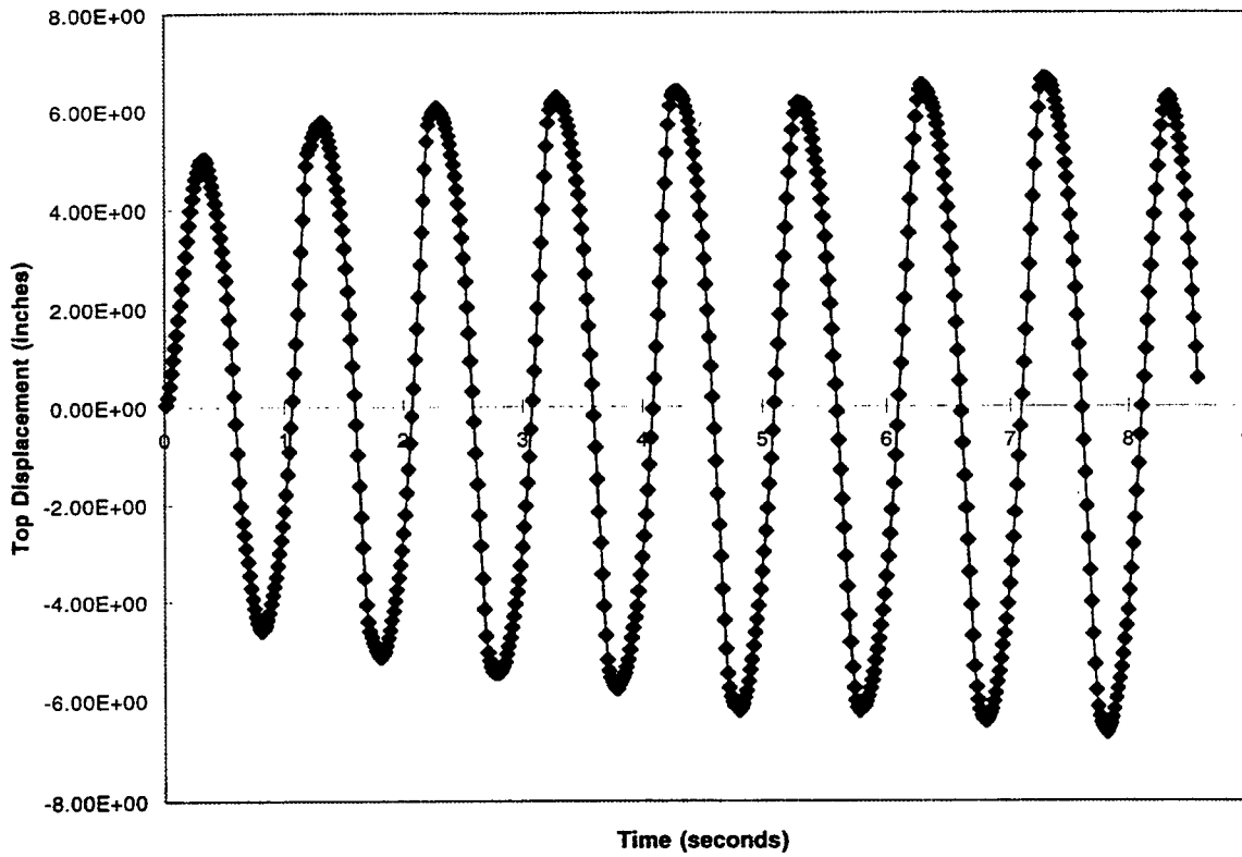
Figure 18. Pile Head Response, 100 Kip Lateral Load at 1 hz
