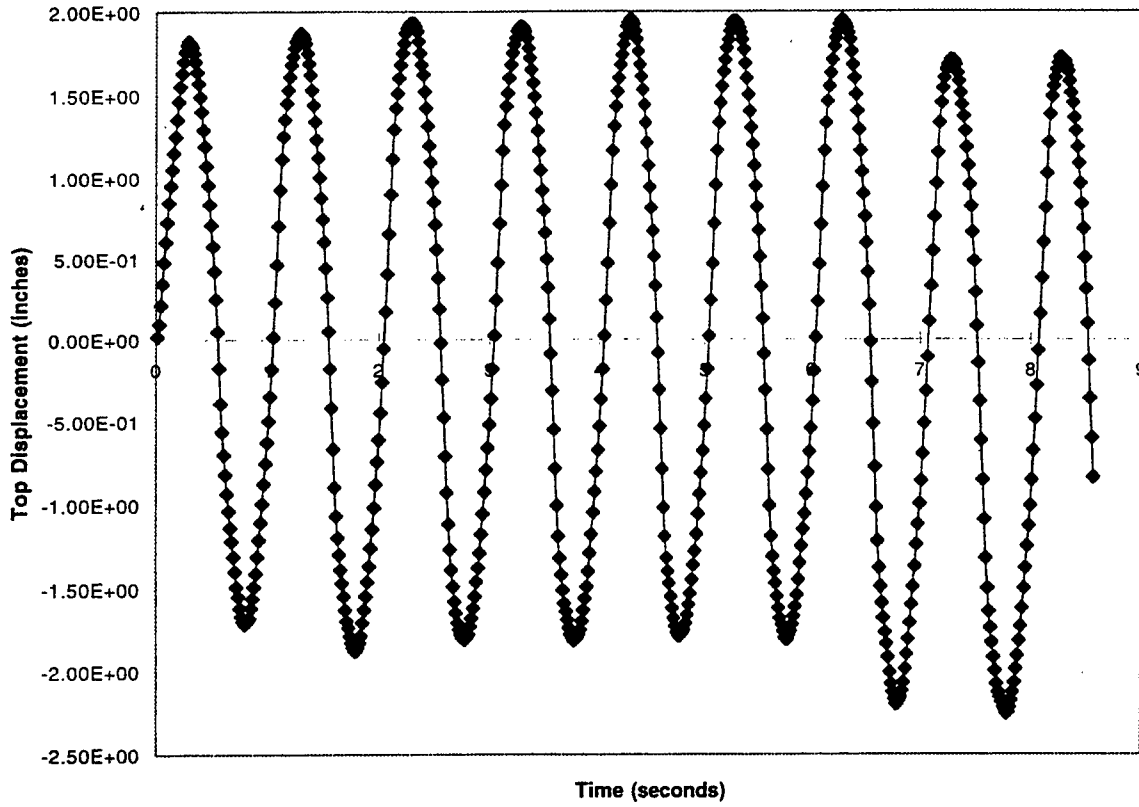
Figure 16. Pile Head Response, 50 Kip Lateral Load at 1 hz
