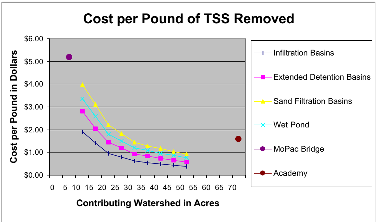
Figure 33. Cost per Pound of TSS Removed: Partial Concrete Construction.
