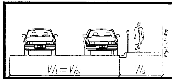
FIGURE 5 Lateral separation with on-street parking.
