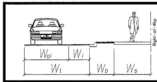
FIGURE 4 Buffers and sidewalk.
