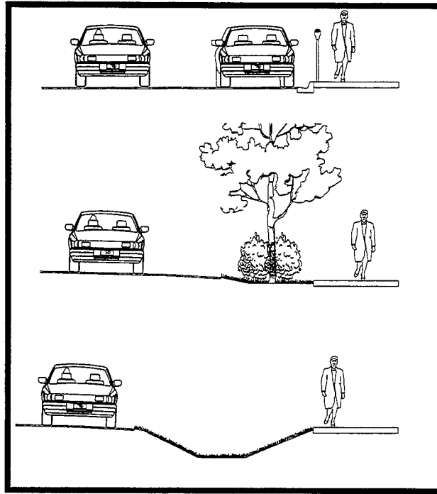
FIGURE 3 Typical barriers within the roadside buffer.
