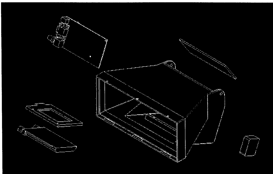
Figure 3. Breadboard Prototype HUD Demonstrated at NHTSA
