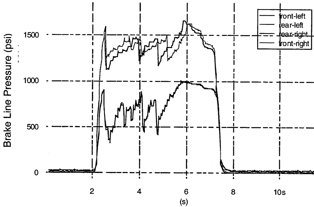
Figure 3–9. Brake line pressures, ABS, high- \mu , simulated, 1994 Ford Taurus
