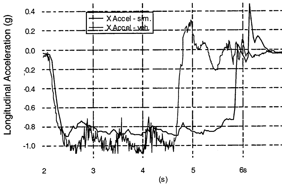
Figure 3–8. Comparison of ABS deceleration of 1997 Concorde and simulated 1994 Taurus
