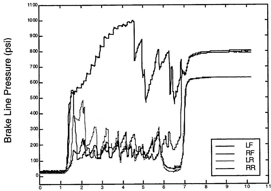
Figure 3-2. Bench test 0.5 g split- \mu stop
