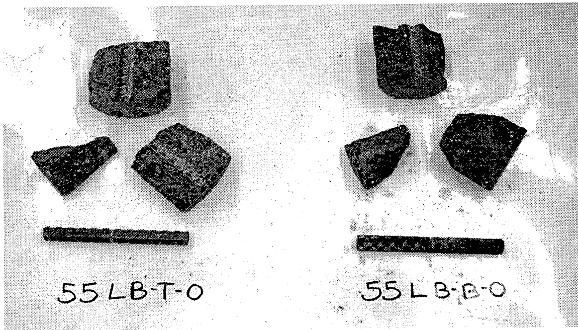
Figure 7. Tensile Bond Pullout Strength Specimens After Testing. Left, epoxy-coated bar; right, black bar.
