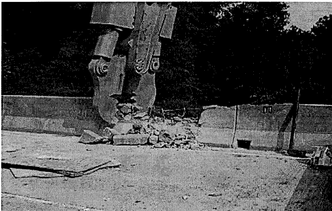
Figure 6. Concrete Removed Using Concrete Crusher
