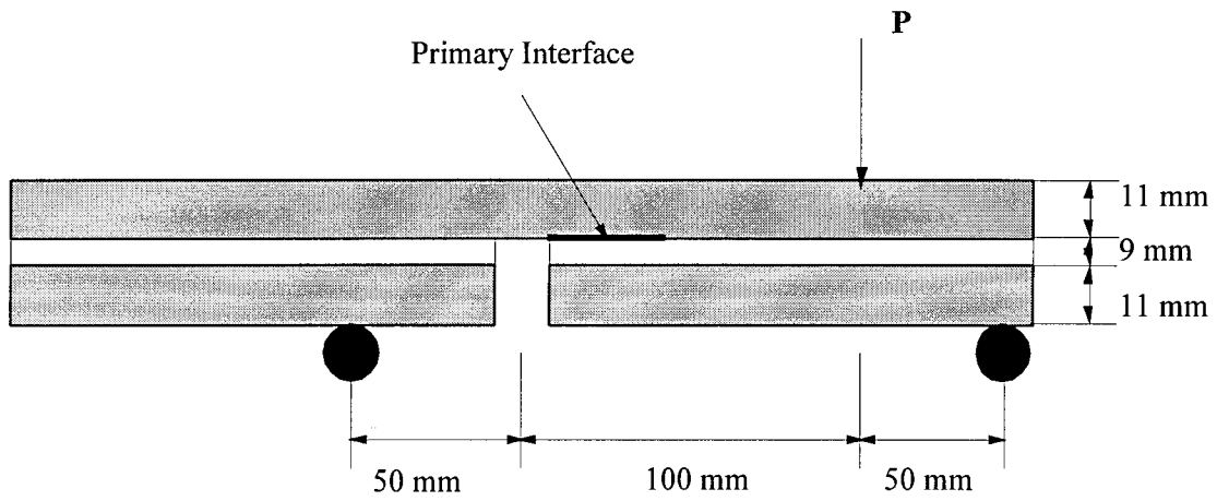
Figure 3: Modified Mixed Mode Flexure Test Geometry
