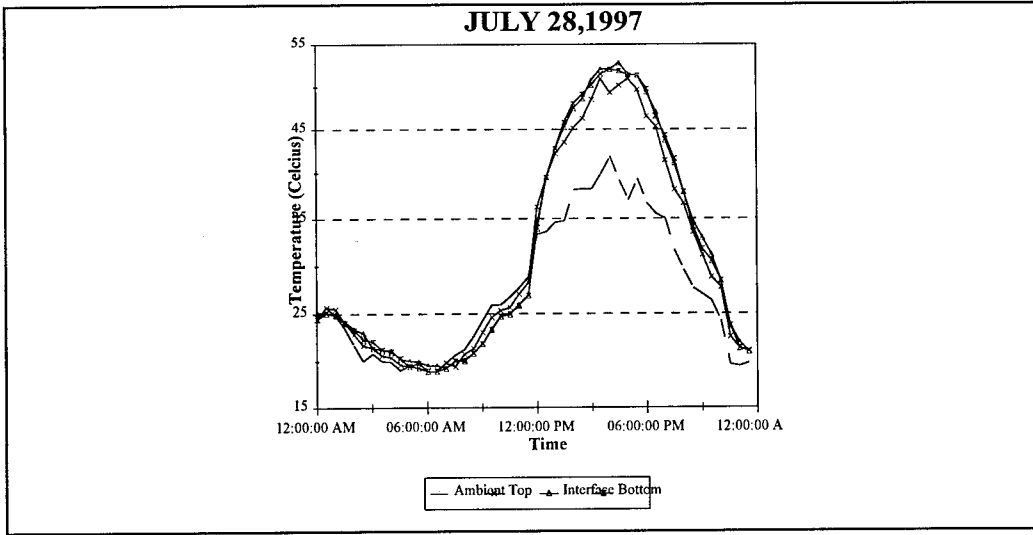
Figure 4: Maximum Temperature of Outdoor Specimen
