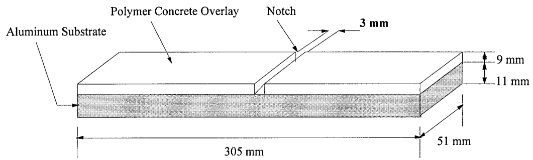
Figure 1: Specimen Dimensions
