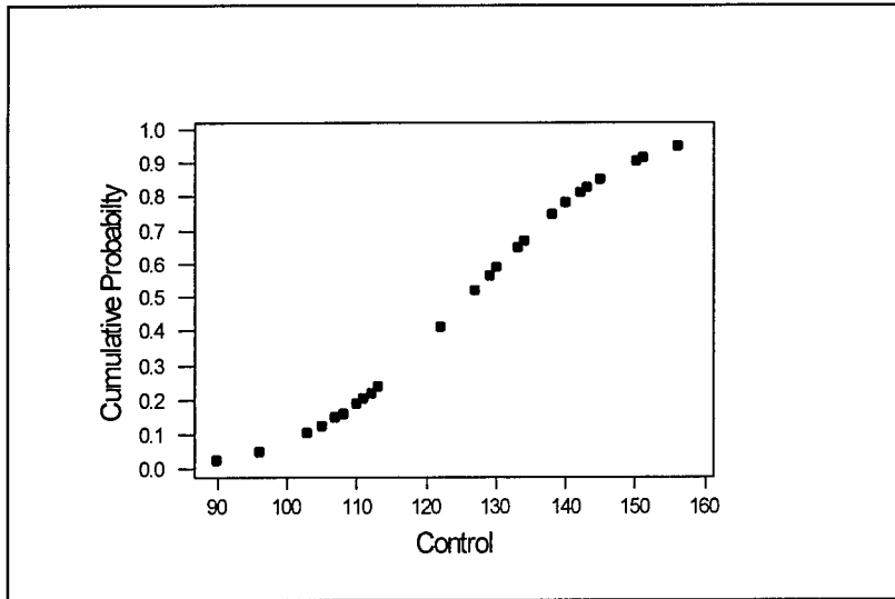
Figure 7: Cumulative Probability of Control Group
