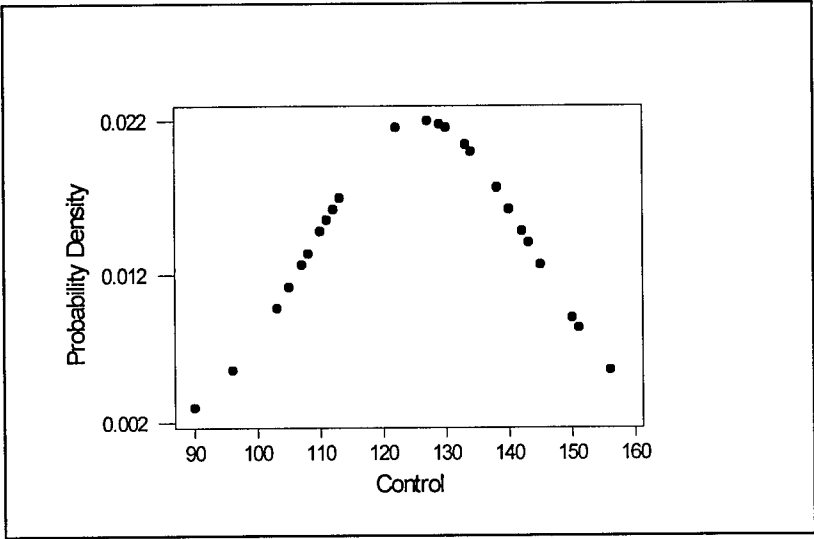
Figure 6: Probability Density of Control Group
