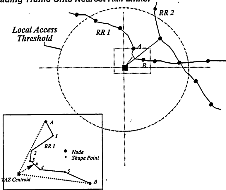
(A) Loading Traffic Onto Nearest Rail Links.
