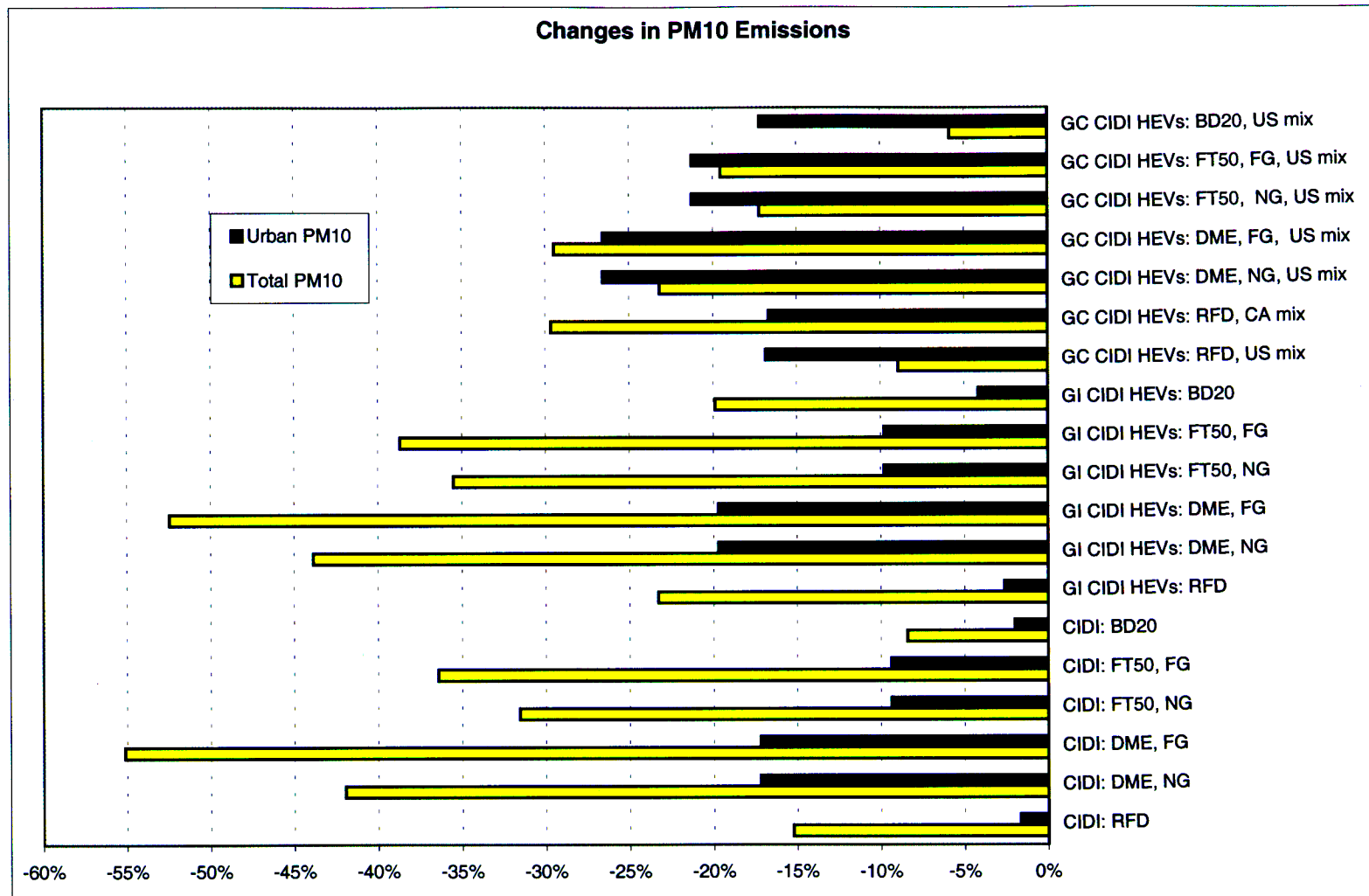
Figure C-2.67 Changes in Fuel-Cycle PM 10 Emissions Relative to GV's Fueled with RFG, Light-Duty Trucks 2: Long-Term CIDI Vehicles and CIDI Hybrid Electric Vehicles
