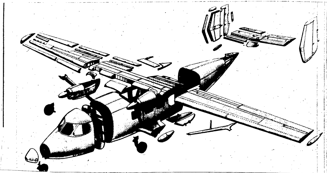
TECHNOLOGICAL BREAKDOWN OF THE AN-28 AIRCRAFT
