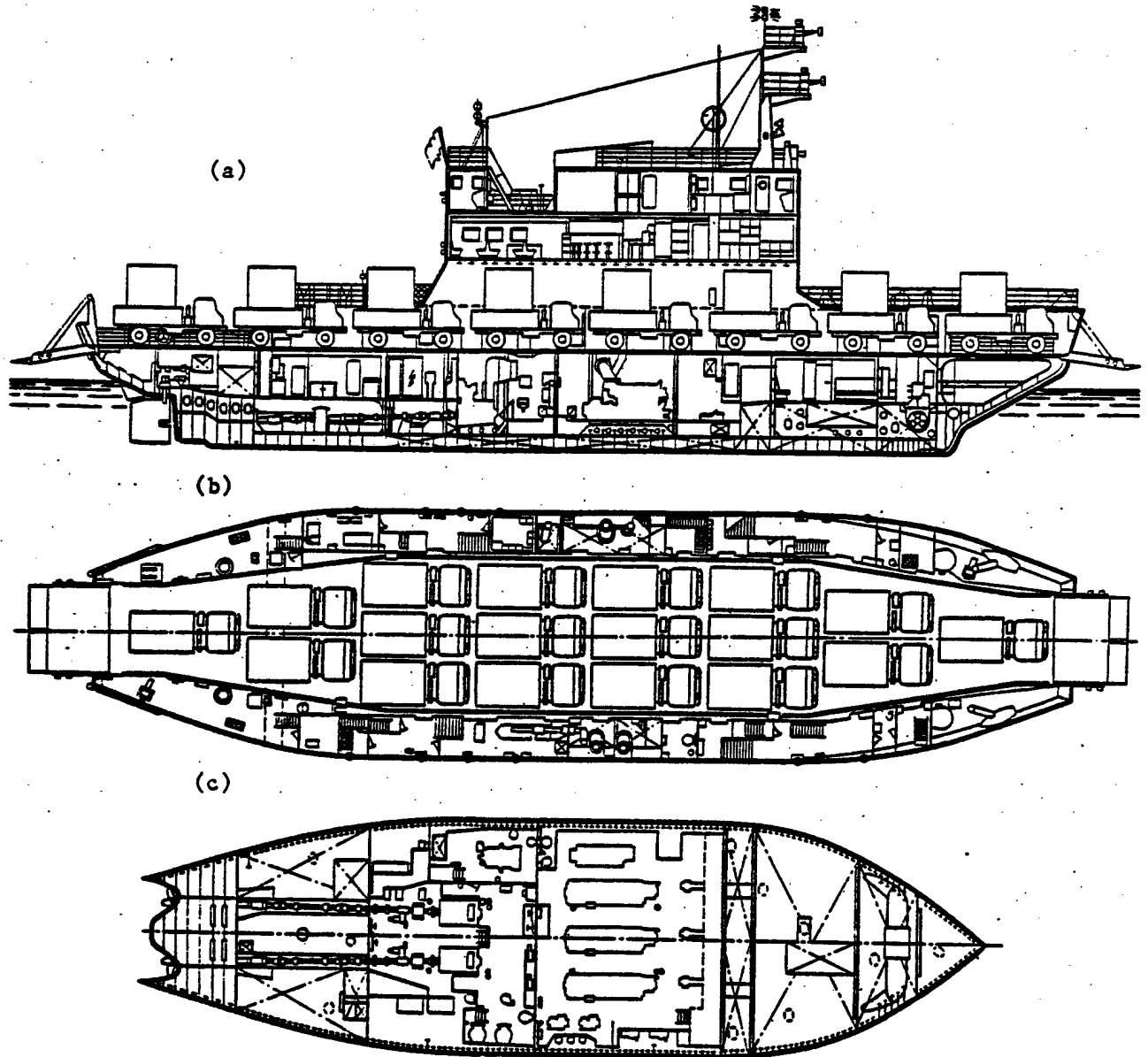
GENERAL LAYOUT OF THE VESSEL a. Side view b. Upper deck c. hold
