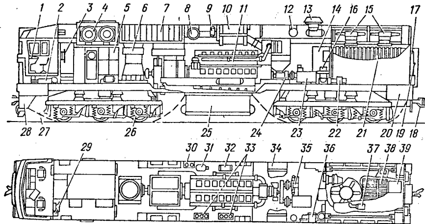
Arrangement of principal equipment on a section of the 4TE130 diesel-electric locomotive.
