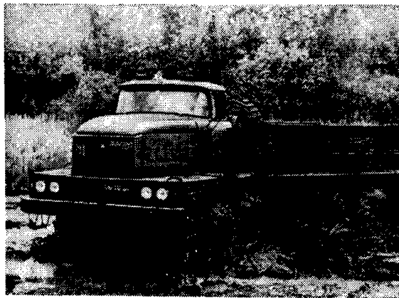
Figure 2. Articulated truck on arch tires making its way through a boggy section.
