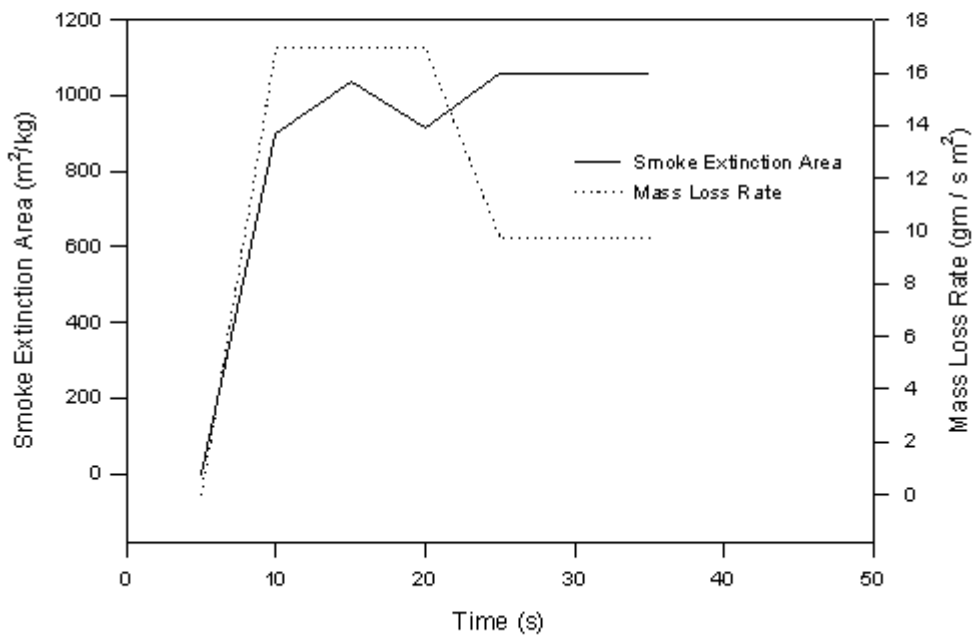
Figure D-5. Sample 1d. Seat Cushion, PVC Cover Only
