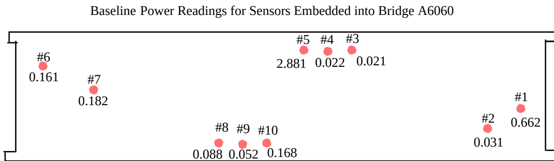
Figure 19.b. Baseline power readings for sensors within bridge A6060.
