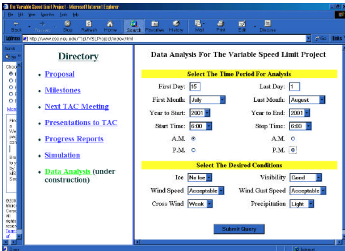
Figure 8. Selecting the Atmospheric and Road Surface Conditions for Analysis
