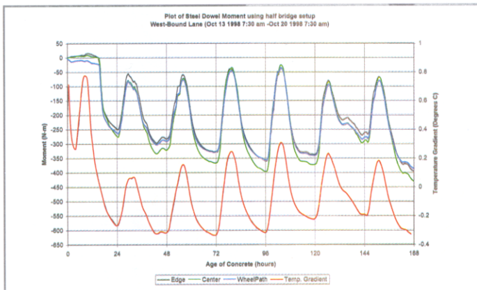
Figure 4—Typical Steel Dowel Environmental Moment Data
