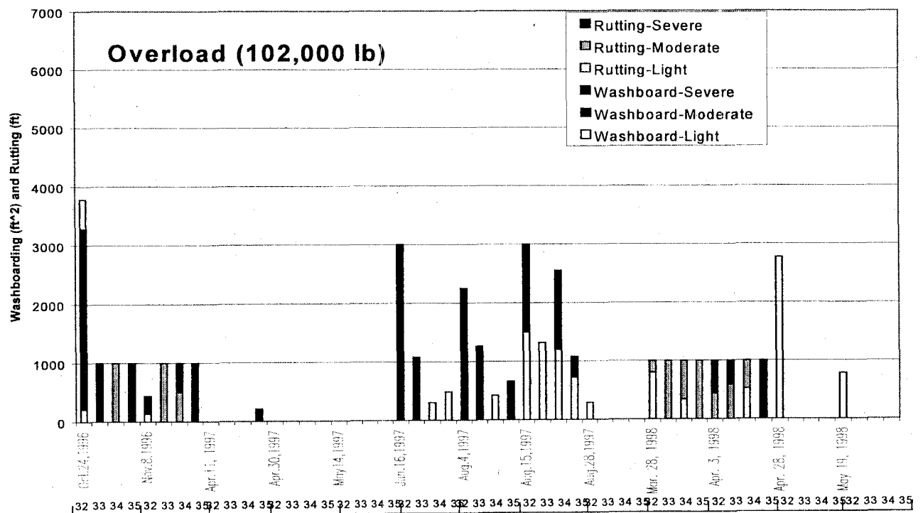
Figure 5. 102,000 lb Lane Distress Rating
