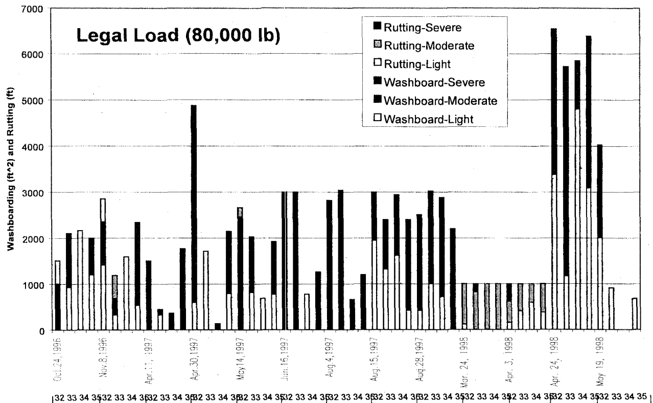
Figure 4. 80,000 lb Lane Distress Rating
