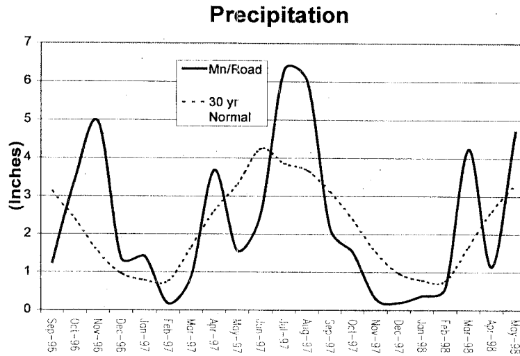
Figure 2. Precipitation at Mn/ROAD
