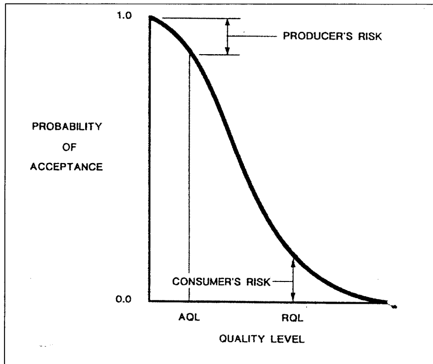
Figure 3.2: Conventional OC curve (after Weed 1995 )
