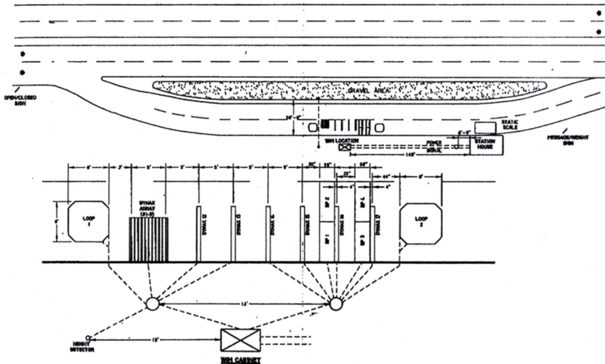
Figure 5.1: Configuration of Wyeth WIM system
