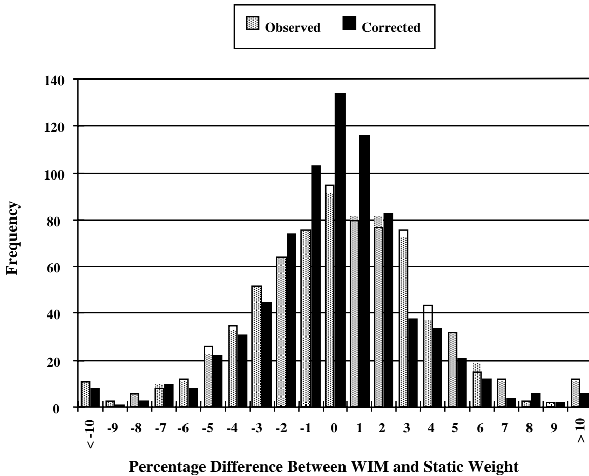
Figure 7.1: Frequency distribution of error for observed and regression-corrected axle weight data
