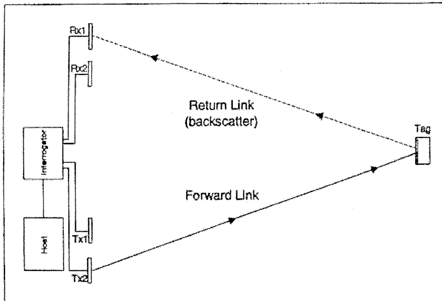
Figure 2.1: MicroStamp 4000 System (courtesy of Micron Communications, Inc.)
