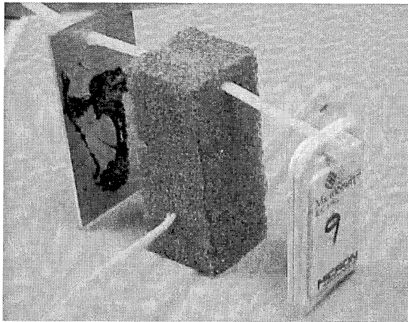
Figure 2.3: Modified Tags. The MicroStamp 10ML tag is right, styrofoam spacer center and back plane left.
