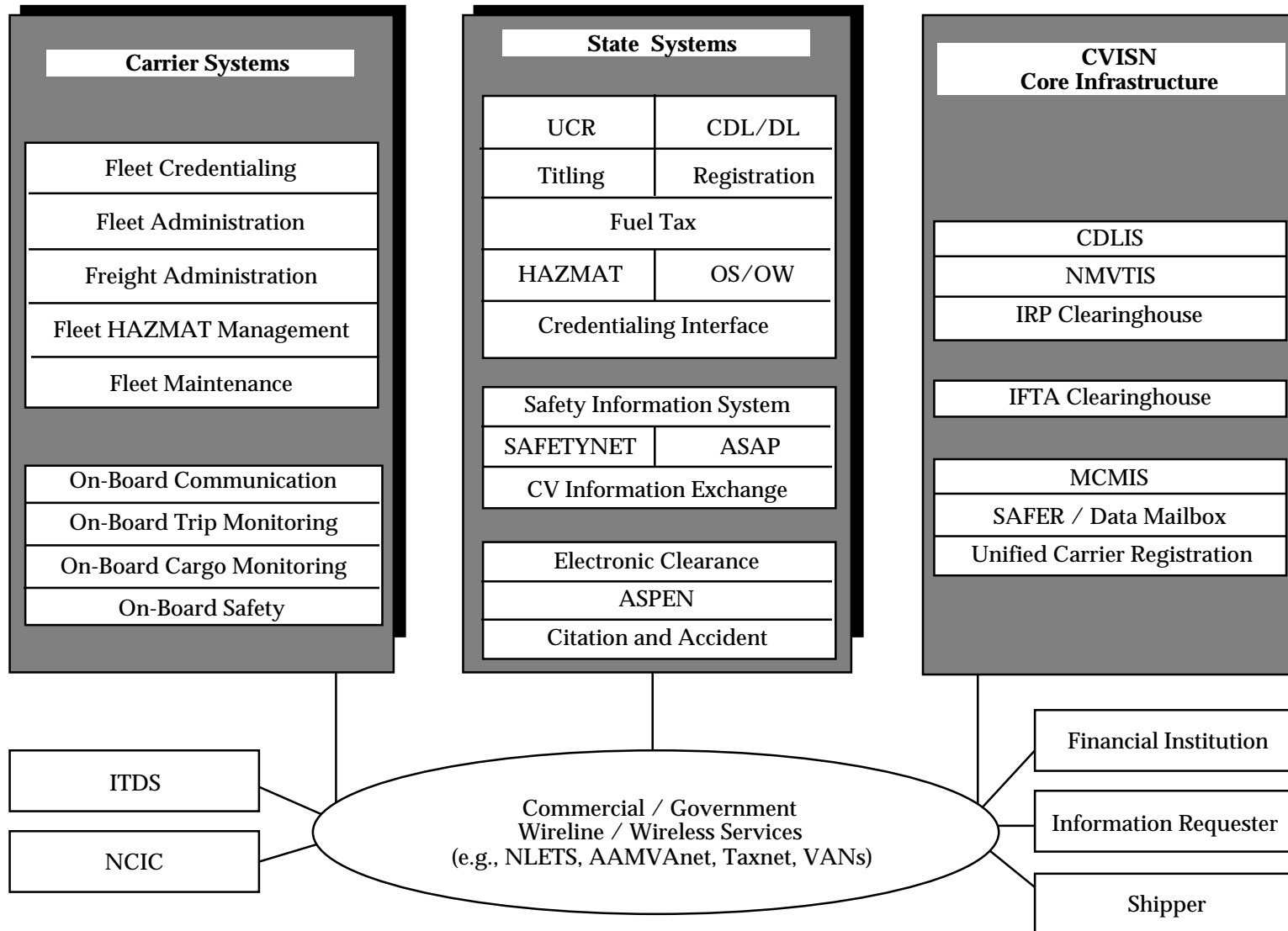
Figure 1.3 CVISN System Design
