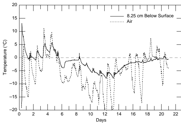
Figure B3. Slab.
