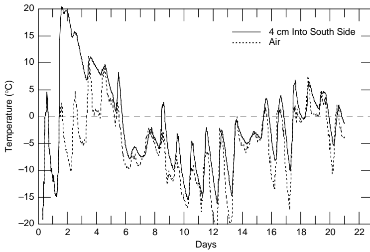
Figure B7. Wall.
